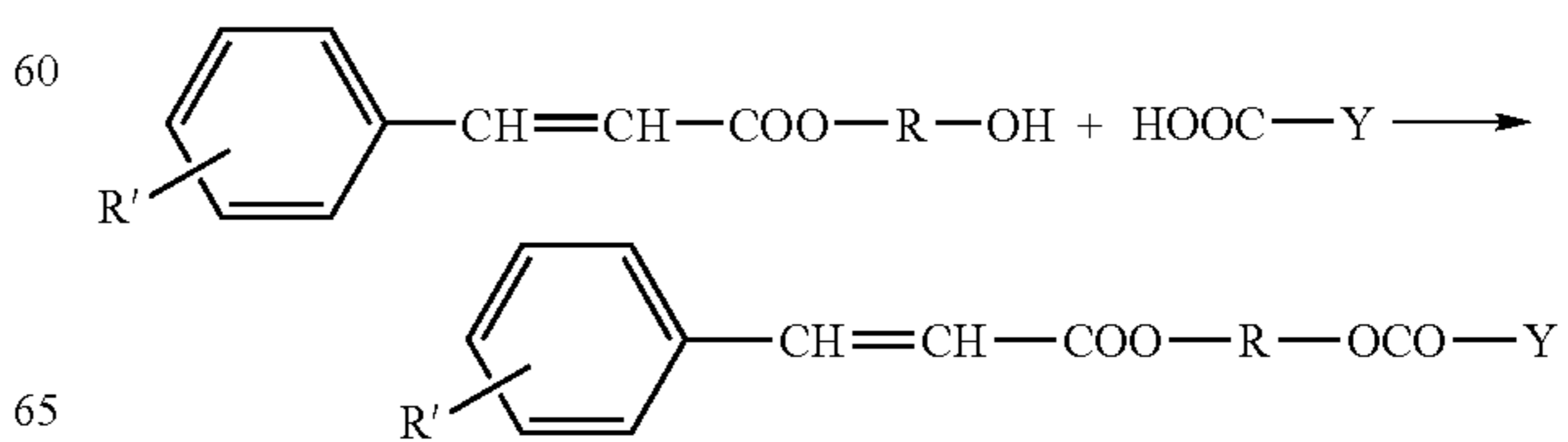
Reaction scheme (4)
