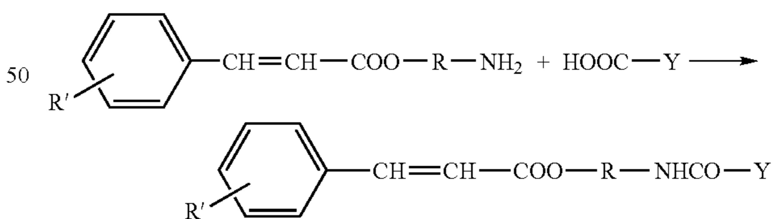
Reaction scheme (3)
