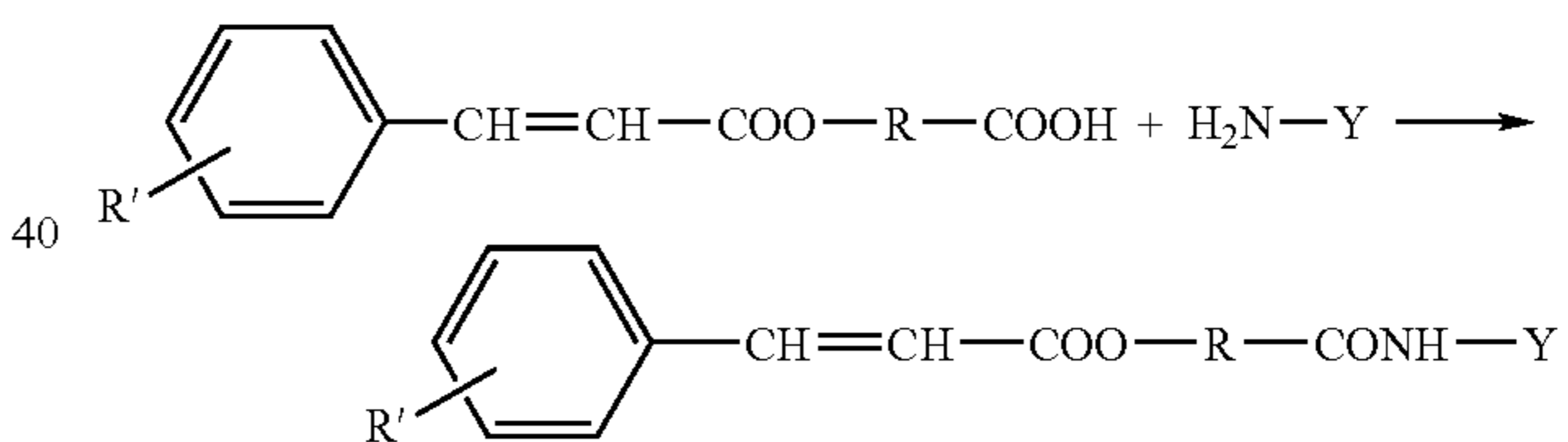
Reaction scheme (2)
