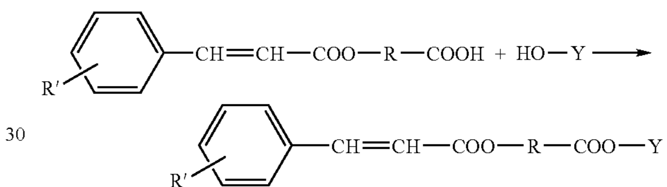
Reaction scheme (1)
