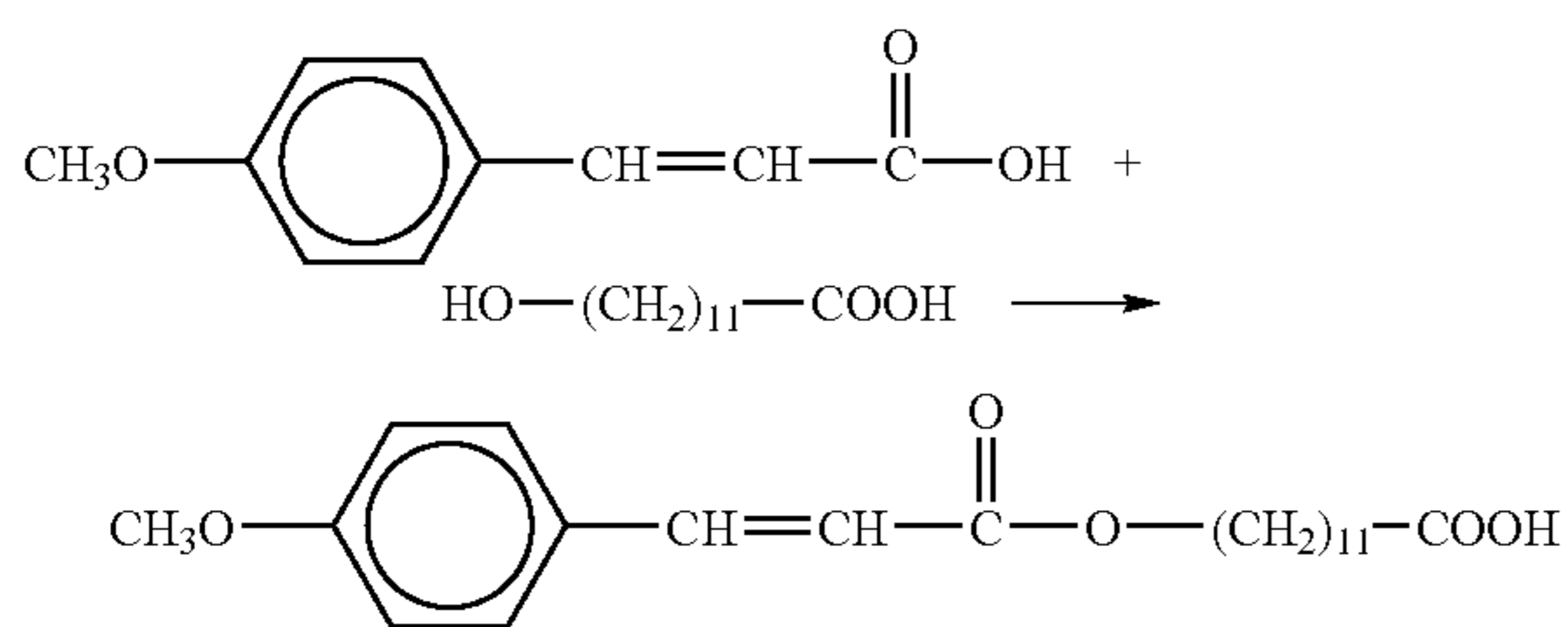
Reaction scheme (8)
