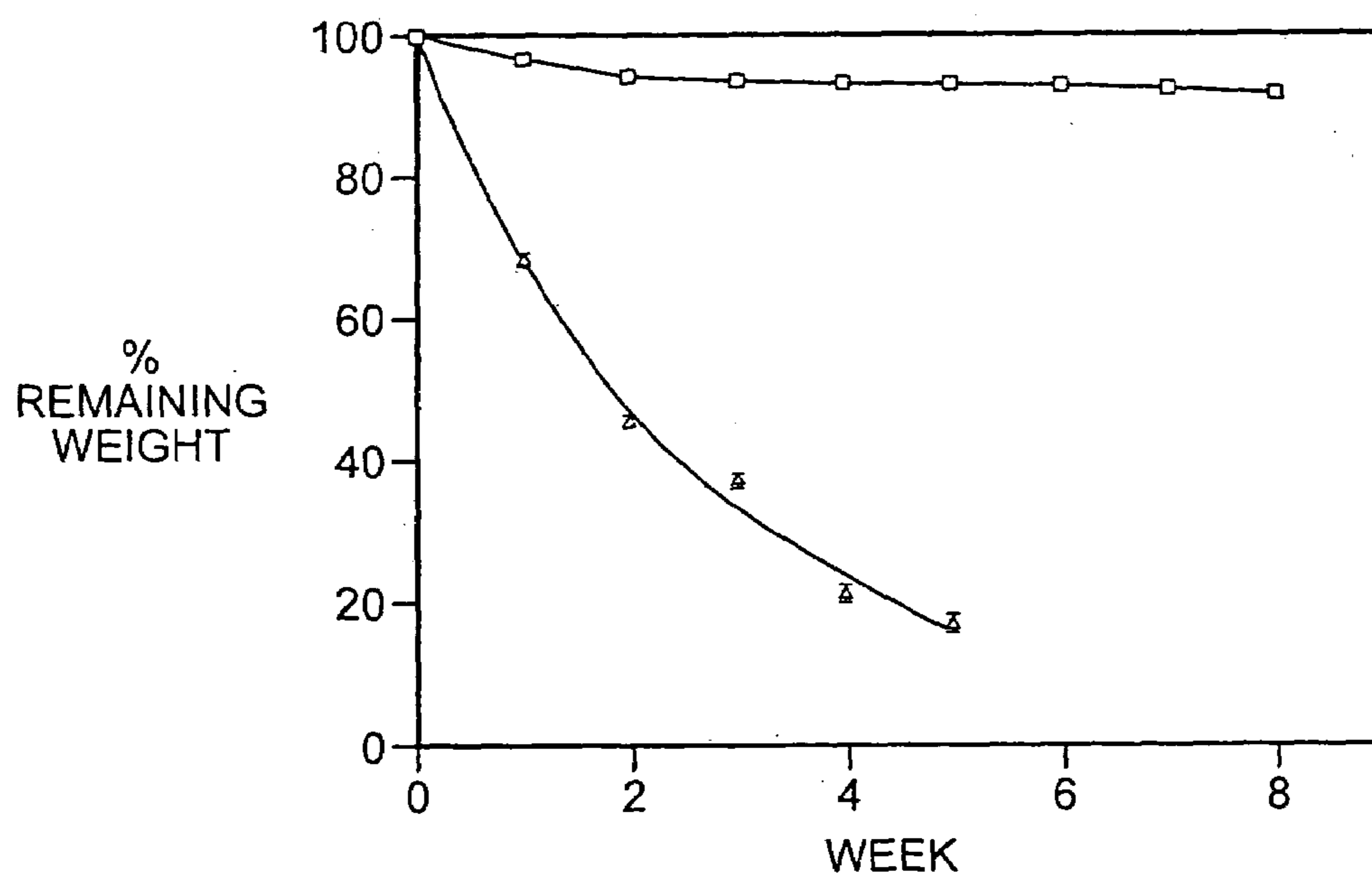
FIG. 10 BIODEGRADATION RATE OF ELECTROSPUN MEMBRANE
