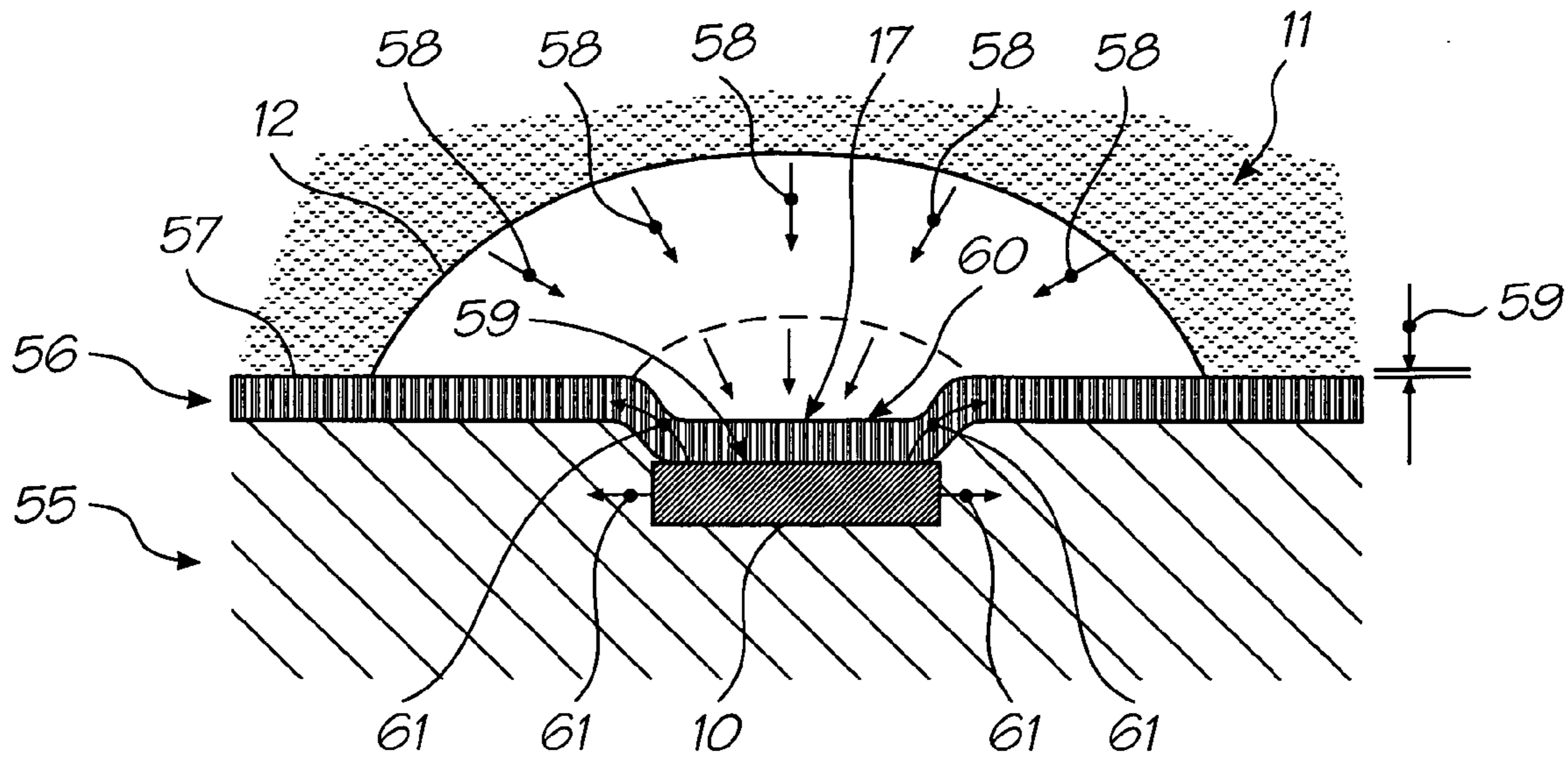
FIG. 47 (PRIOR ART)
