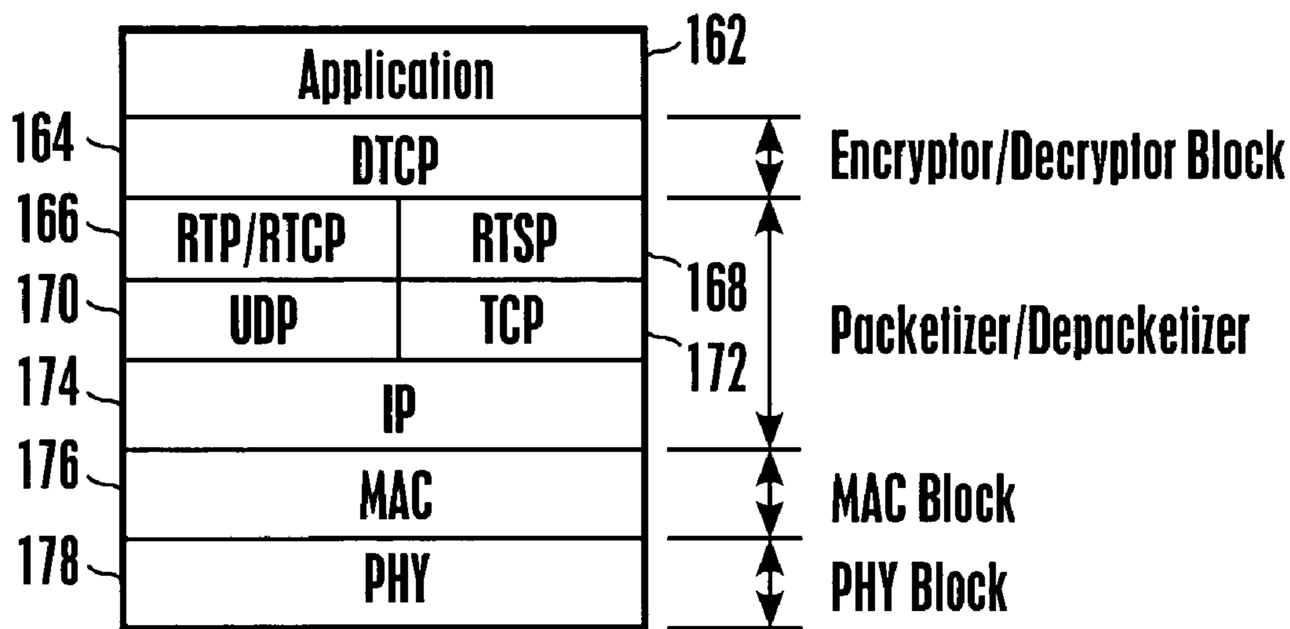
Figure 6 Protocol Stack
