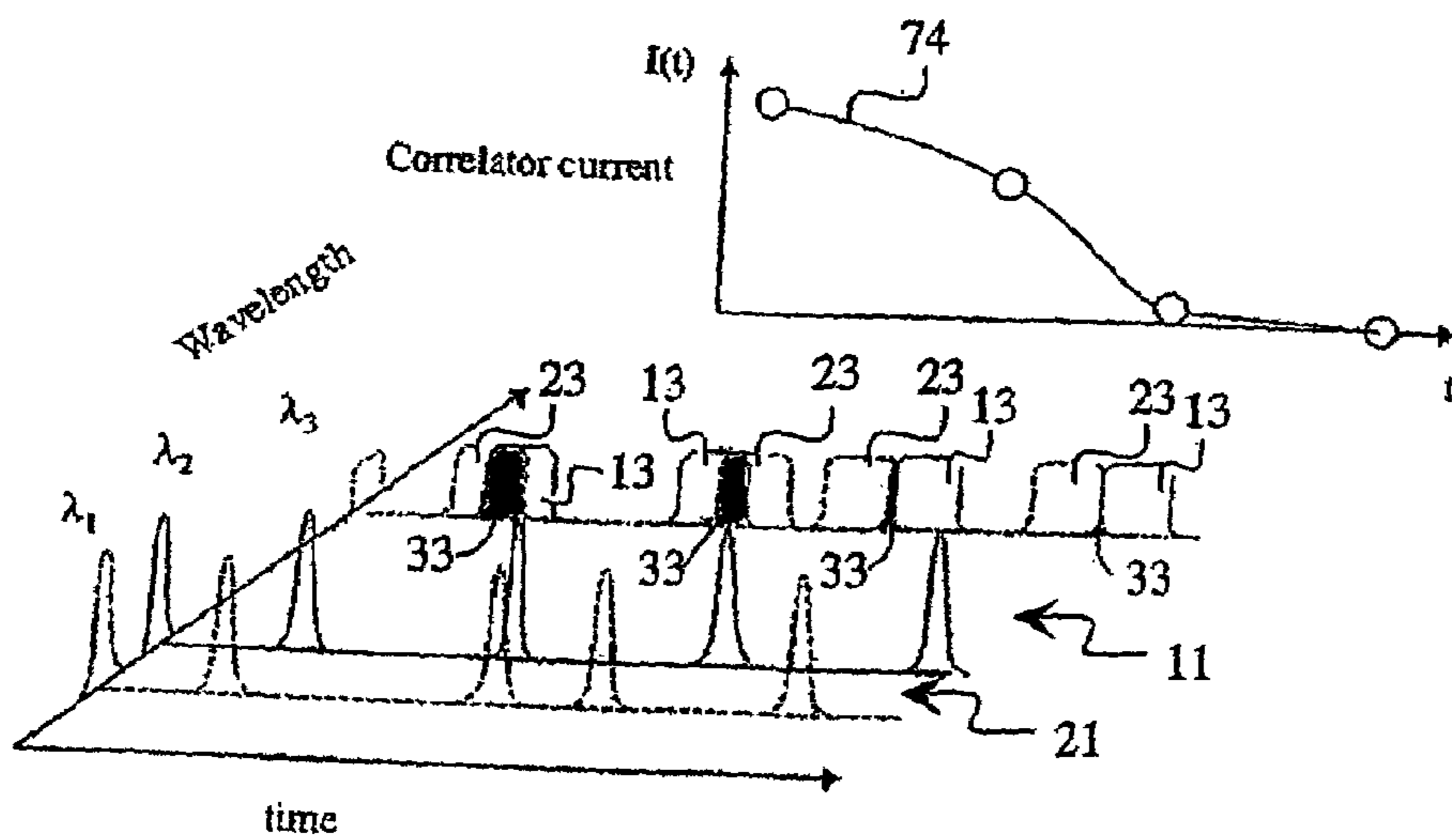
FIG. 5 (Prior Art)
