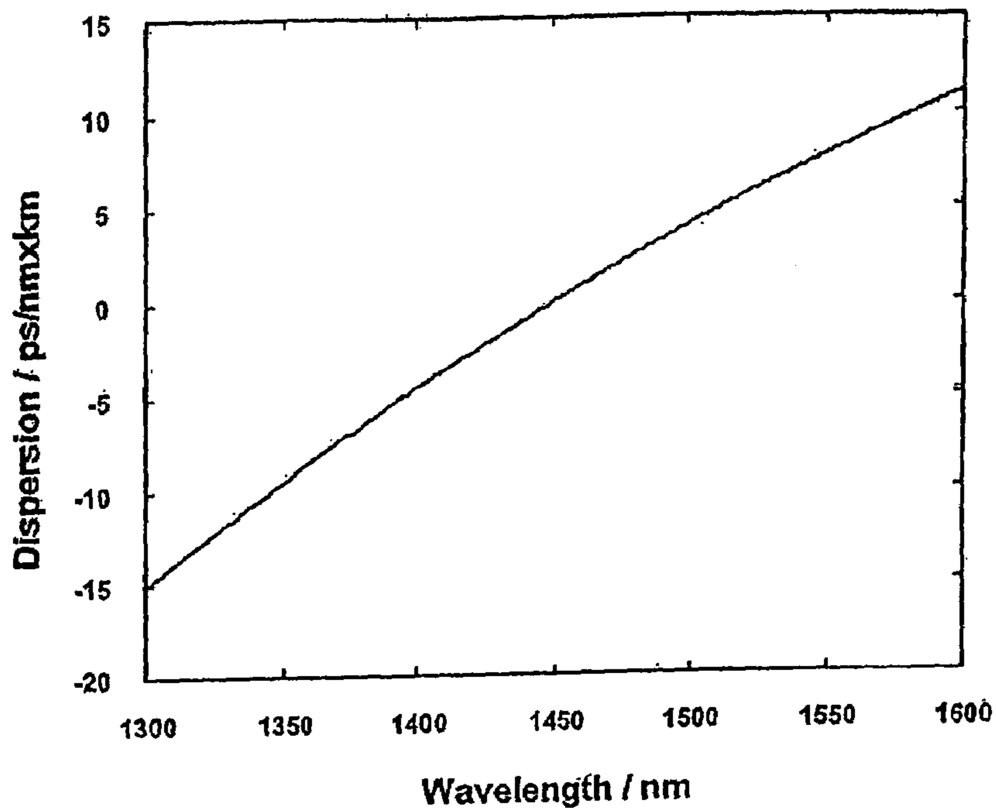
FIG. 10 (Prior Art)
