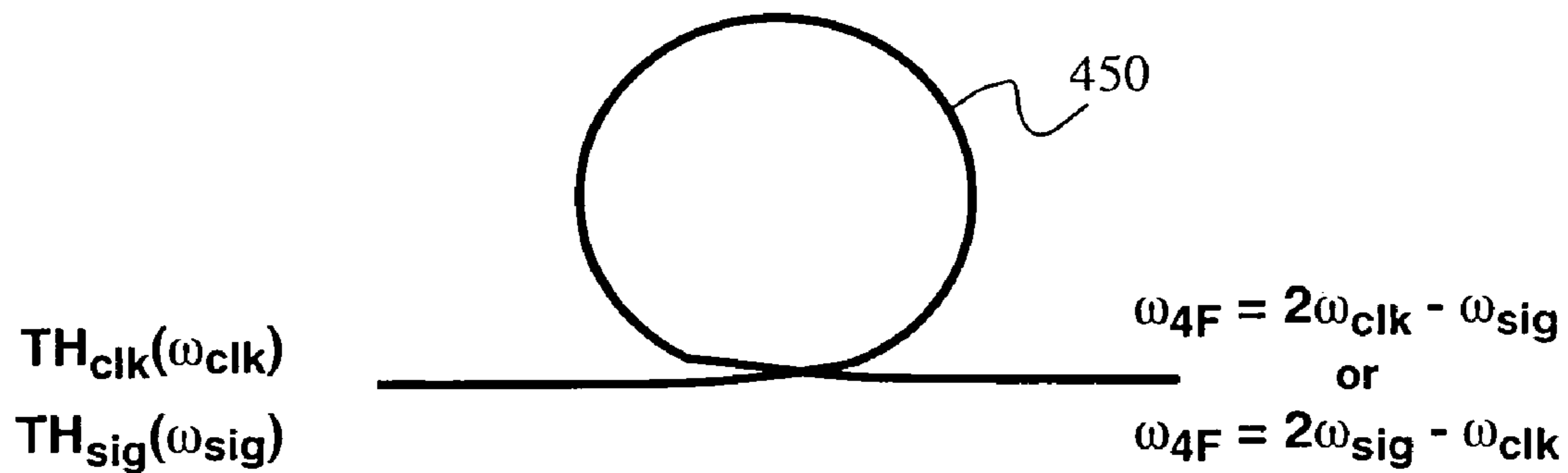
FIG. 4C (Prior Art)
