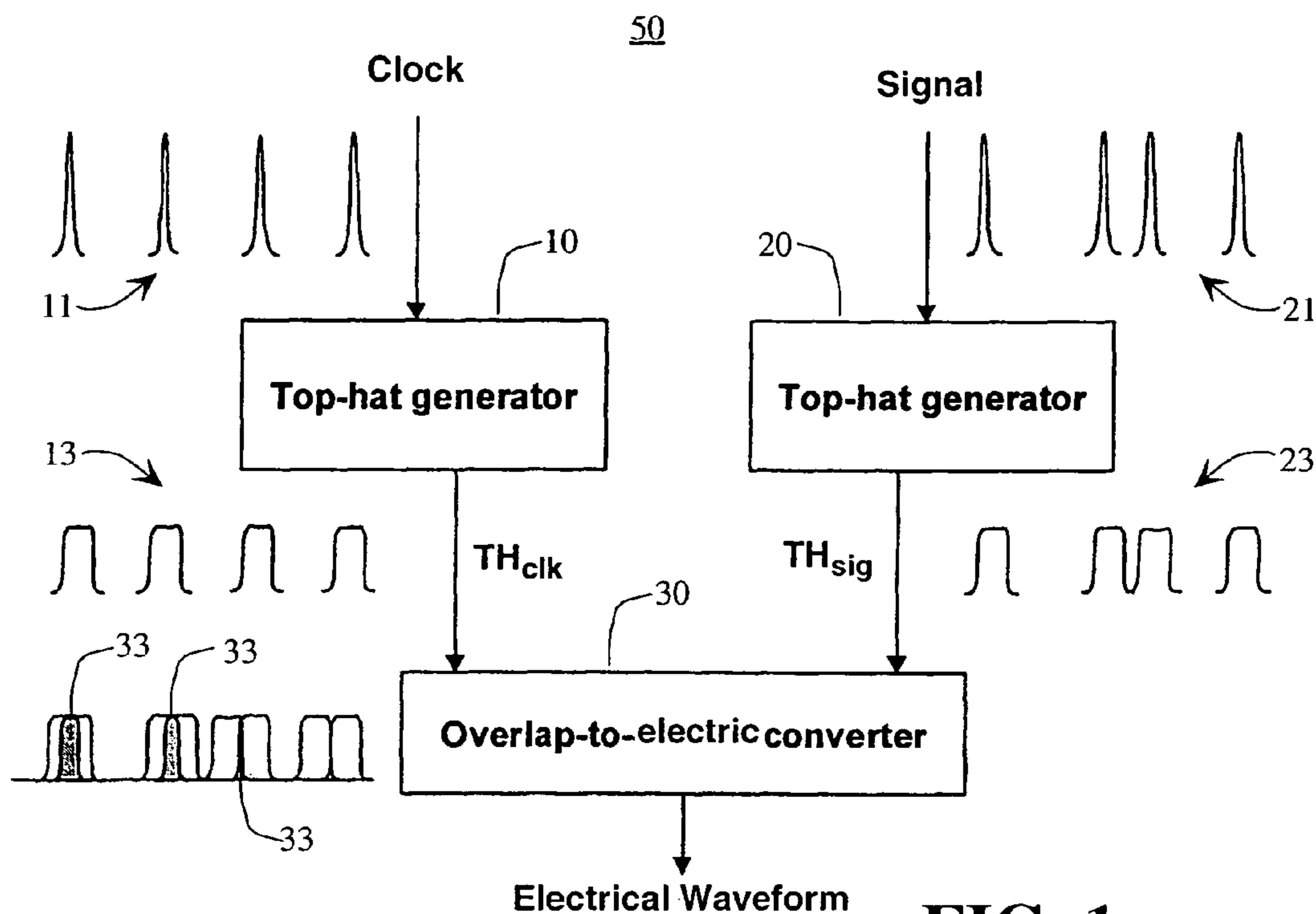
FIG. 1 (Prior Art)
