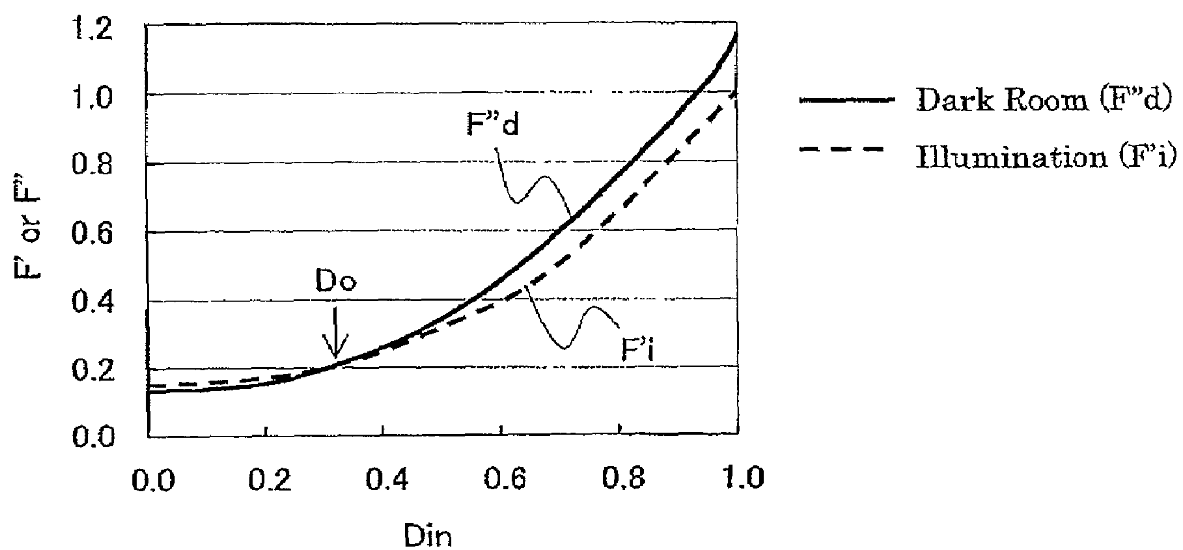
Overlapping \gamma Curves at a Reference Point D_o
