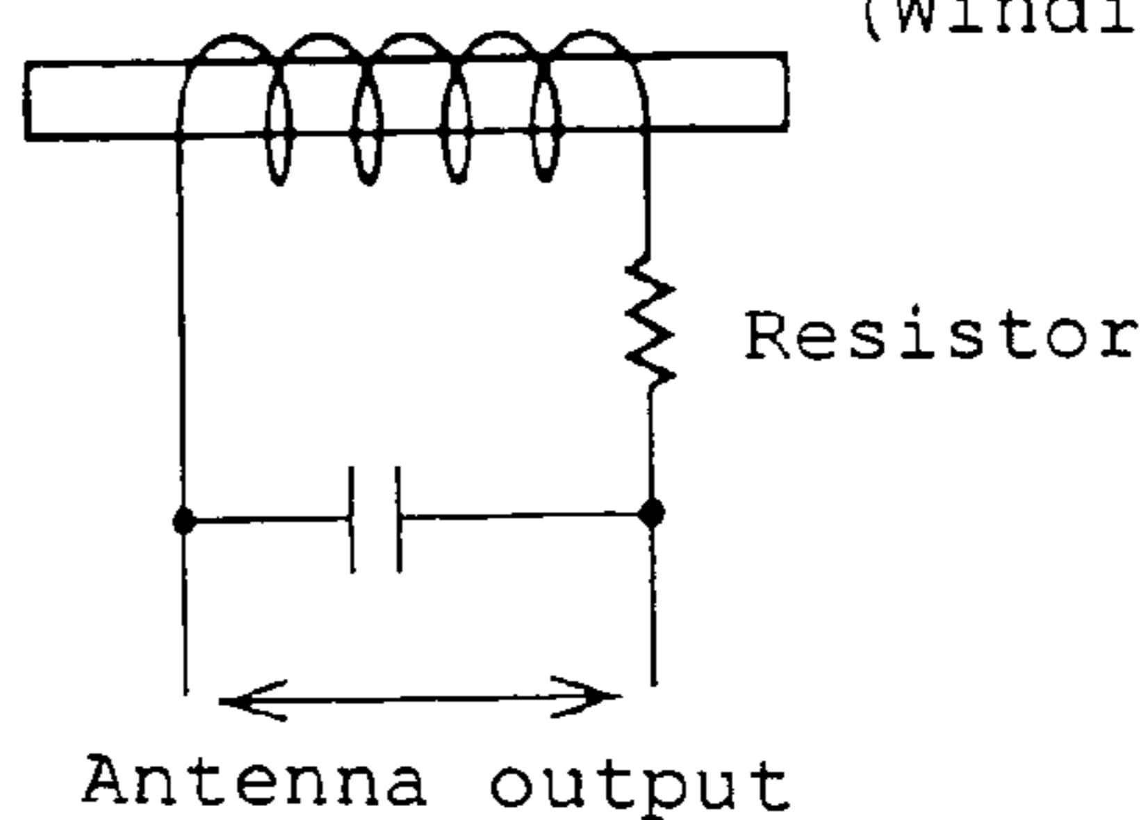
(B) Number of turns: 500 T
