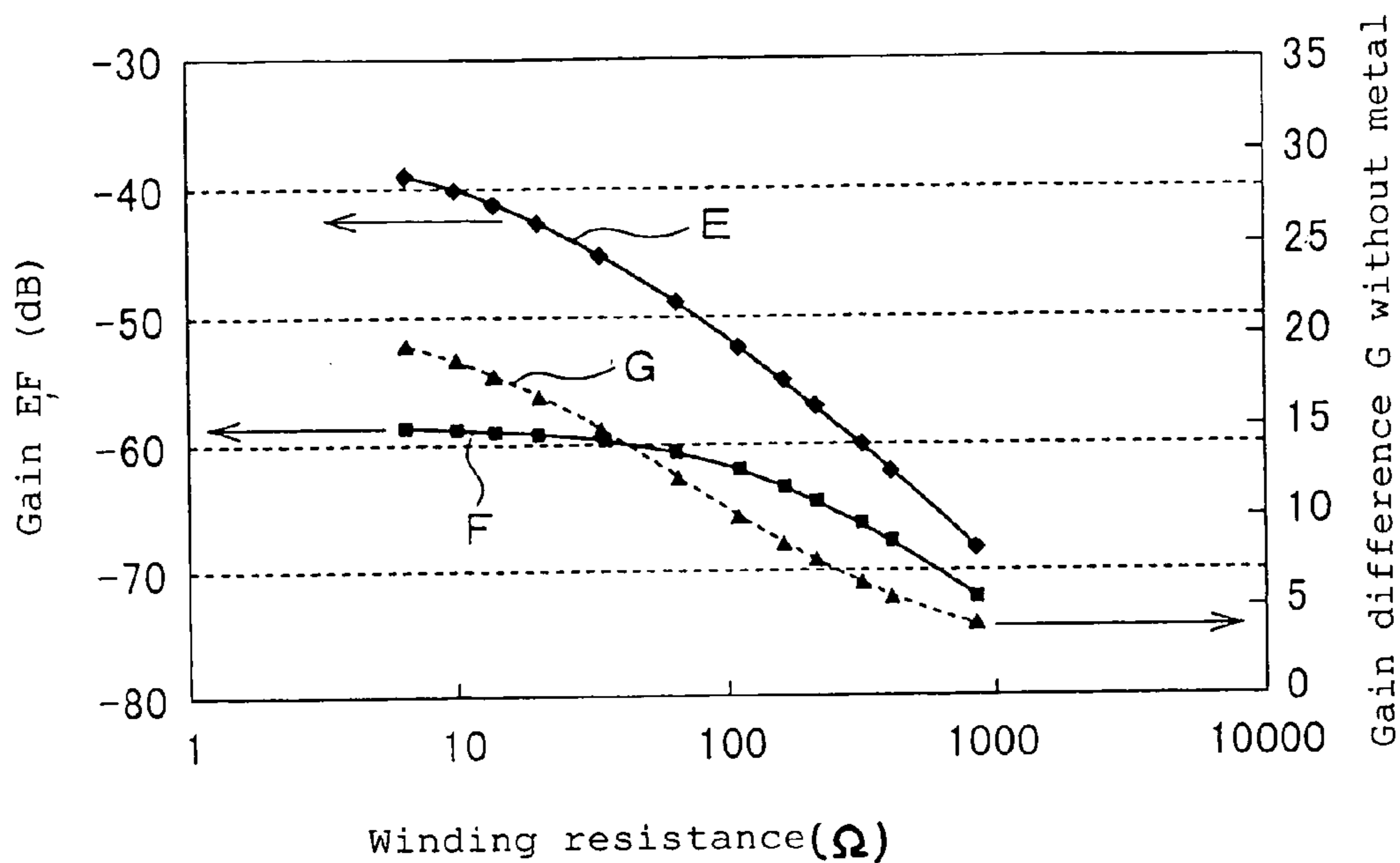
(A) Antenna Gain-Winding Resistance
