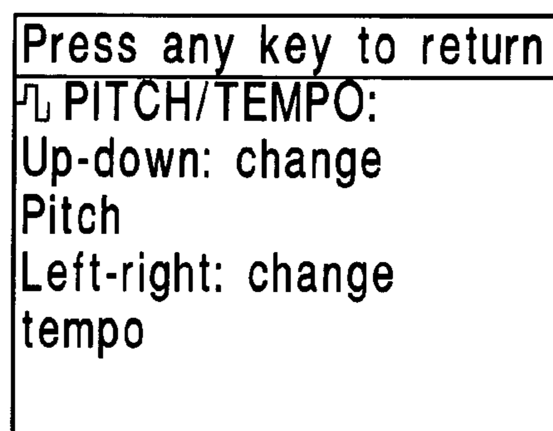
Help Screen
