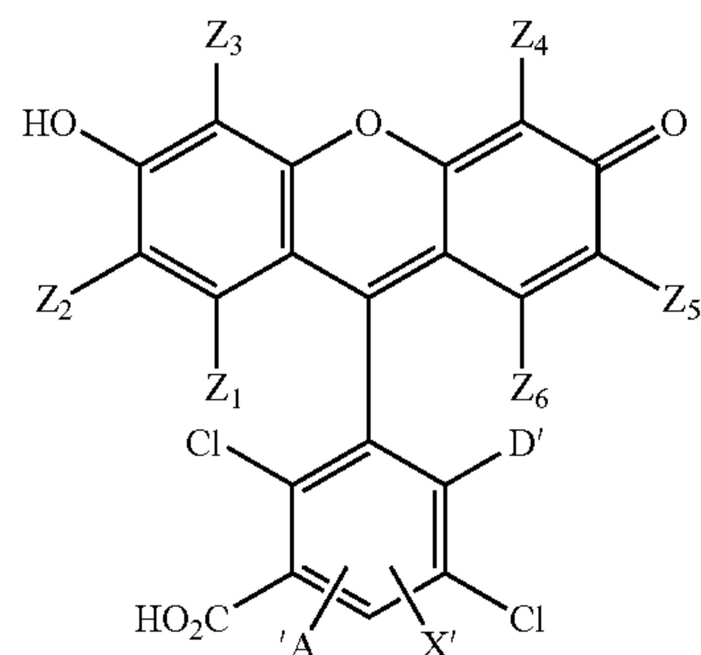
4,7 Dichlorofluorescein (See U.S. Pat. No. 5,188,934)
