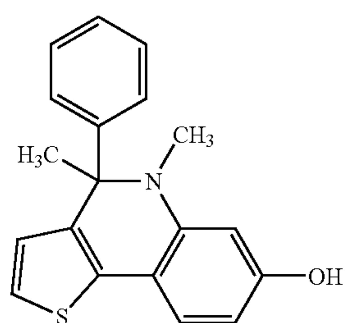
Compound 22
