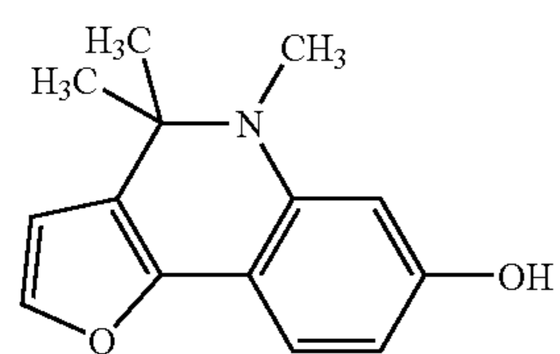
Compound 11
