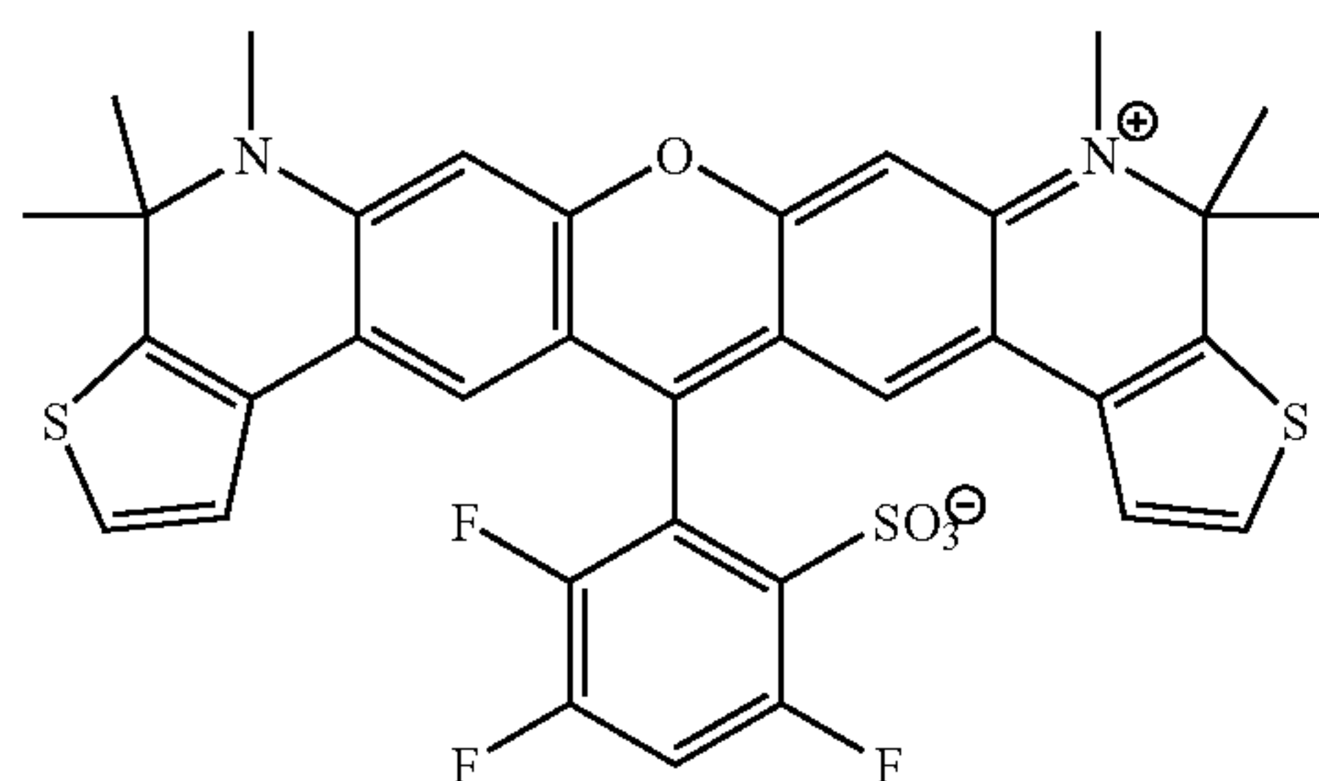
Compound 62
