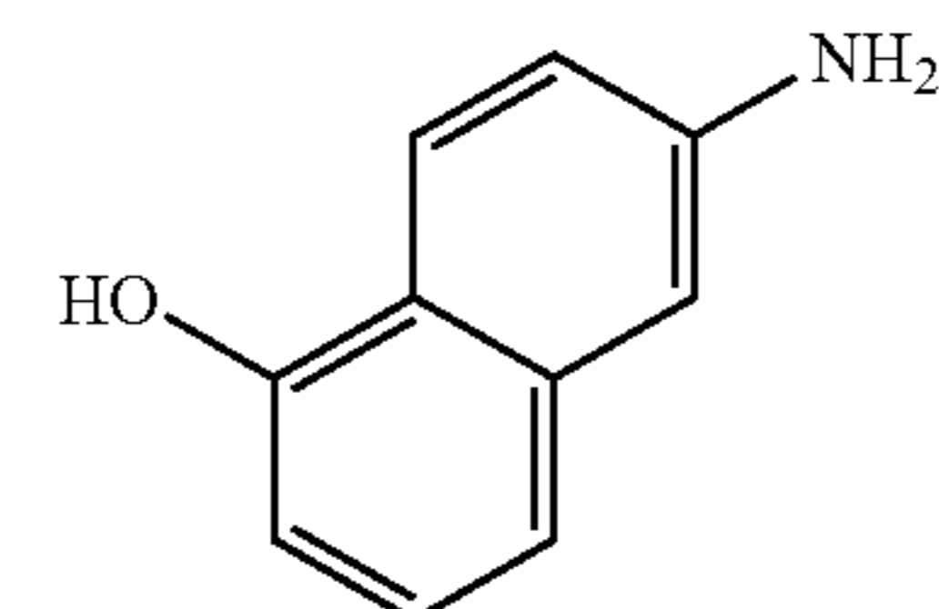
a 6-amino-1-naphthol
