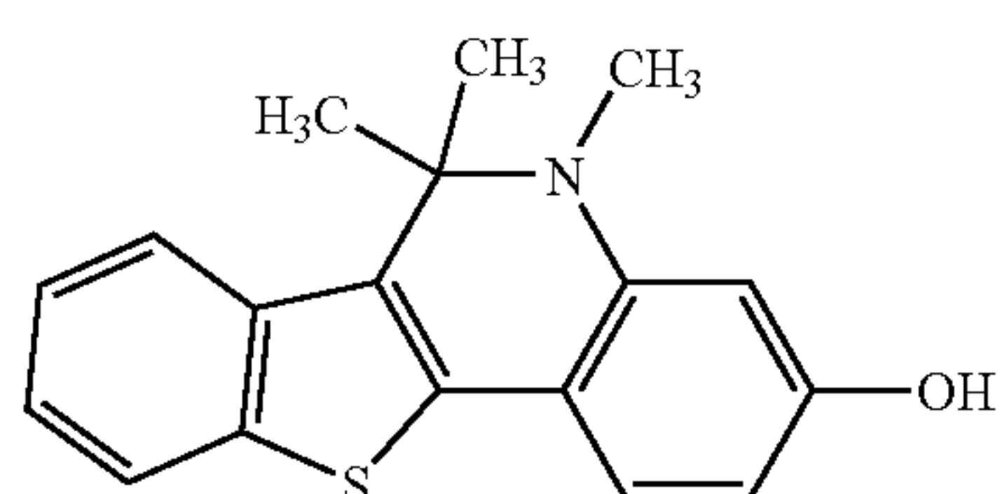
Compound 10
