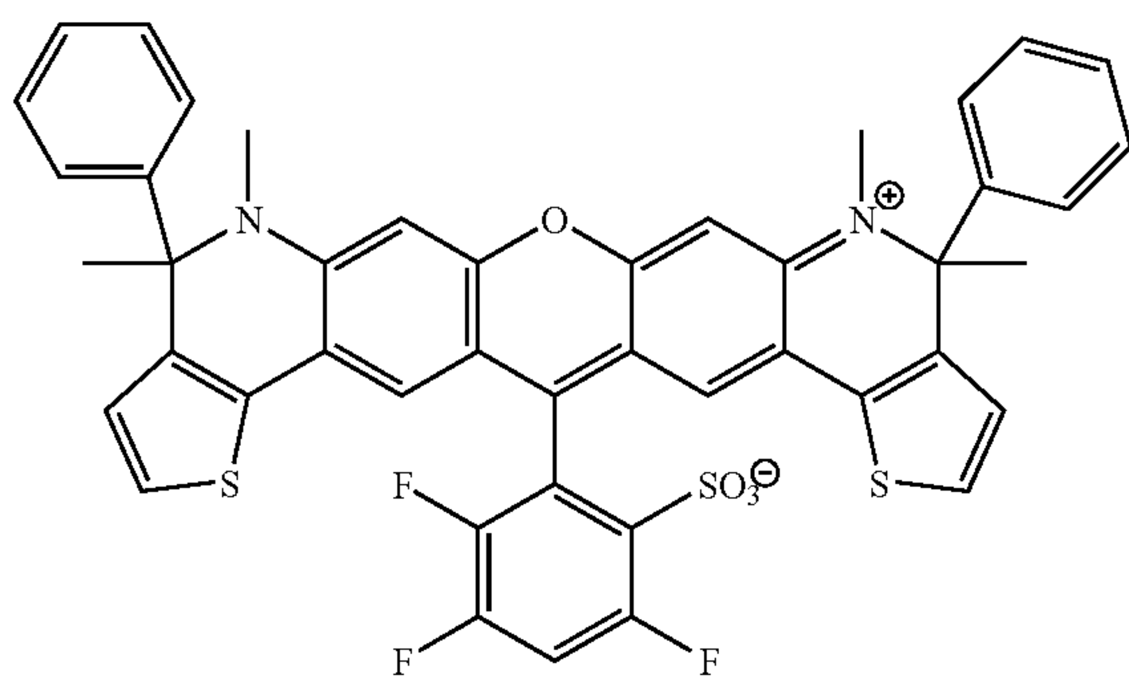
Compound 32
