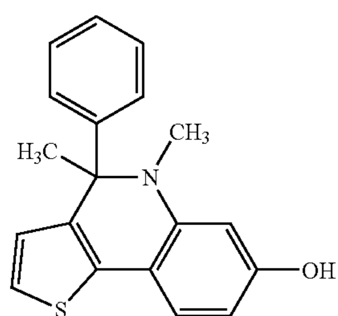
Compound 22
