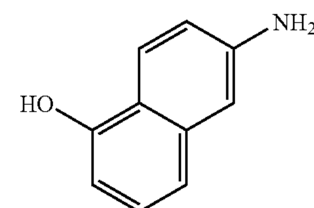
a 6-amino-1-naphthol
