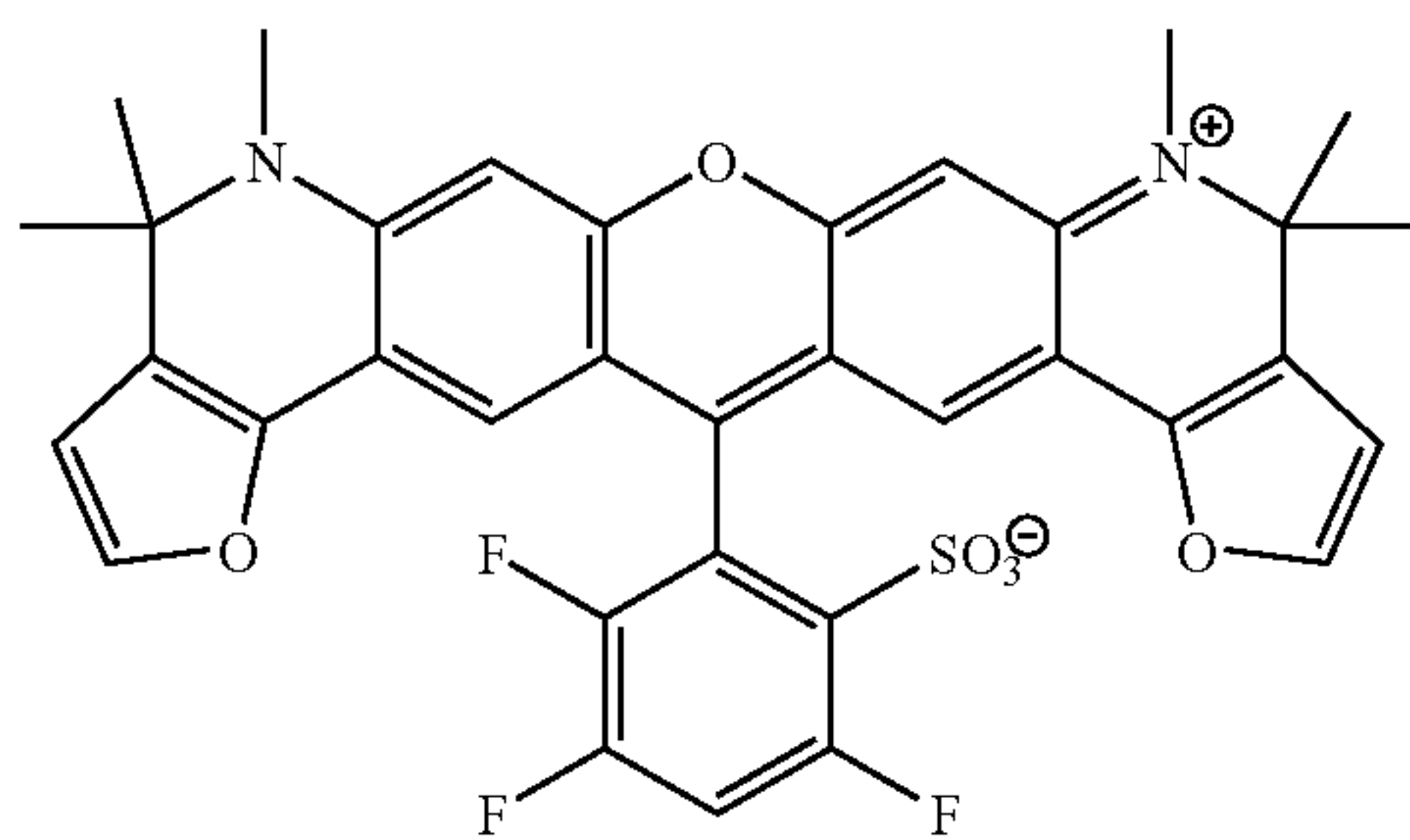
Compound 35
