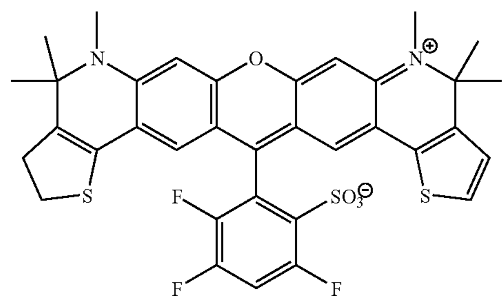
Compound 23
