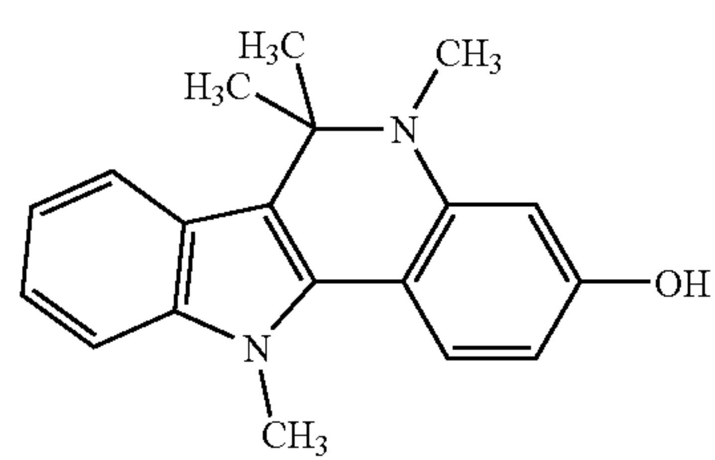
Compound 12
