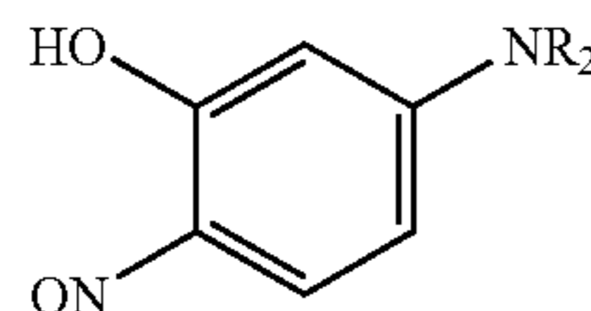
a 6-nitroso-3-aminophenol
