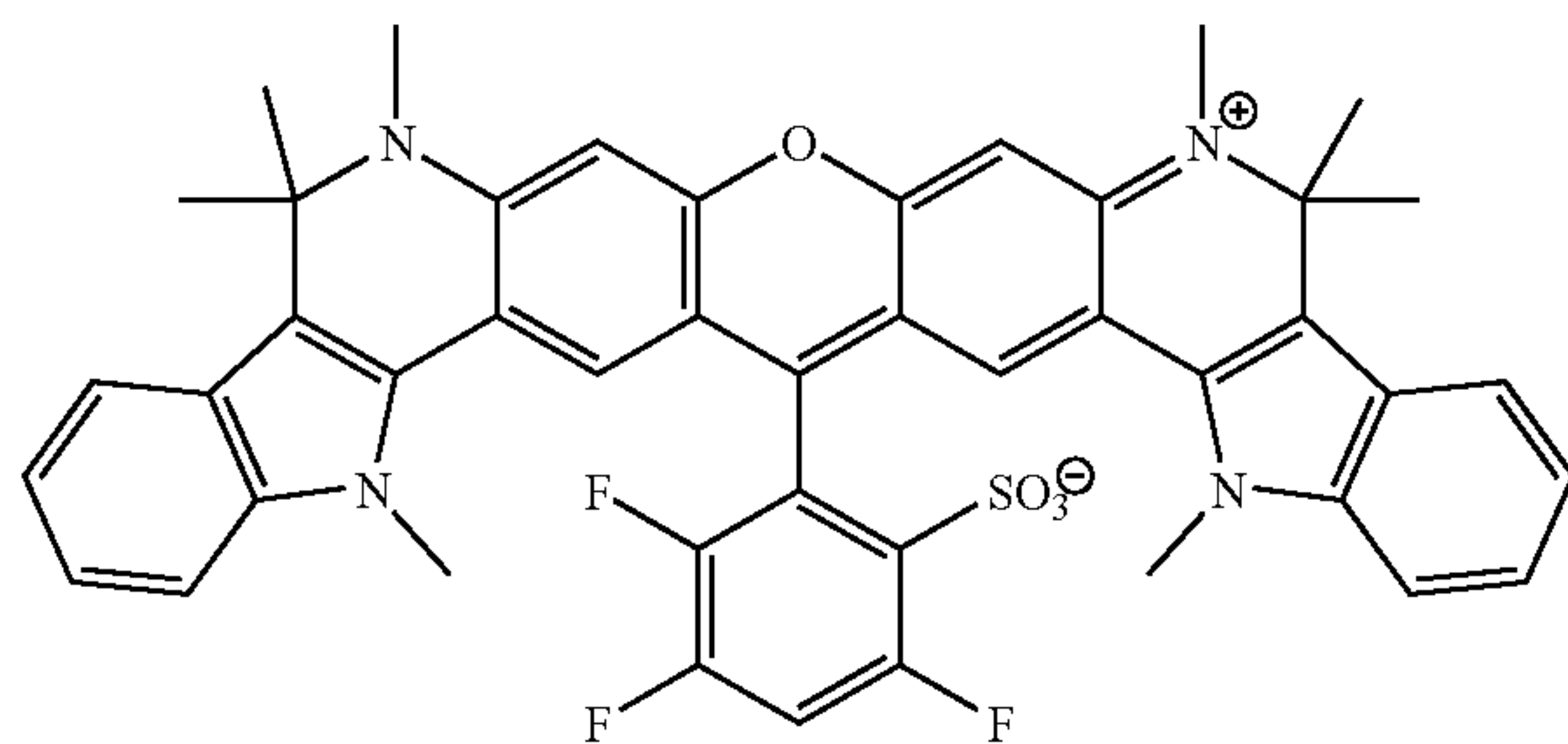
Compound 36
