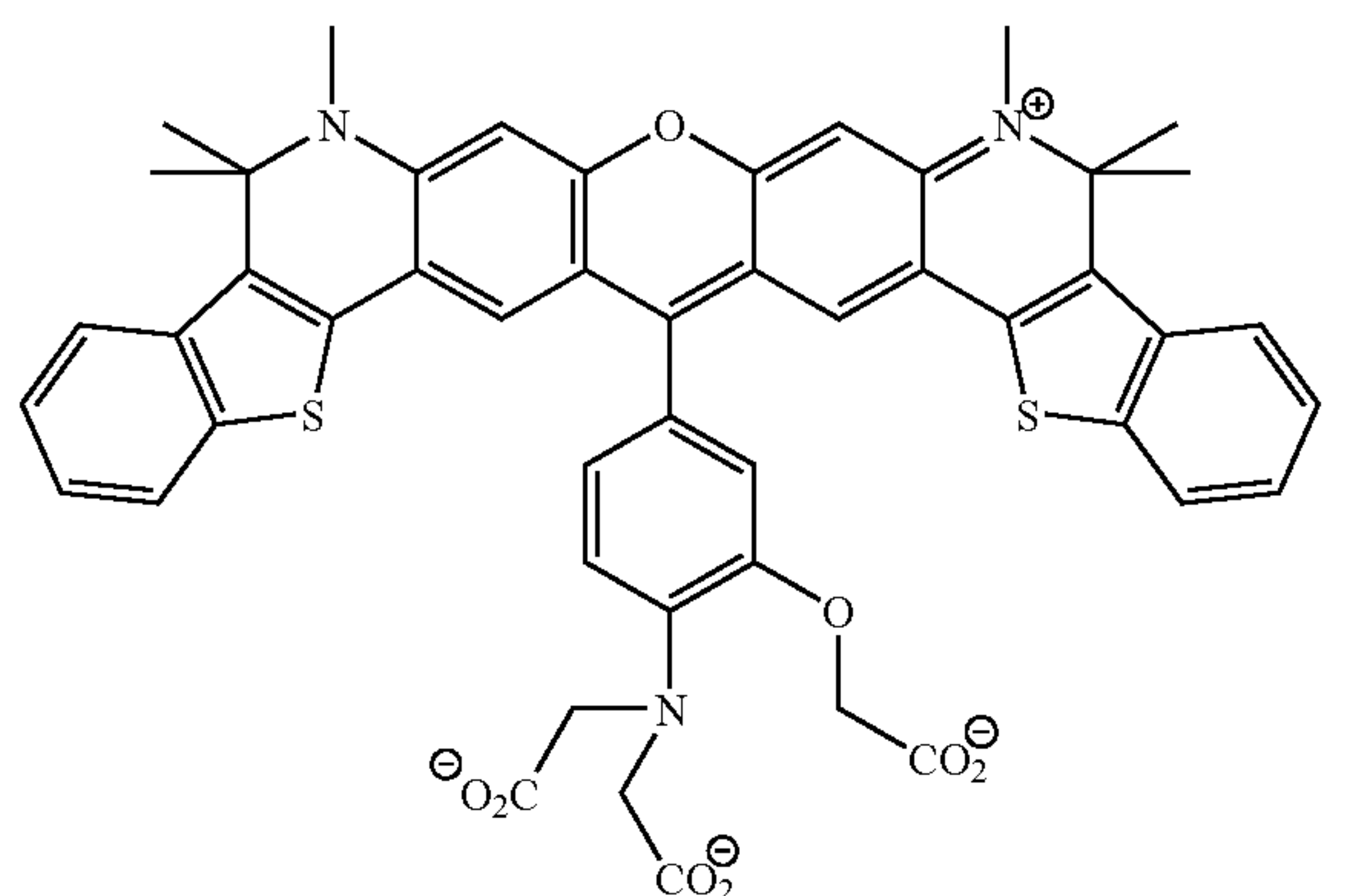
Compound 59
