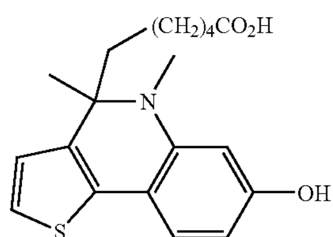
Compound 20
