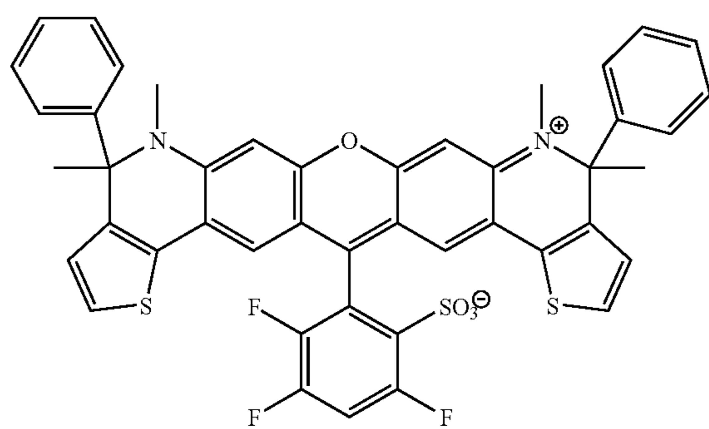
Compound 32
