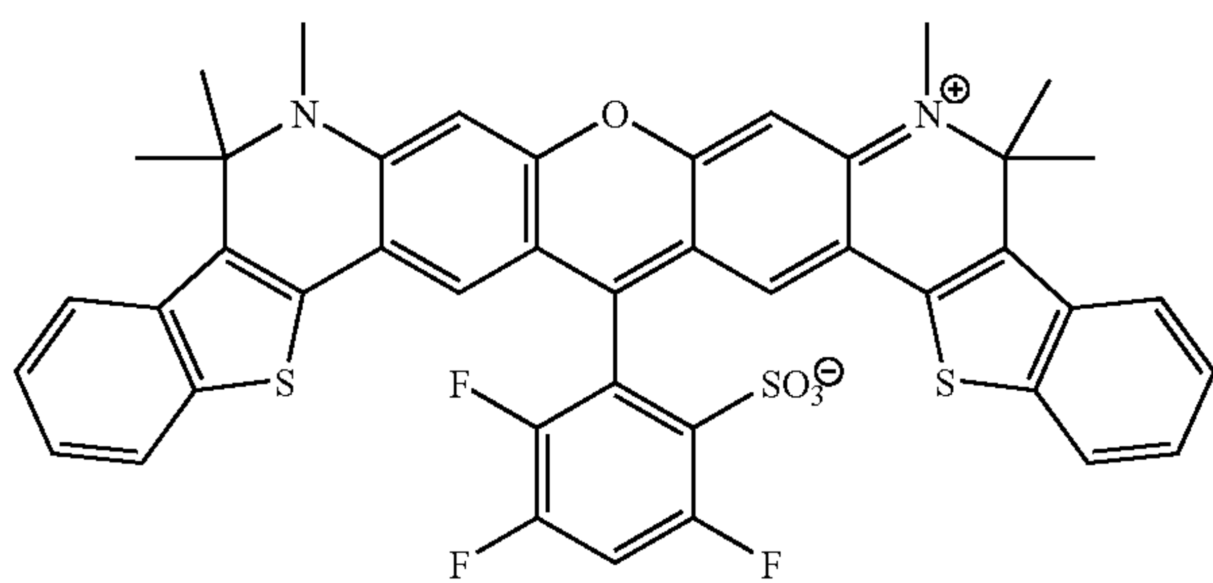
Compound 24
