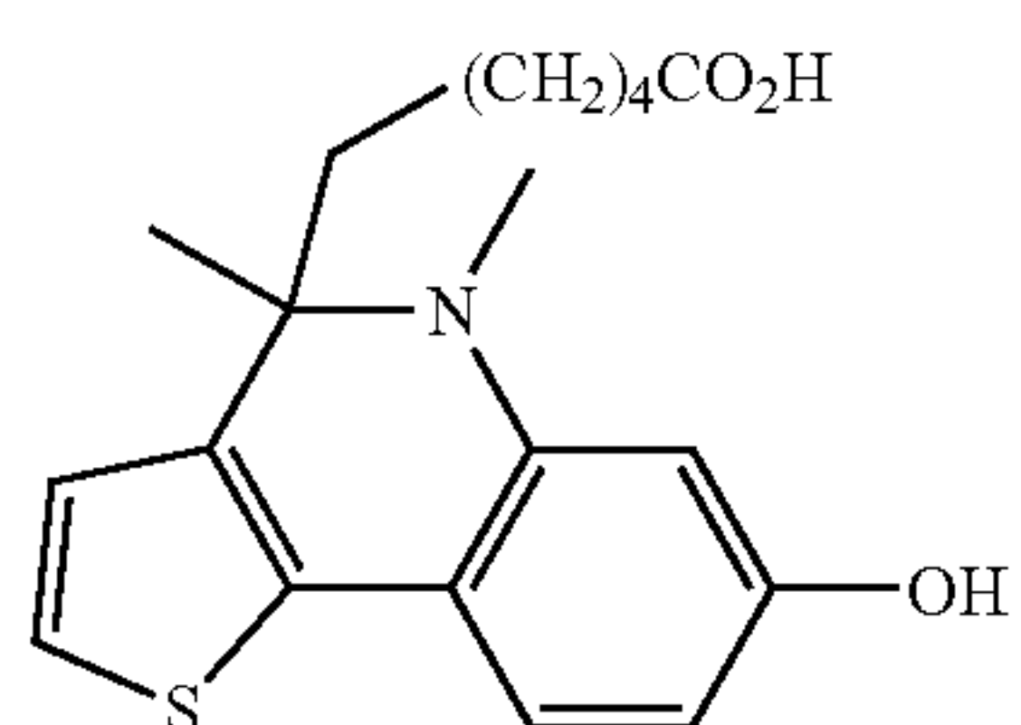
Compound 20
