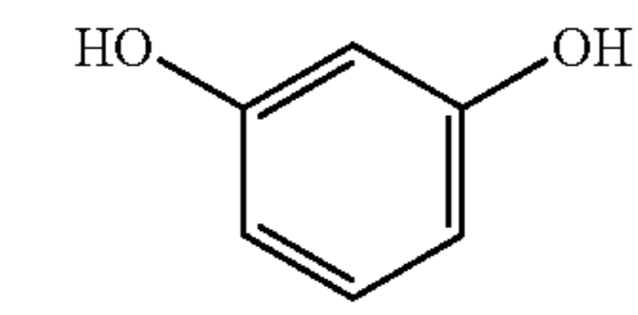
a resorcinol
