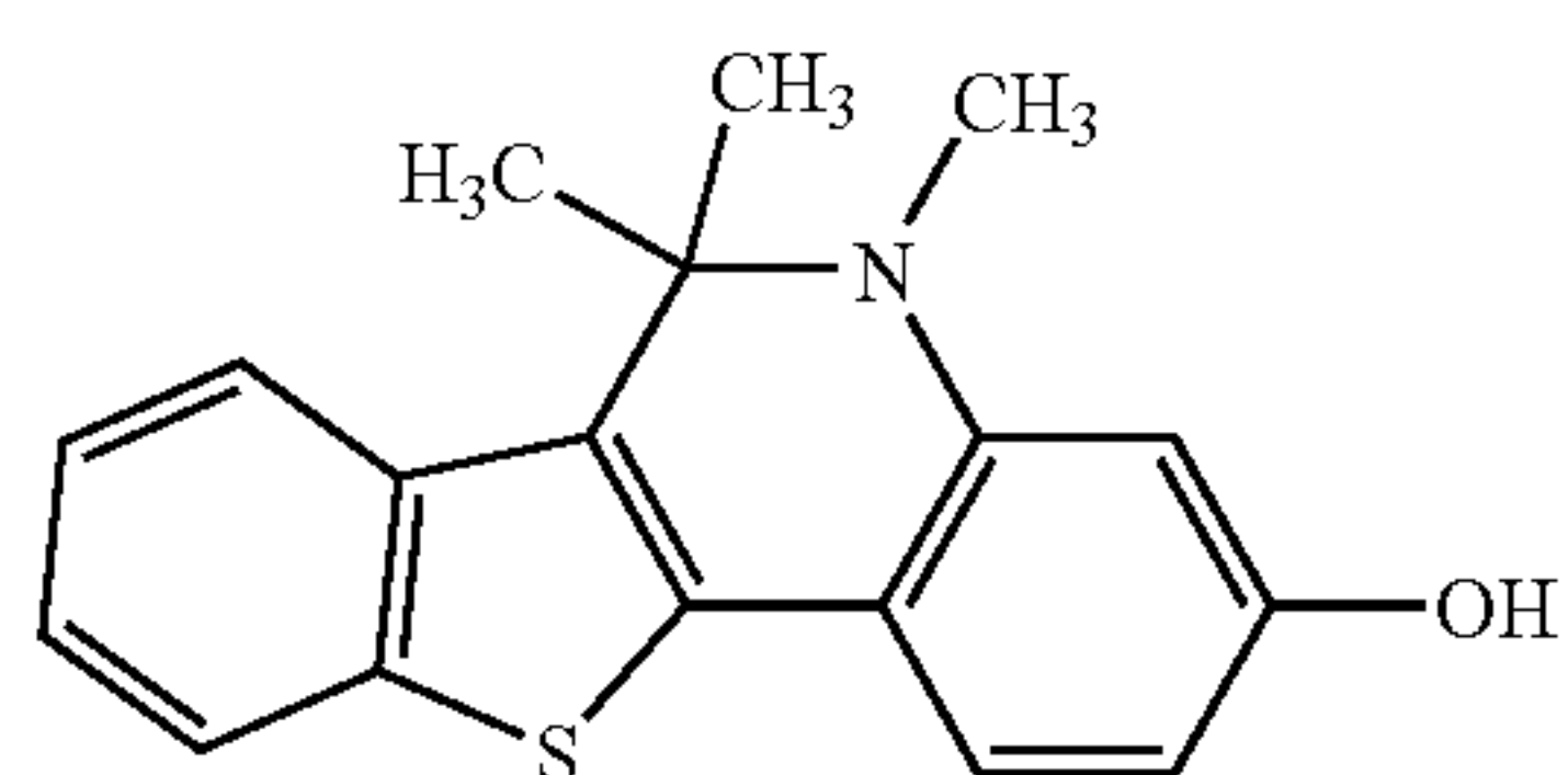
Compound 10
