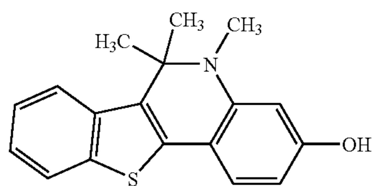
Compound 10
