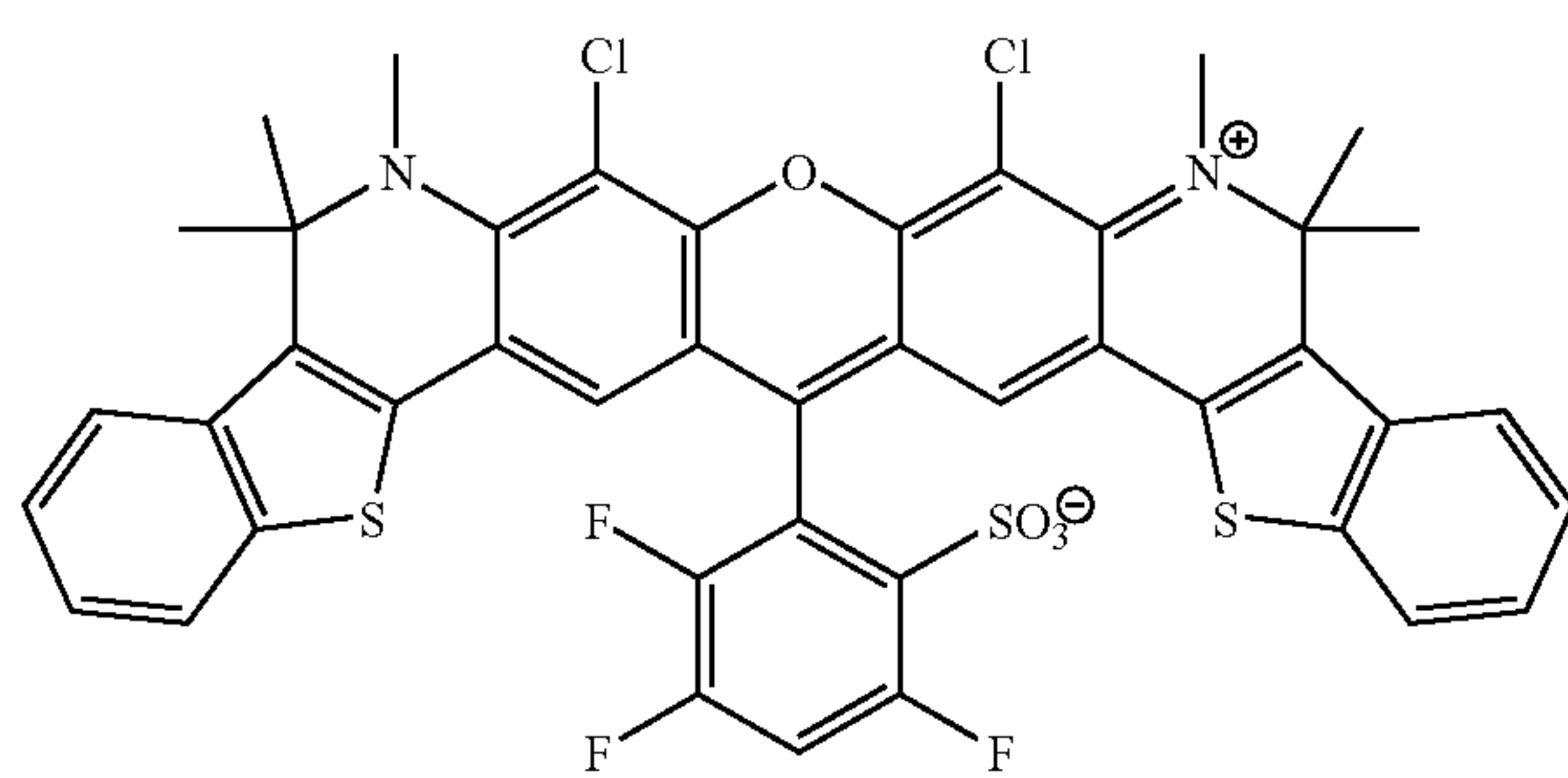
Compound 29
