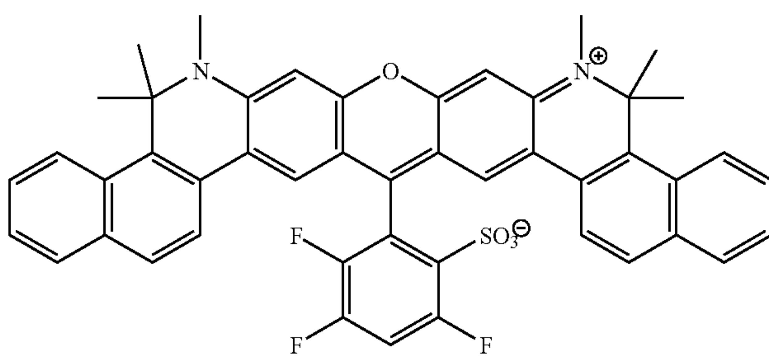
Compound 26
