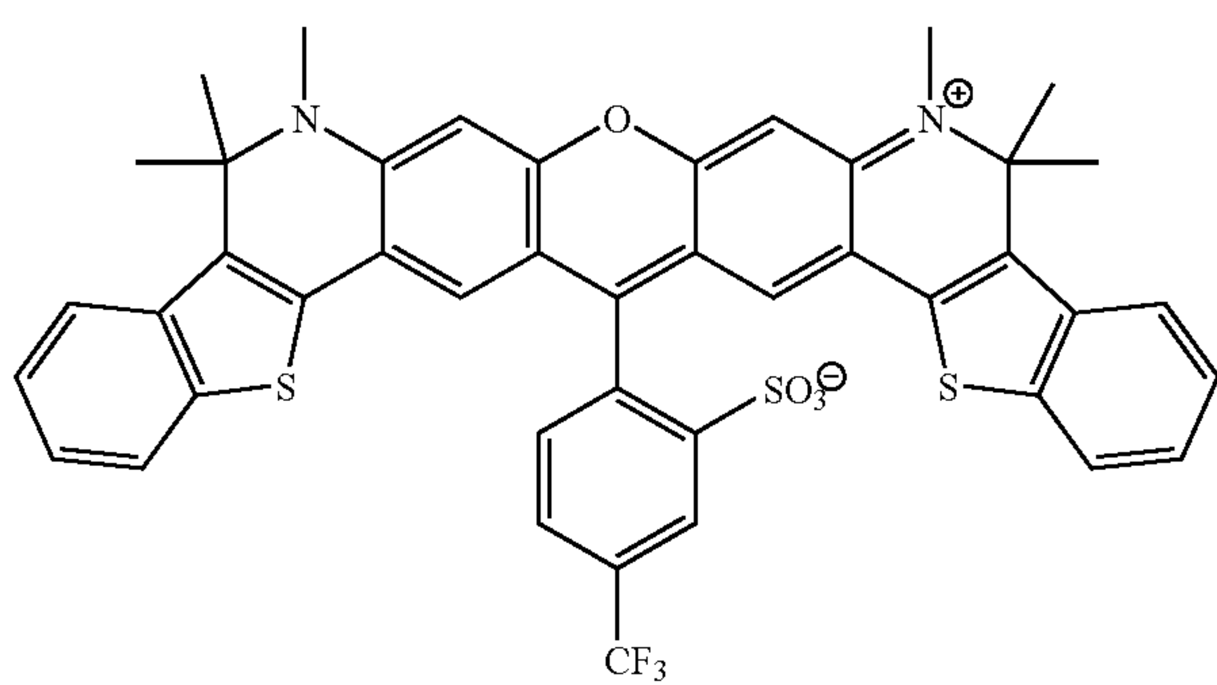
Compound 25
