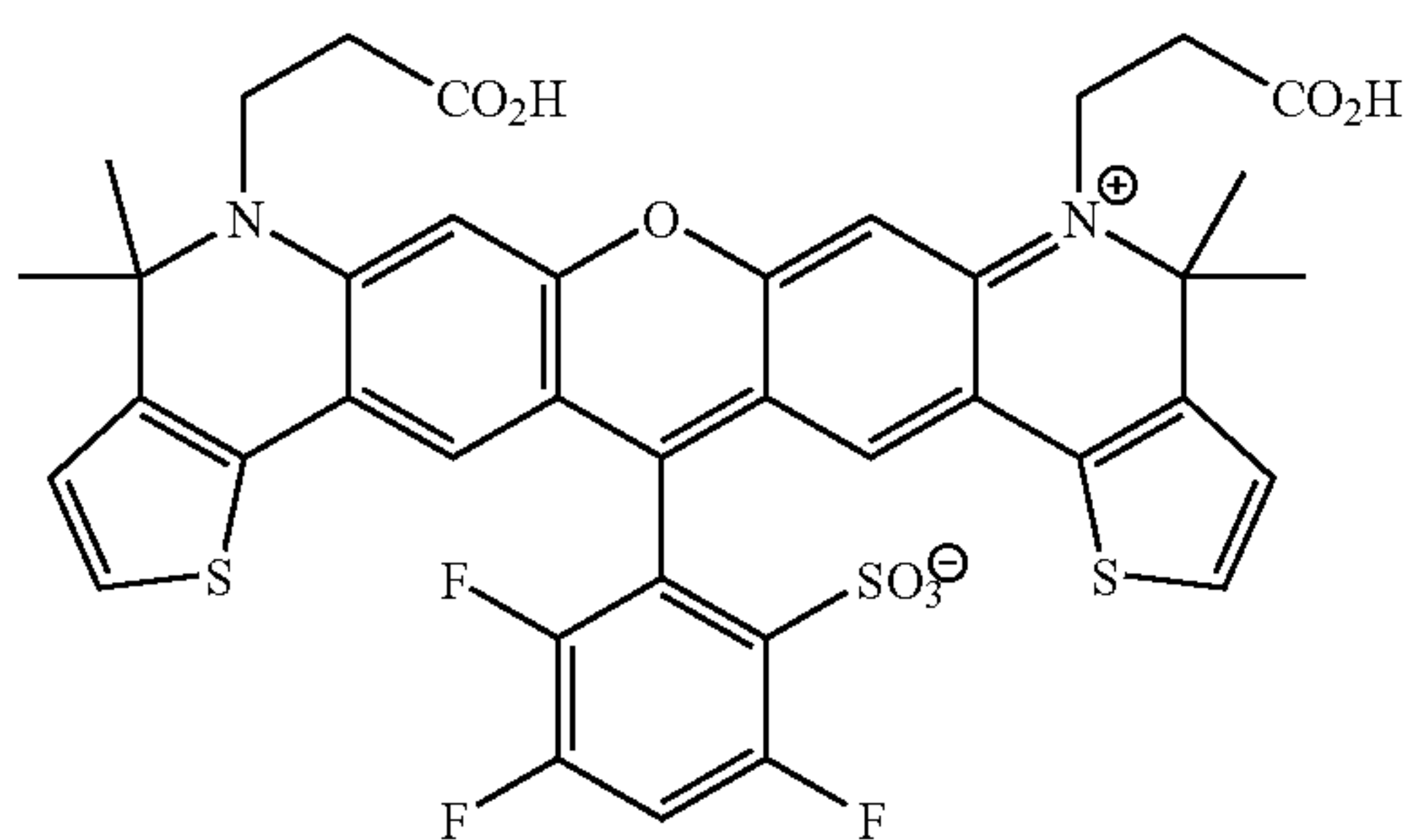
Compound 33
