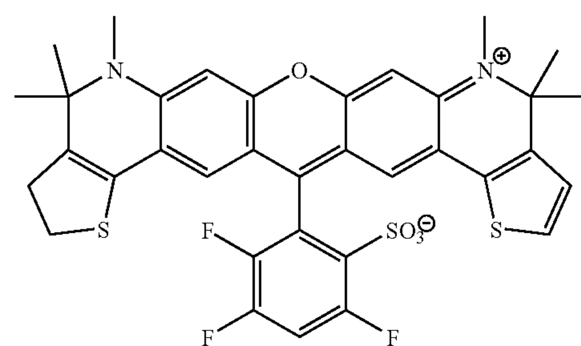
Compound 23
