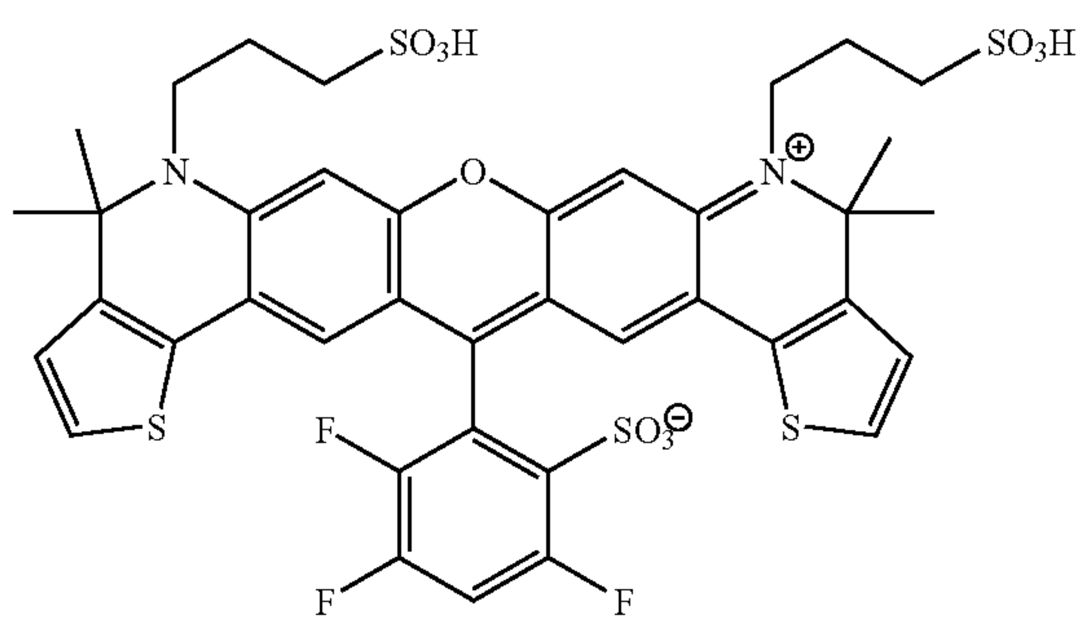
Compound 34
