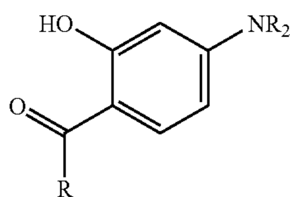
a 6-acyl-3-aminophenol
