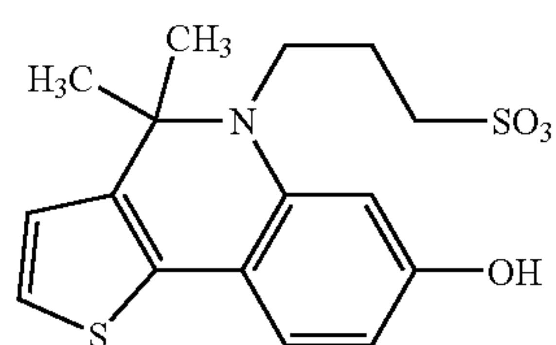
Compound 18
