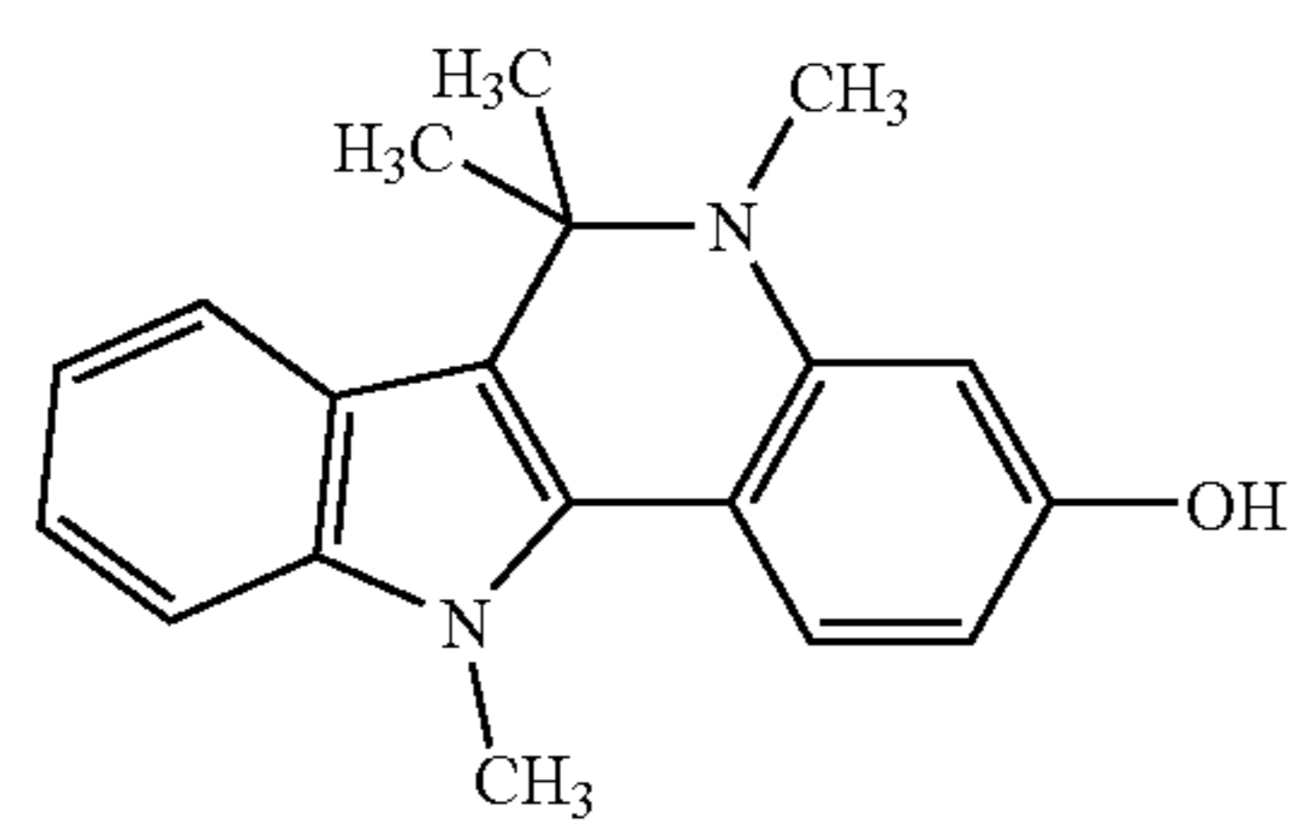
Compound 12
