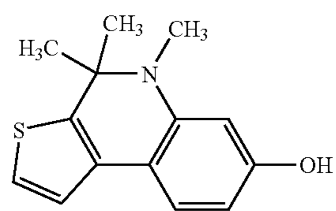
Compound 60
