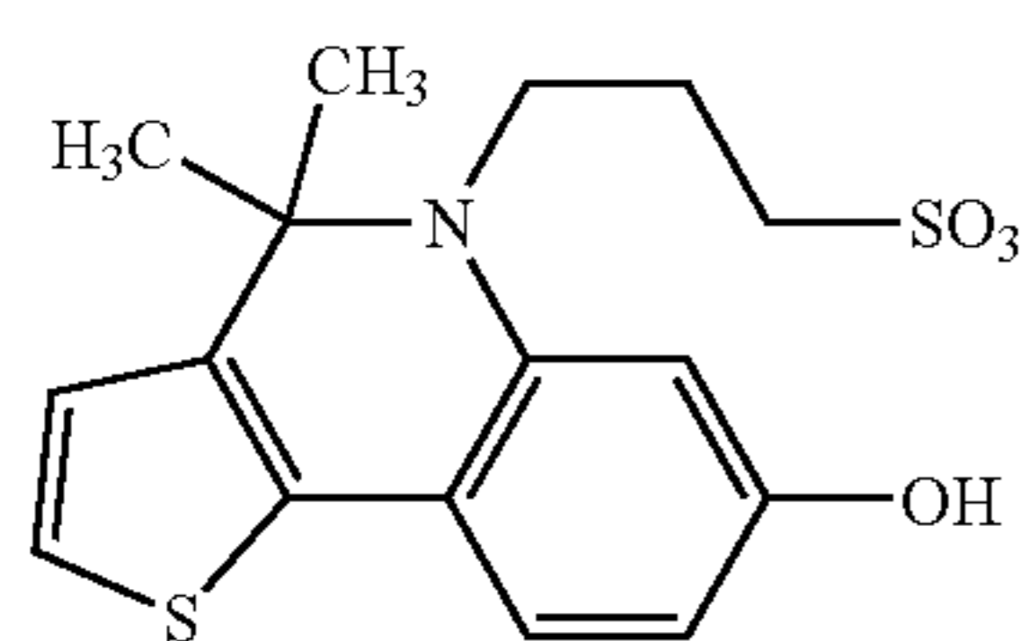
Compound 18
