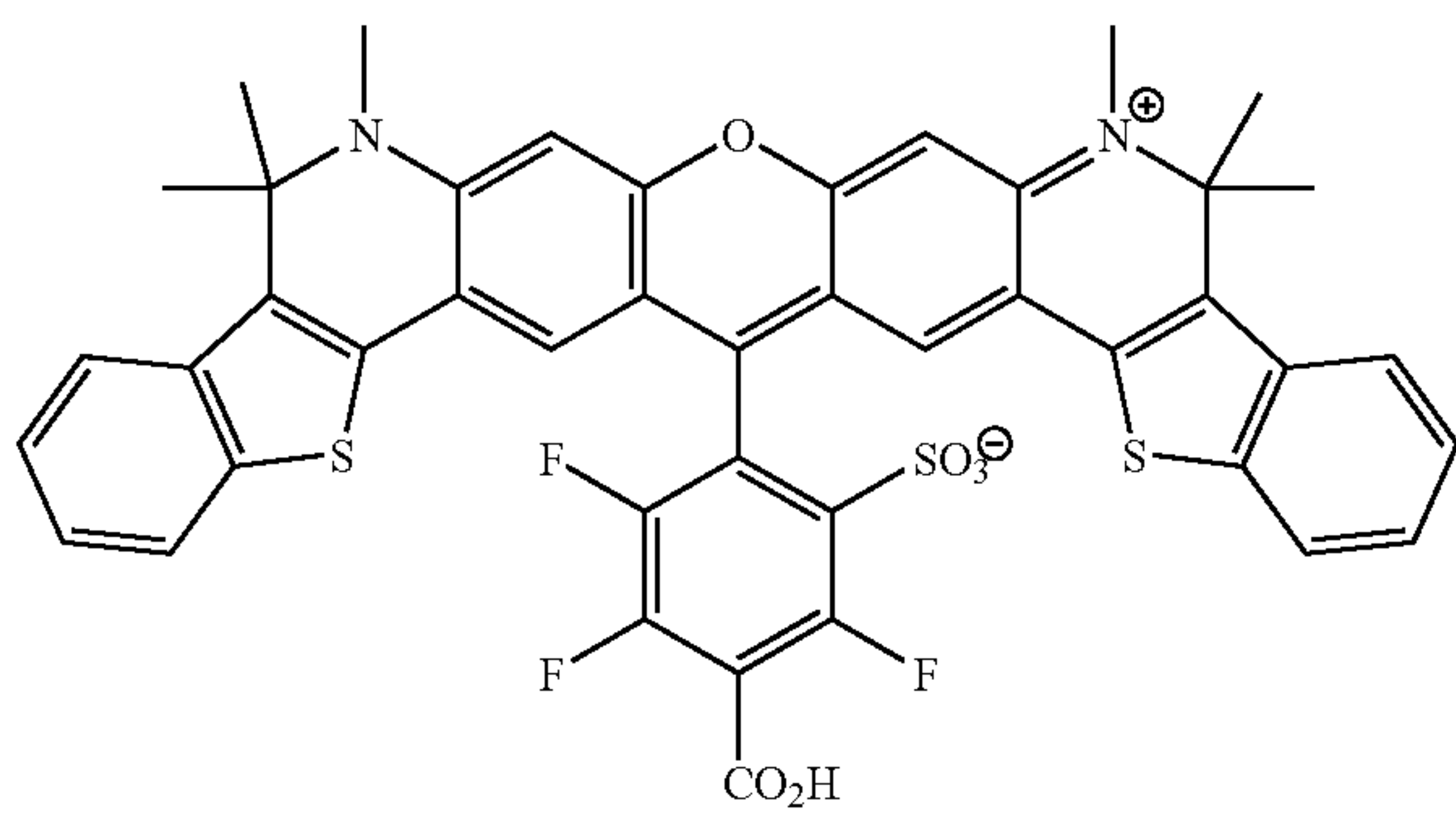
Compound 27
