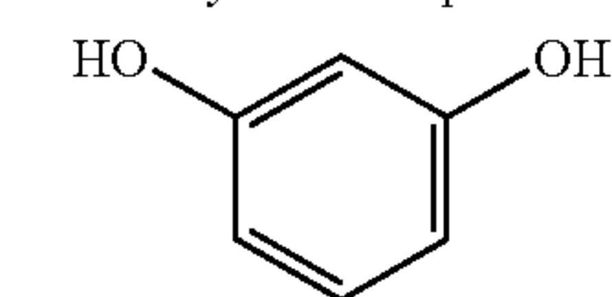
a resorcinol
