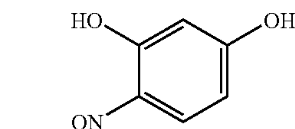
a resorcinol
