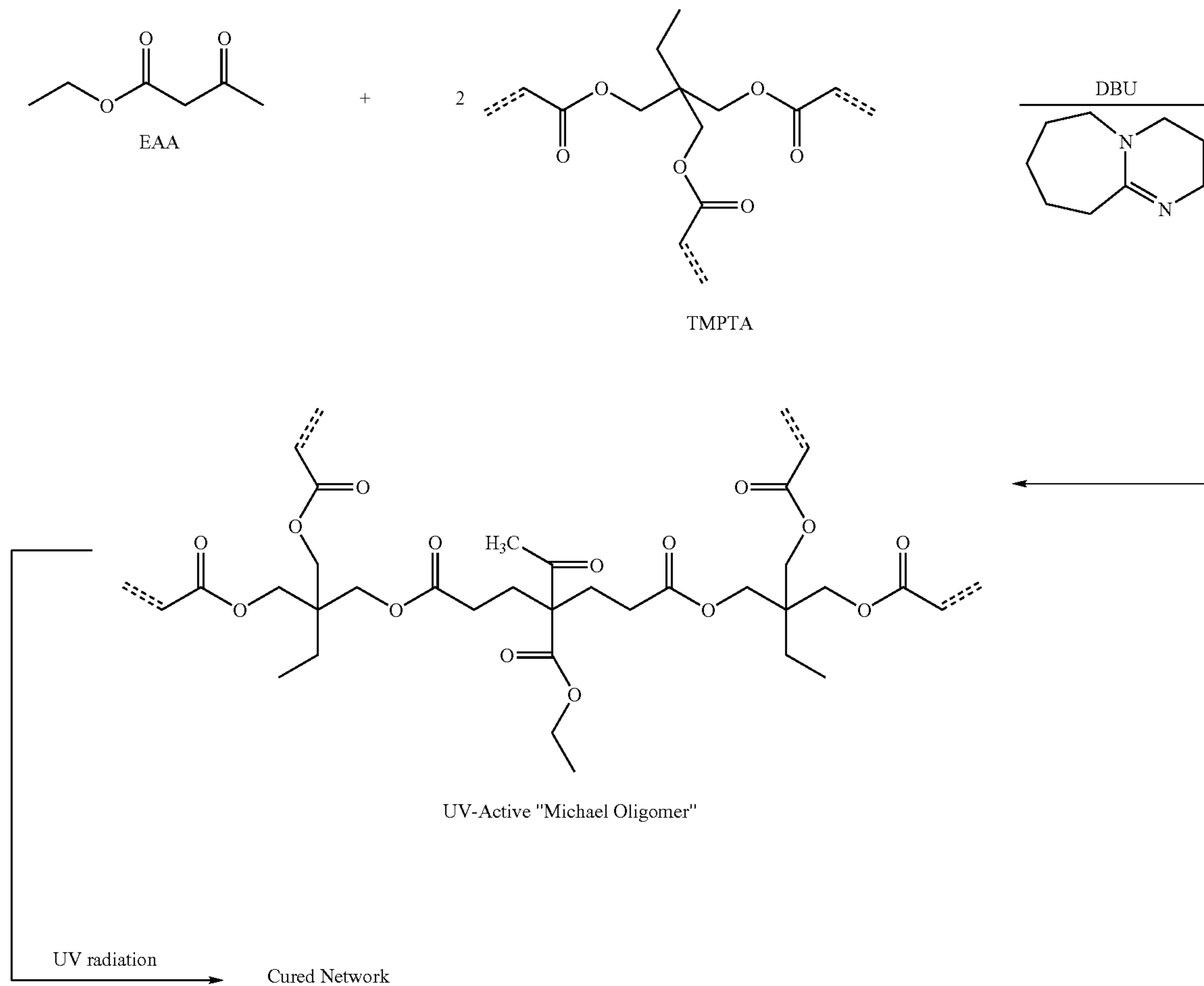
Scheme 2. Novel UV-curable oligomer from the Michael Addition reaction of trimethylolpropane triacrylate (TMPTA) and ethyl acetoacetate (EAA).
