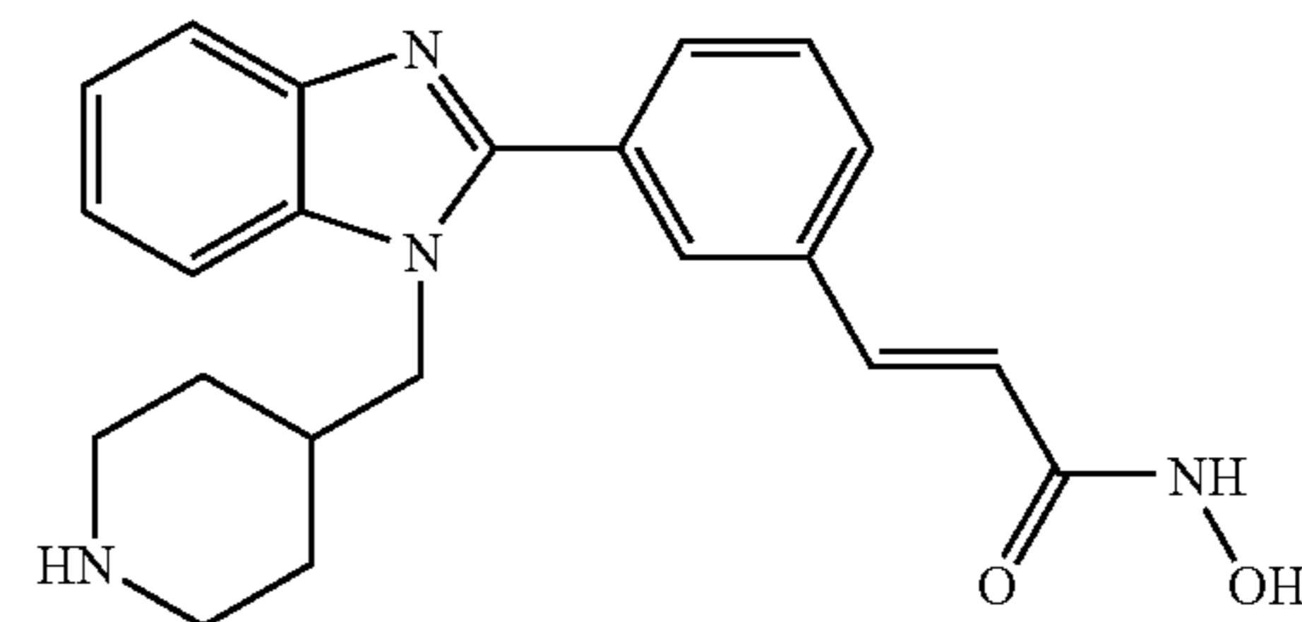
N-Hydroxy-3-[3-(1-piperidin-4-ylmethyl-1H-benzoimidazol-2-yl)-phenyl]-acrylamide.
