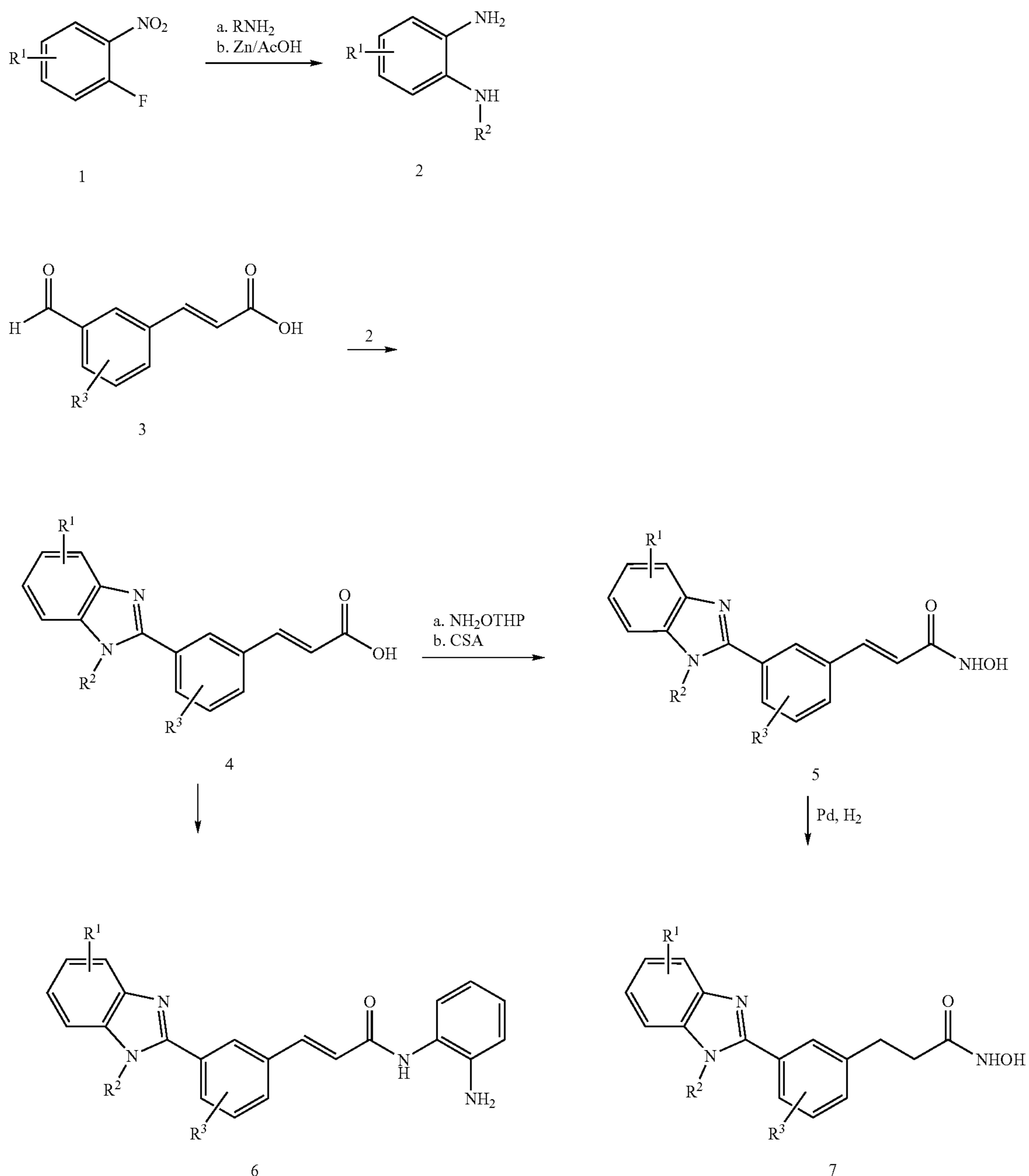
Scheme 1:
