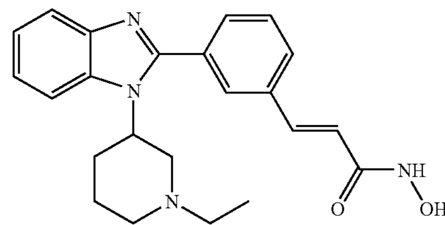
(±)-3-{3-[1-(1-Ethyl-piperidin-3-yl)-1H-benzoimidazol-2-yl]-phenyl}-N-hydroxy-acrylamide.
