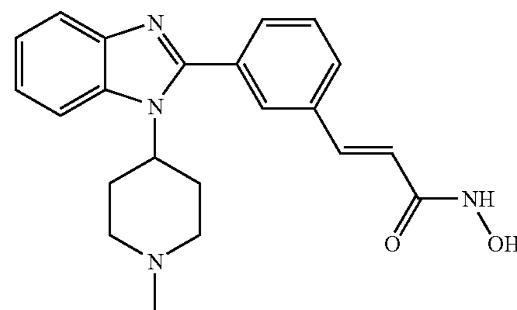
N-Hydroxy-3-{3-[1-(1-methyl-piperidin-4-yl)-1H-benzoimidazol-2-yl]-phenyl}-acrylamide.
