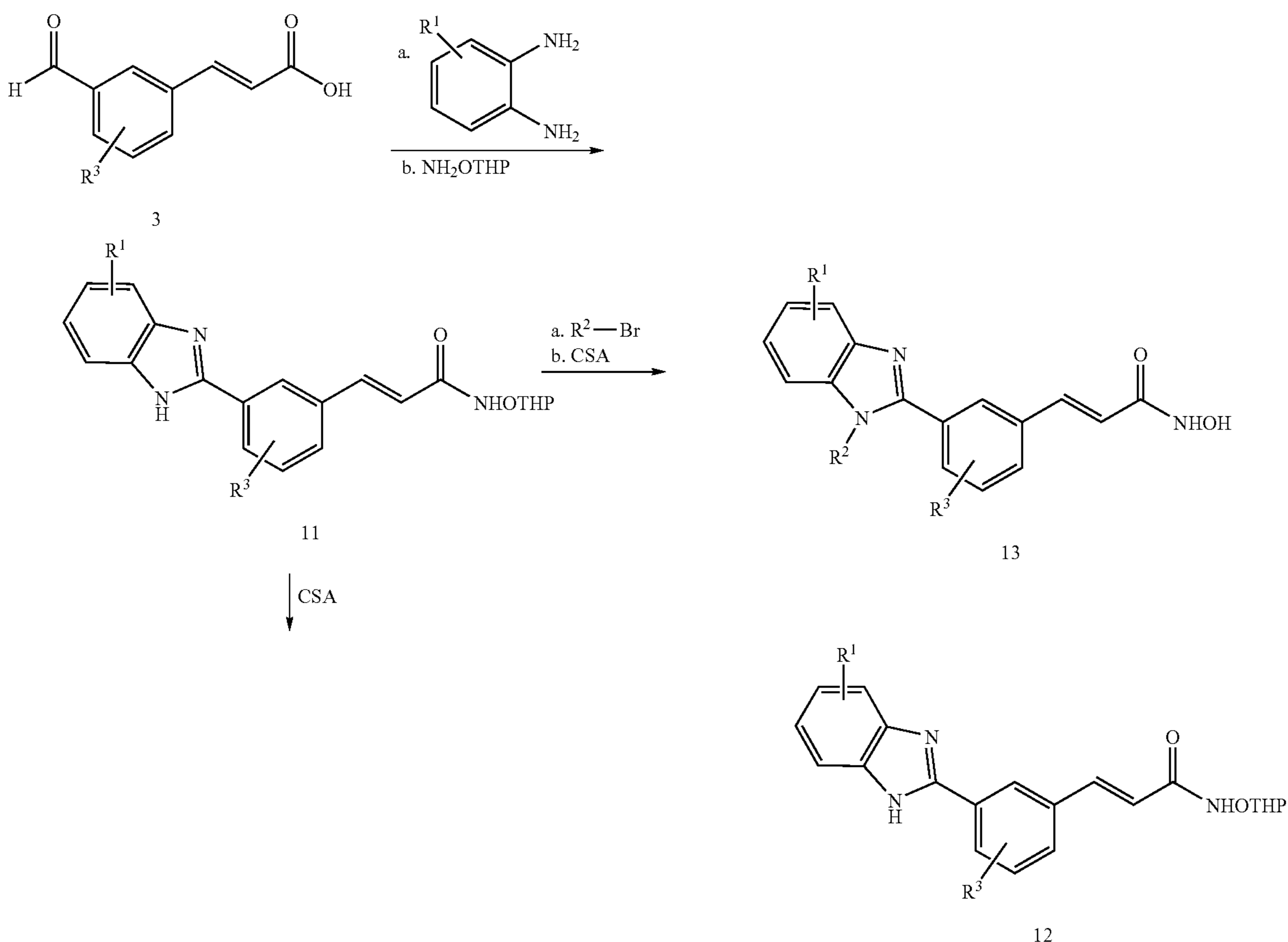
Scheme 3:
