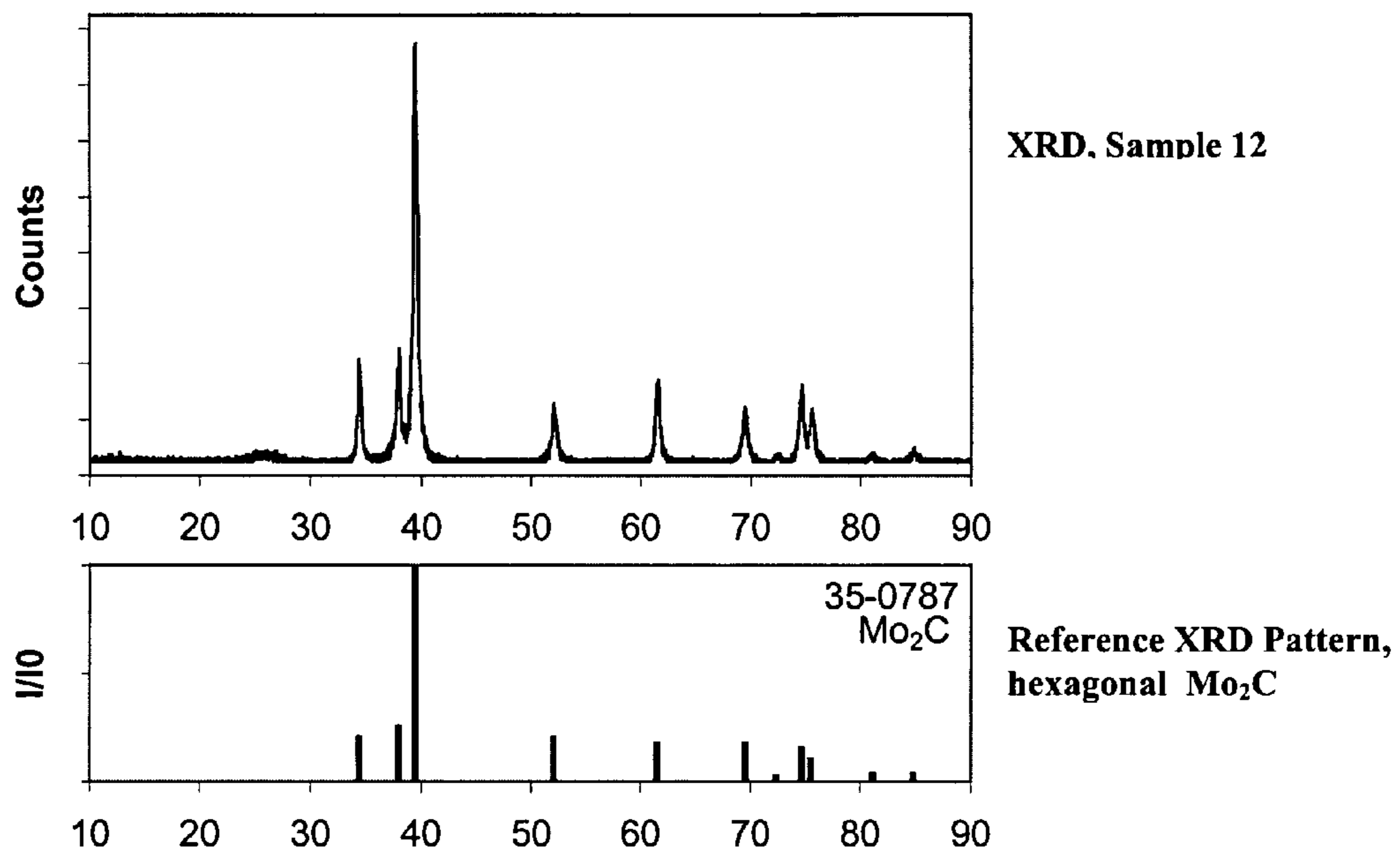
FIG. 1A XRD and SEM of CARBON NANORODS
