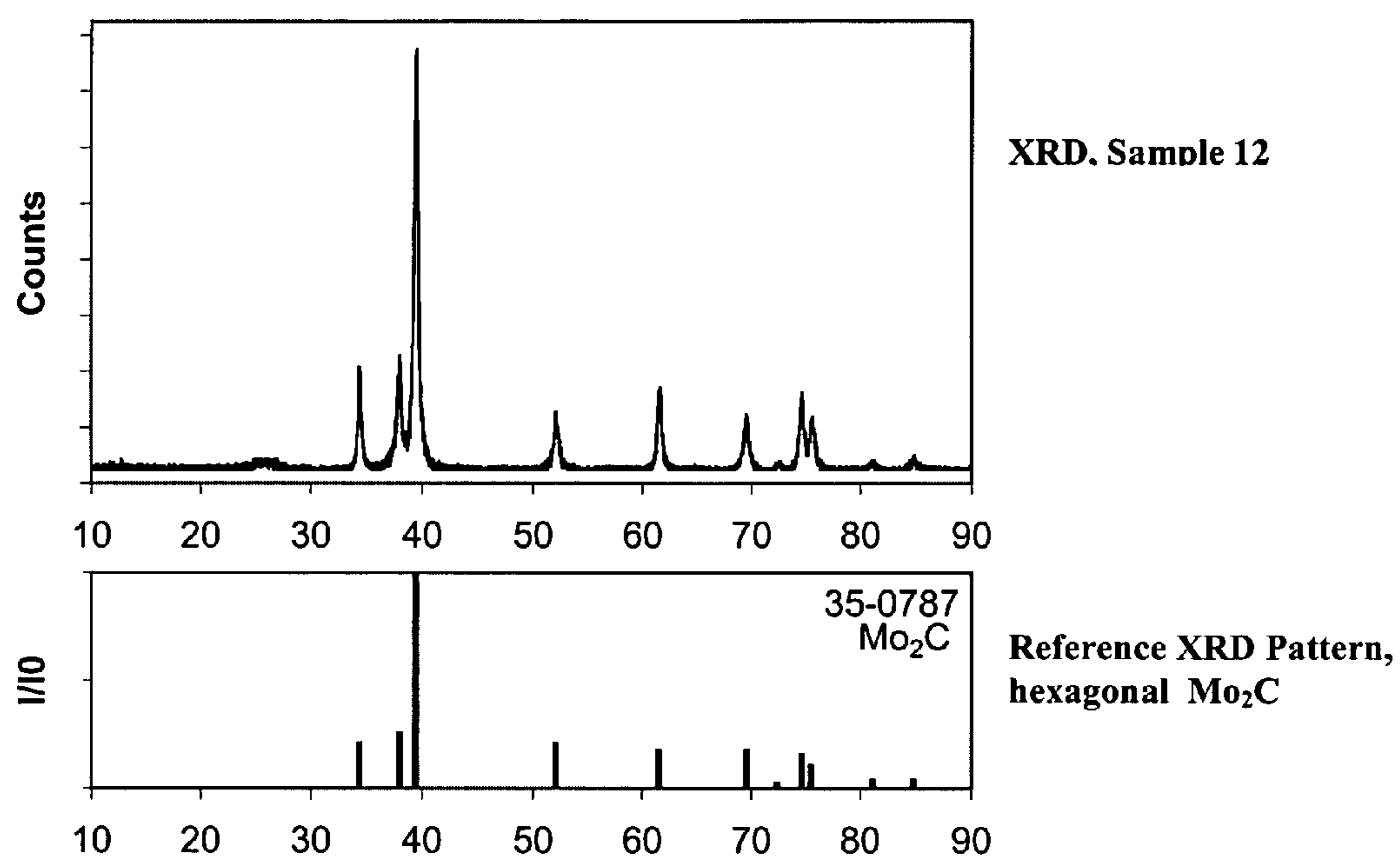
FIG. 2A XRD and HRTEM of CARBIDE NANORODS
