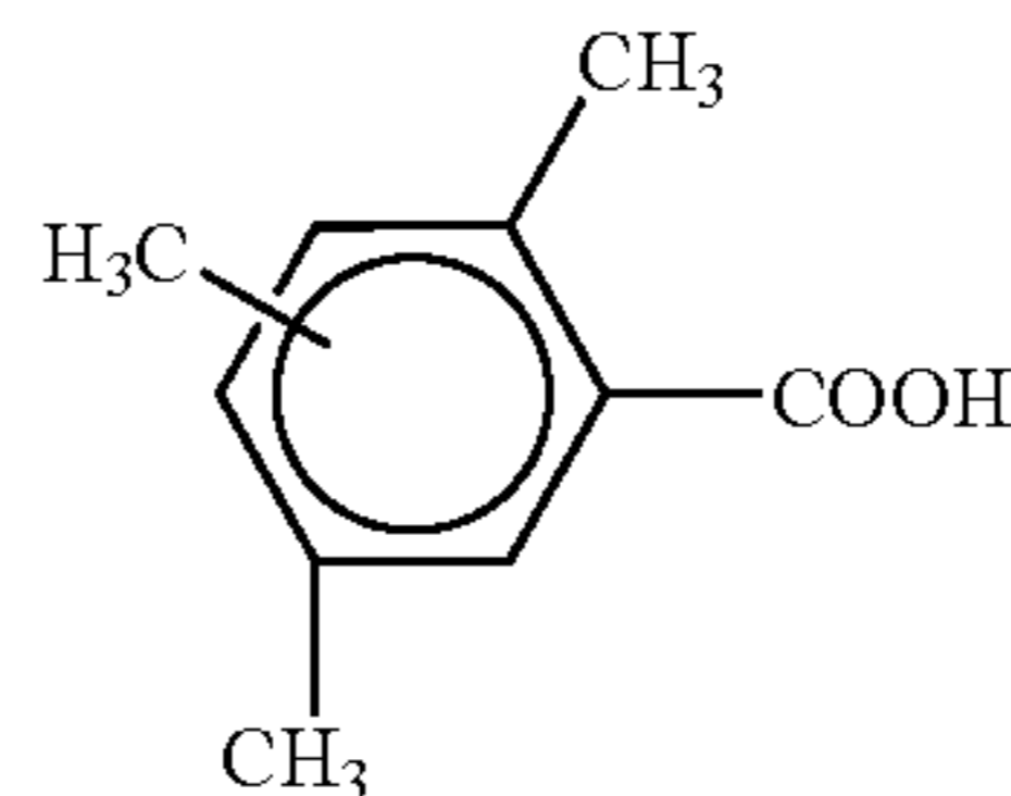
(10) Cyclohexylcarboxylic acid
