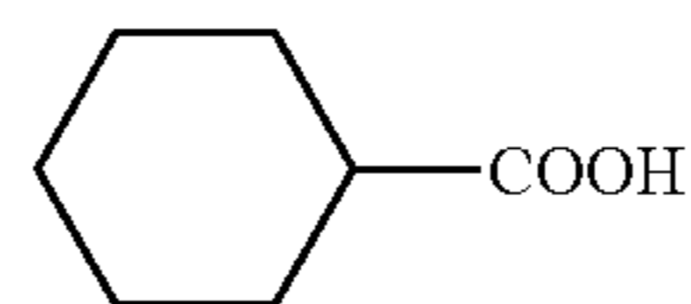
(11) Salt of the above-mentioned carboxylic acid
