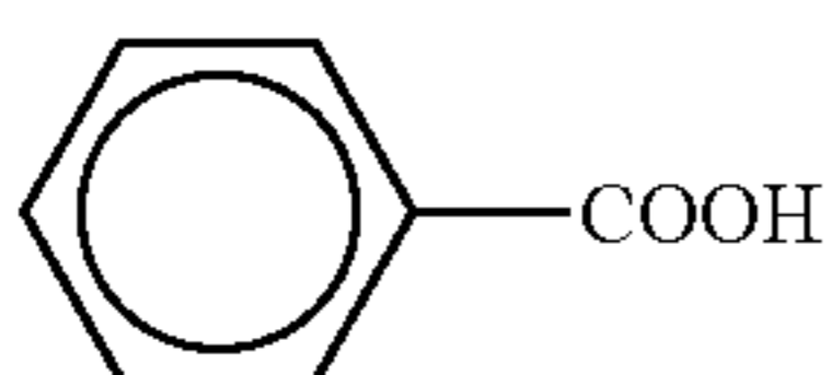
(1) Benzoic acid
