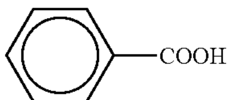
(1) Benzoic acid
