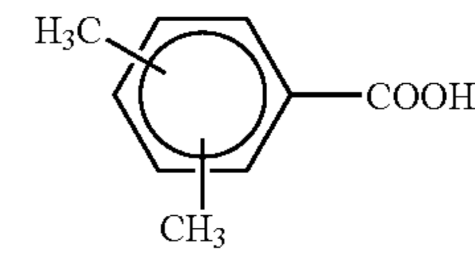
(9) Trimethylbenzoic acid
