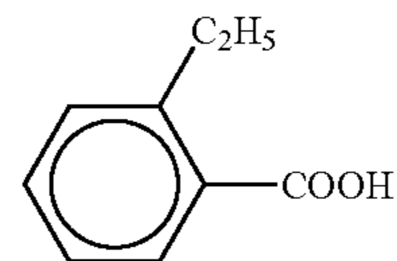
(8) Dimethylbenzoic acid
