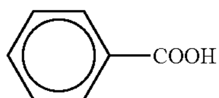
(1) Benzoic acid
