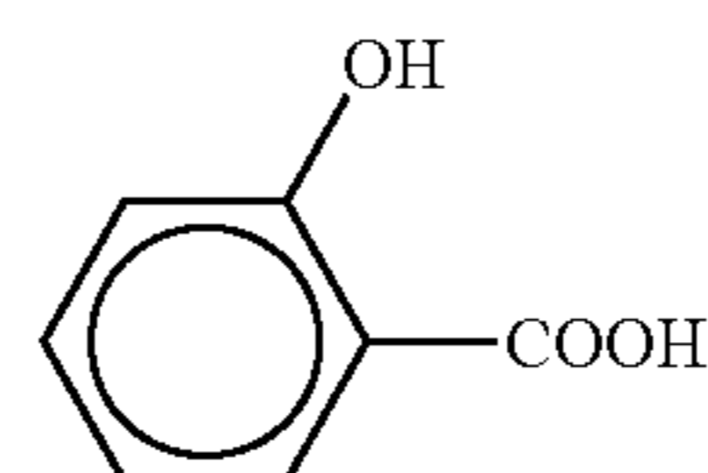
(6) Toluic acid (methylbenzoic acid)
