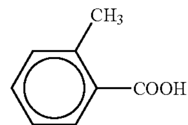
(7) O-ethylbenzoic acid
