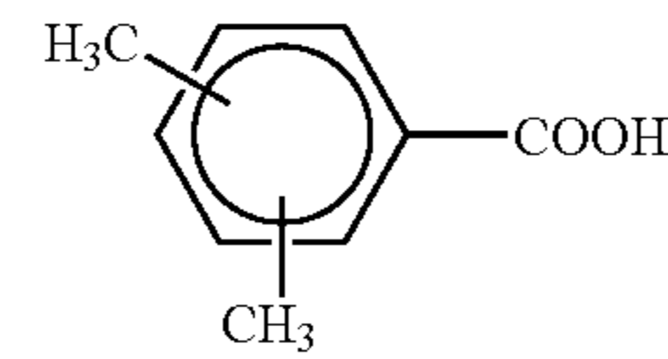
(9) Trimethylbenzoic acid
