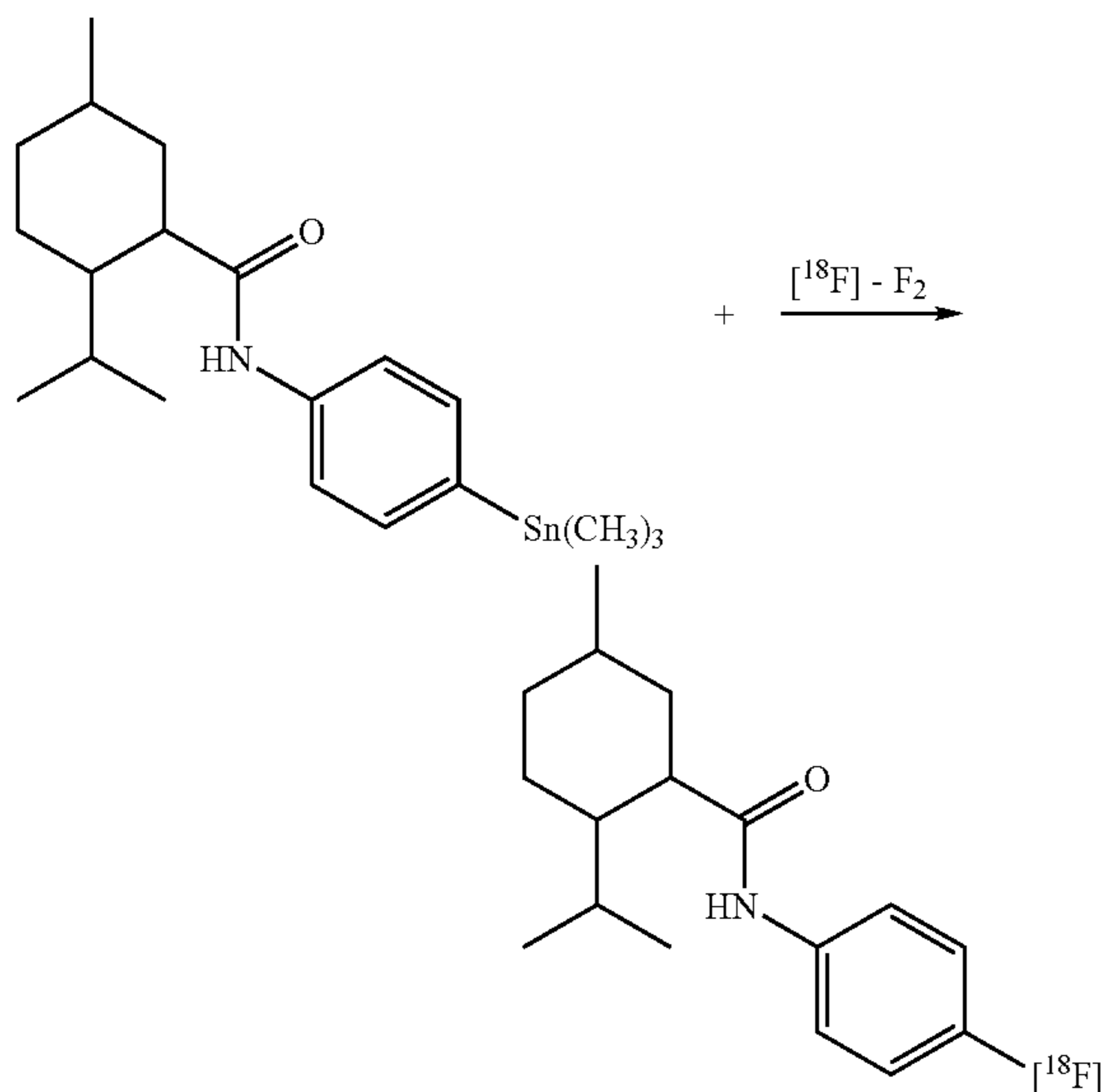
Schematic 2
