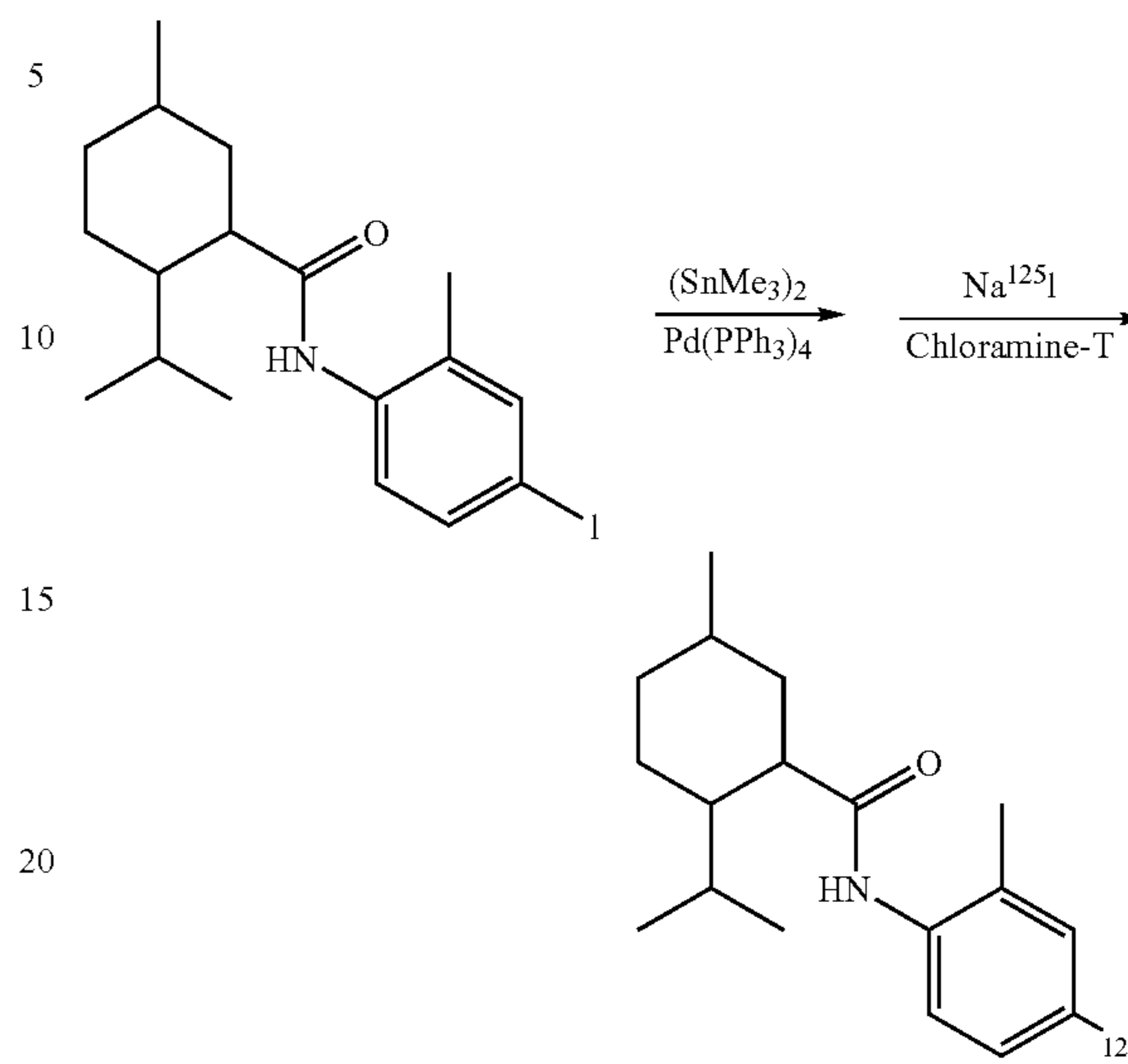
Schematic 3
