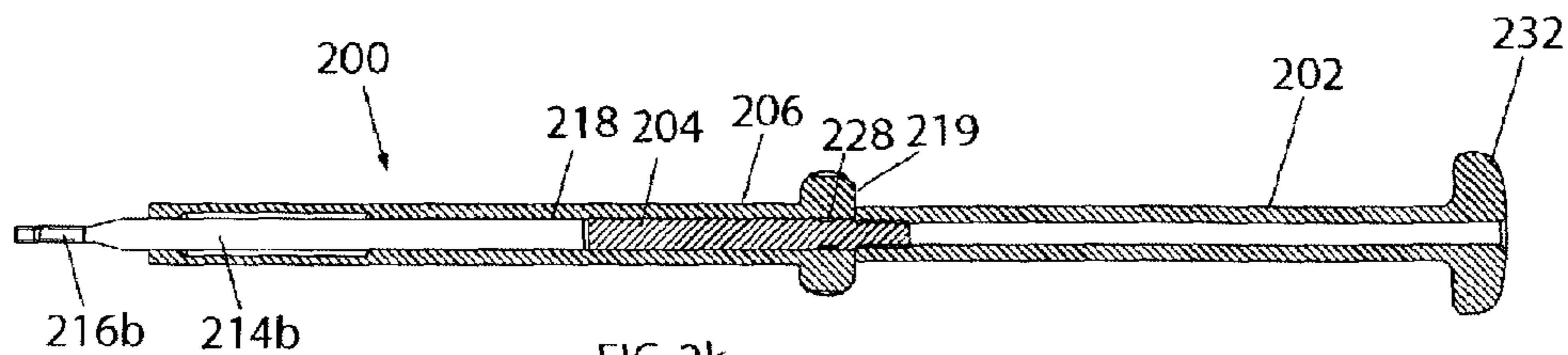
FIG. 2k (Section A-A of Fig. 2b)
