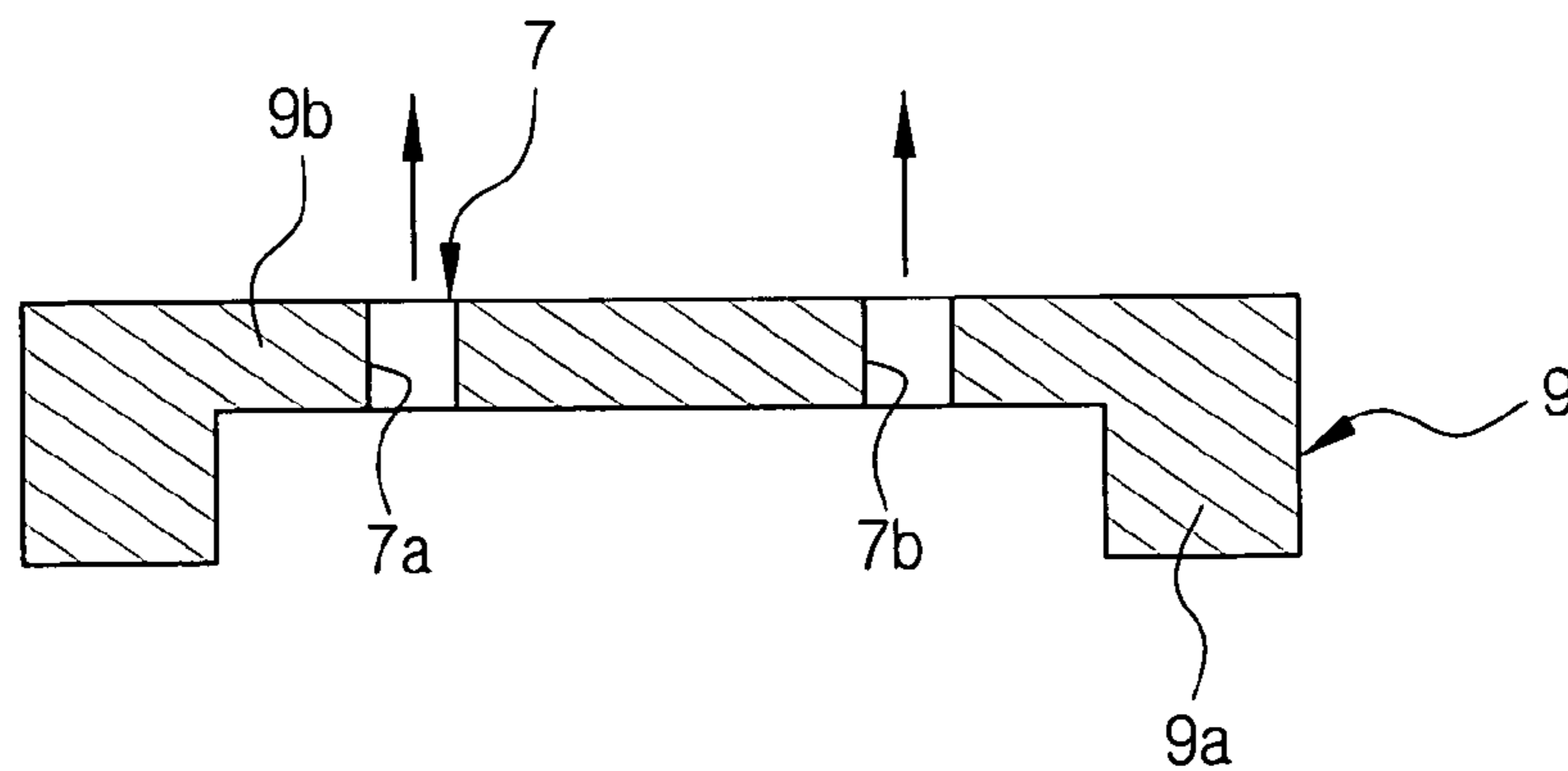
FIG. 5C (PRIOR ART)
