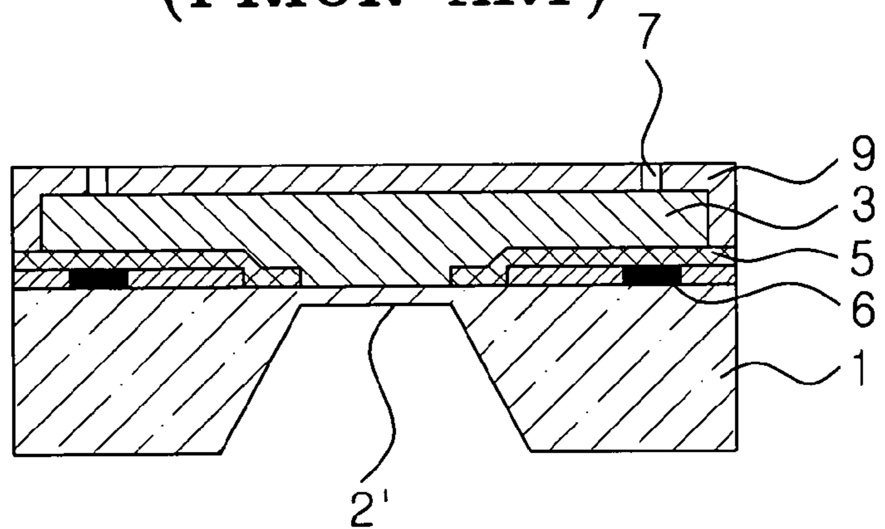
FIG. 2C (PRIOR ART)
