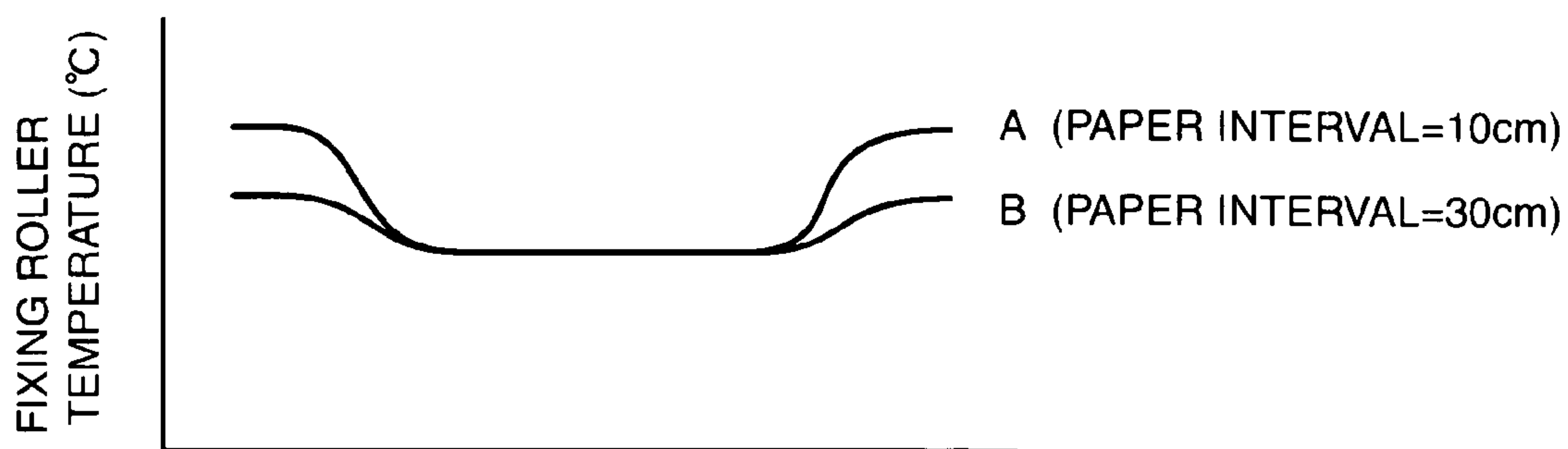
TEMPERATURE IN LONGITUDINAL DIRECTION OF FIXING ROLLER (°C) (A4 SIZE)
