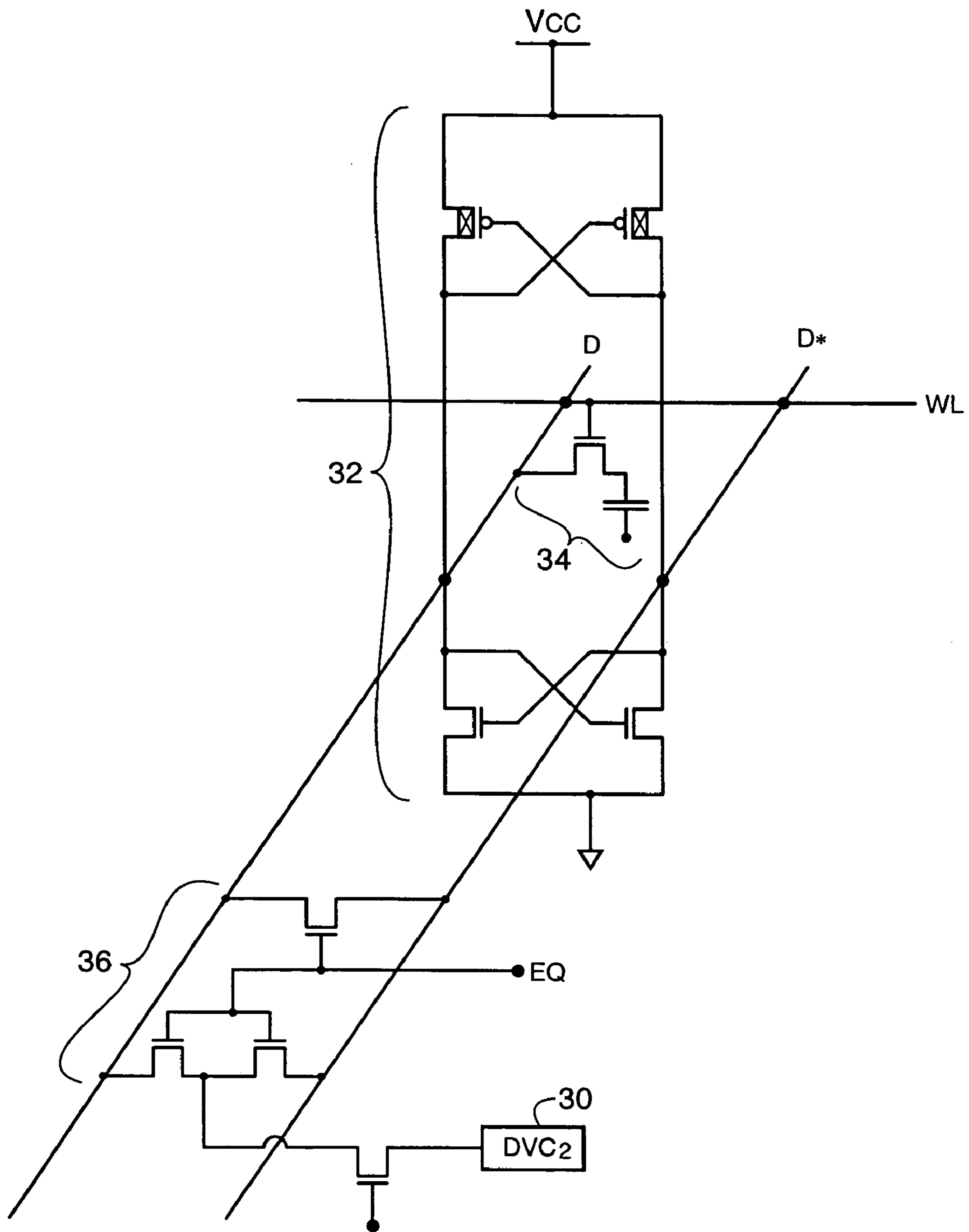
FIG. 5 (PRIOR ART)
