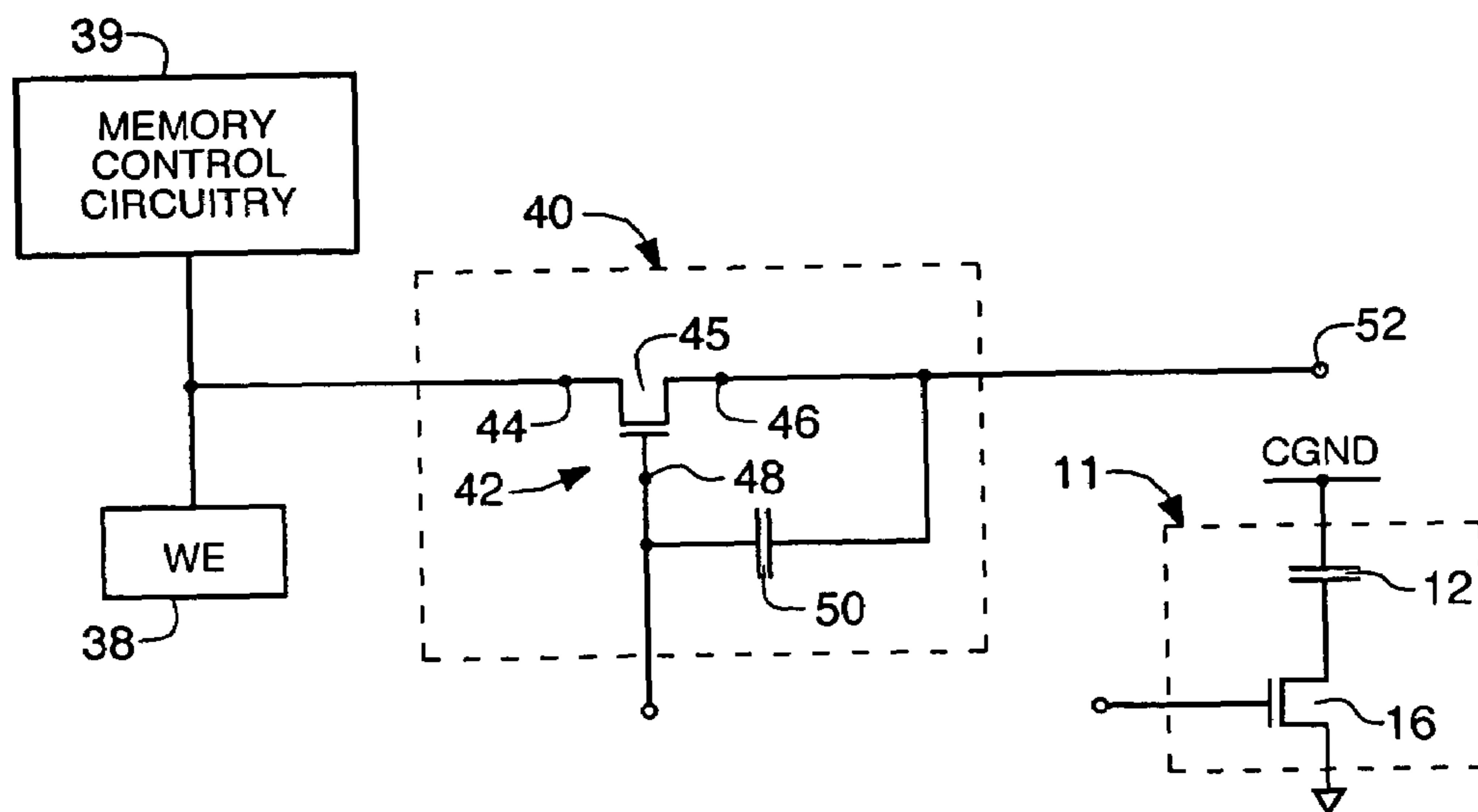
FIG. 2 (PRIOR ART)
