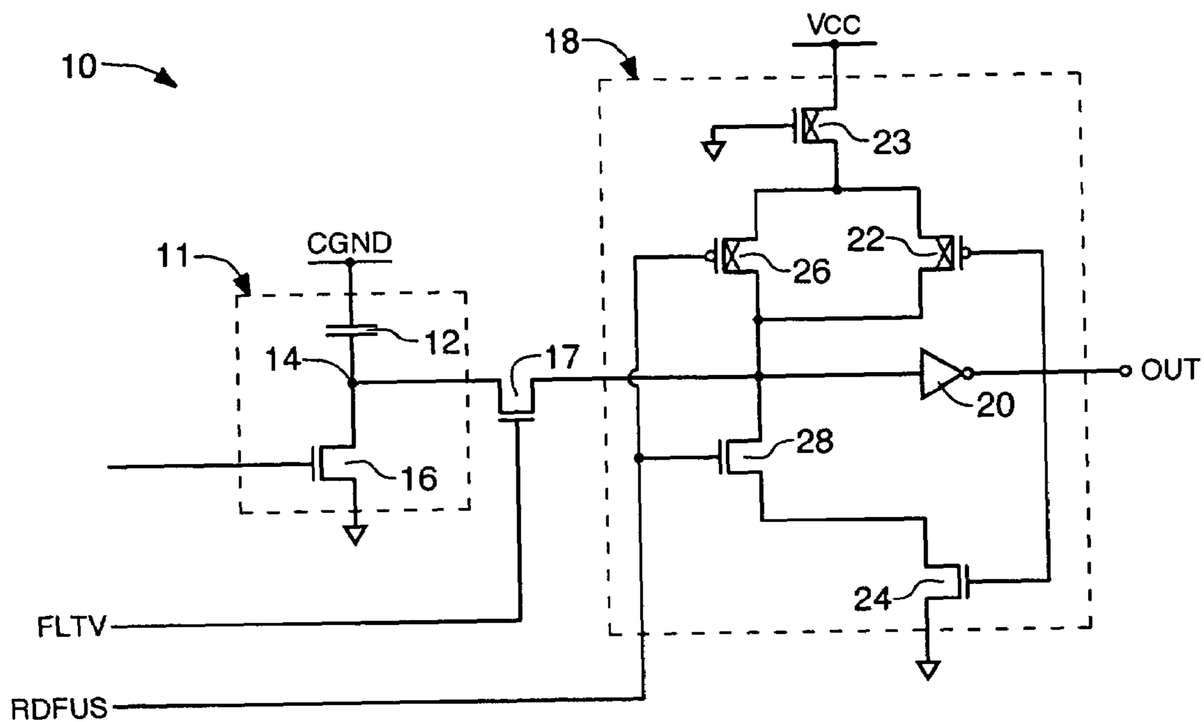
FIG. 1 (PRIOR ART)
