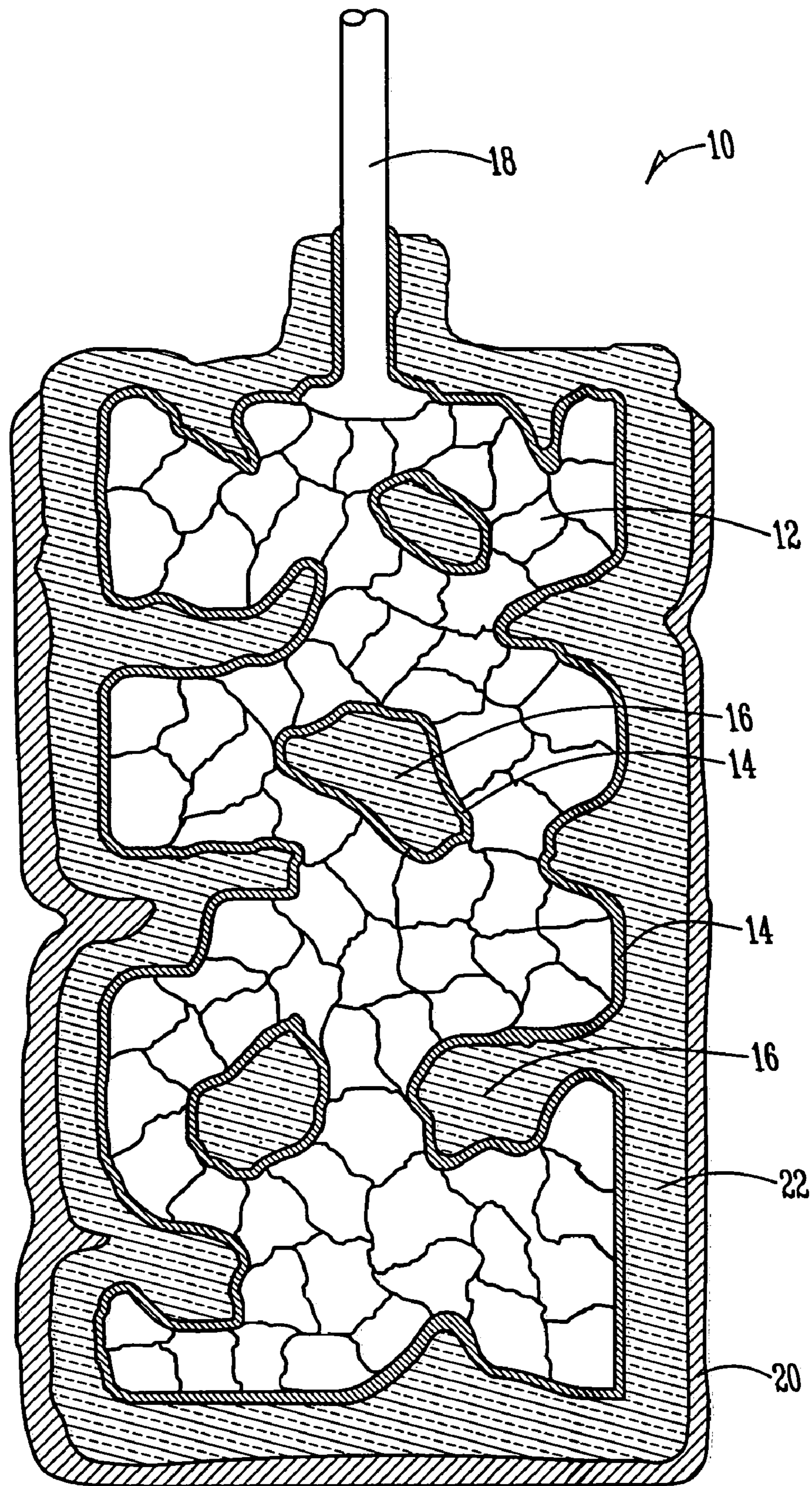
Fig. 10 (PRIOR ART)
