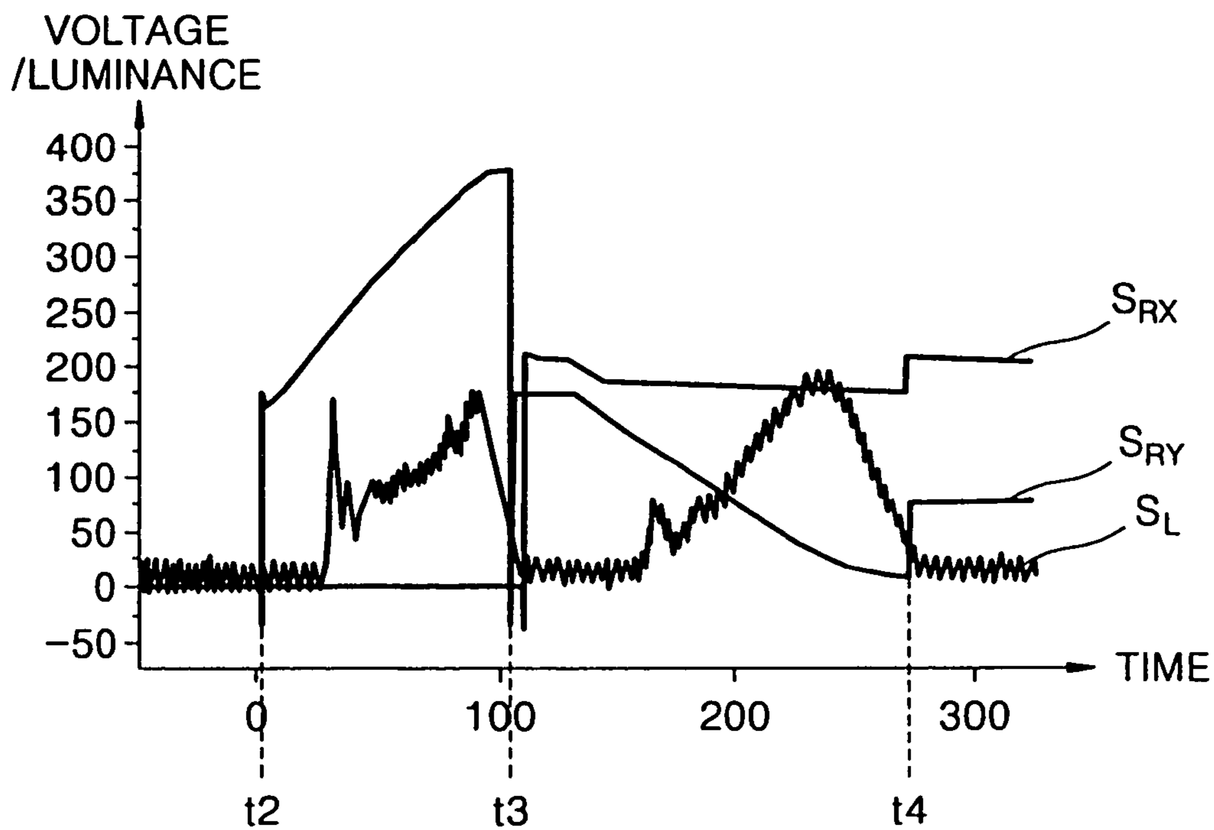
FIG. 8 (PRIOR ART)
