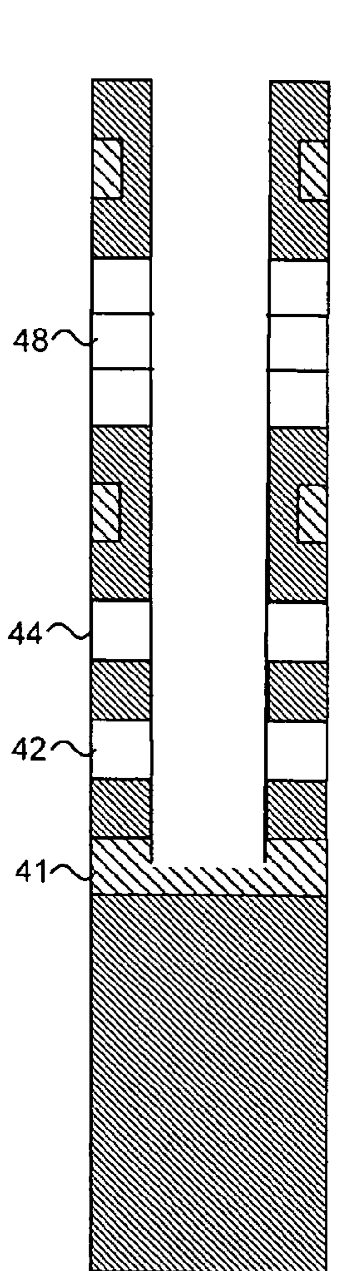
timed etch into n+ red diode layer
