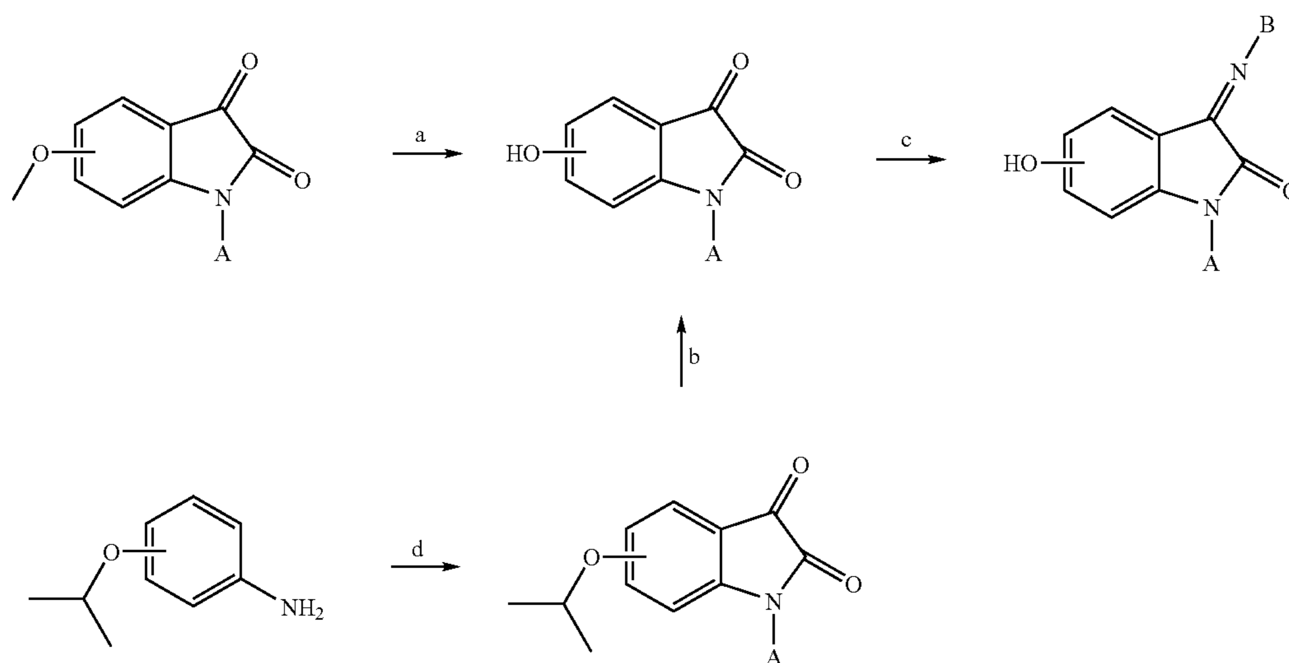
Scheme 3. Synthesis of Hydroxy-3-imino-2-indolones.
