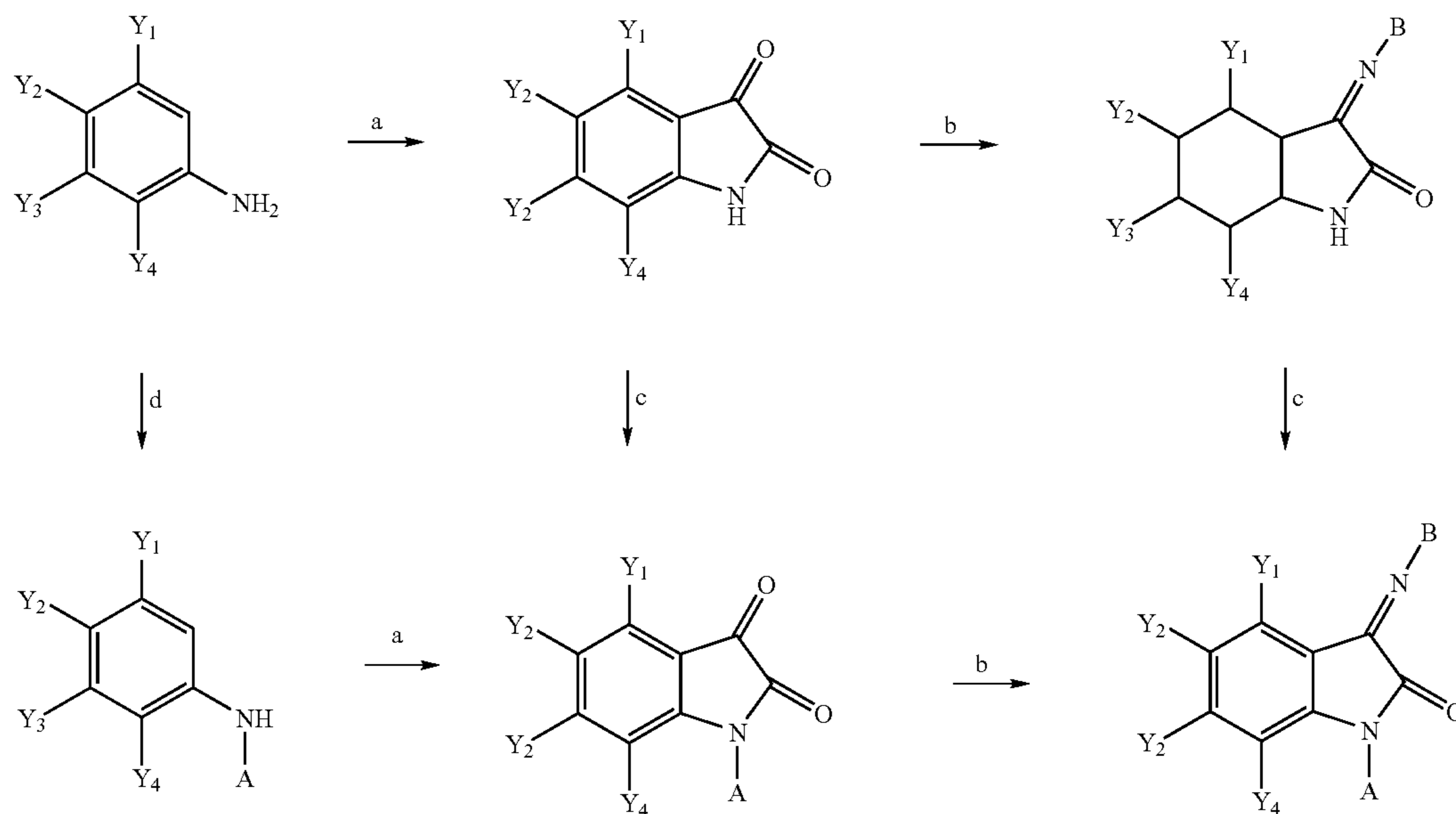
Scheme 1. Synthesis of N-Aryl-3-imino-2-indolones.
