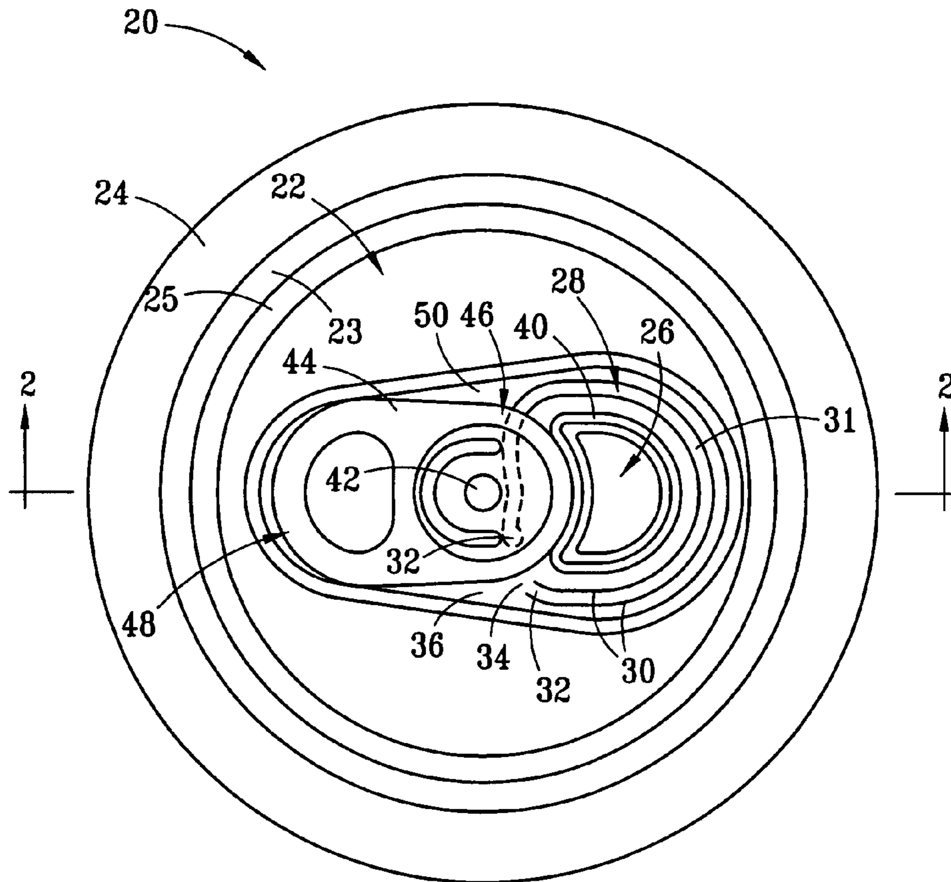
FIG. 1 (PRIOR ART)
