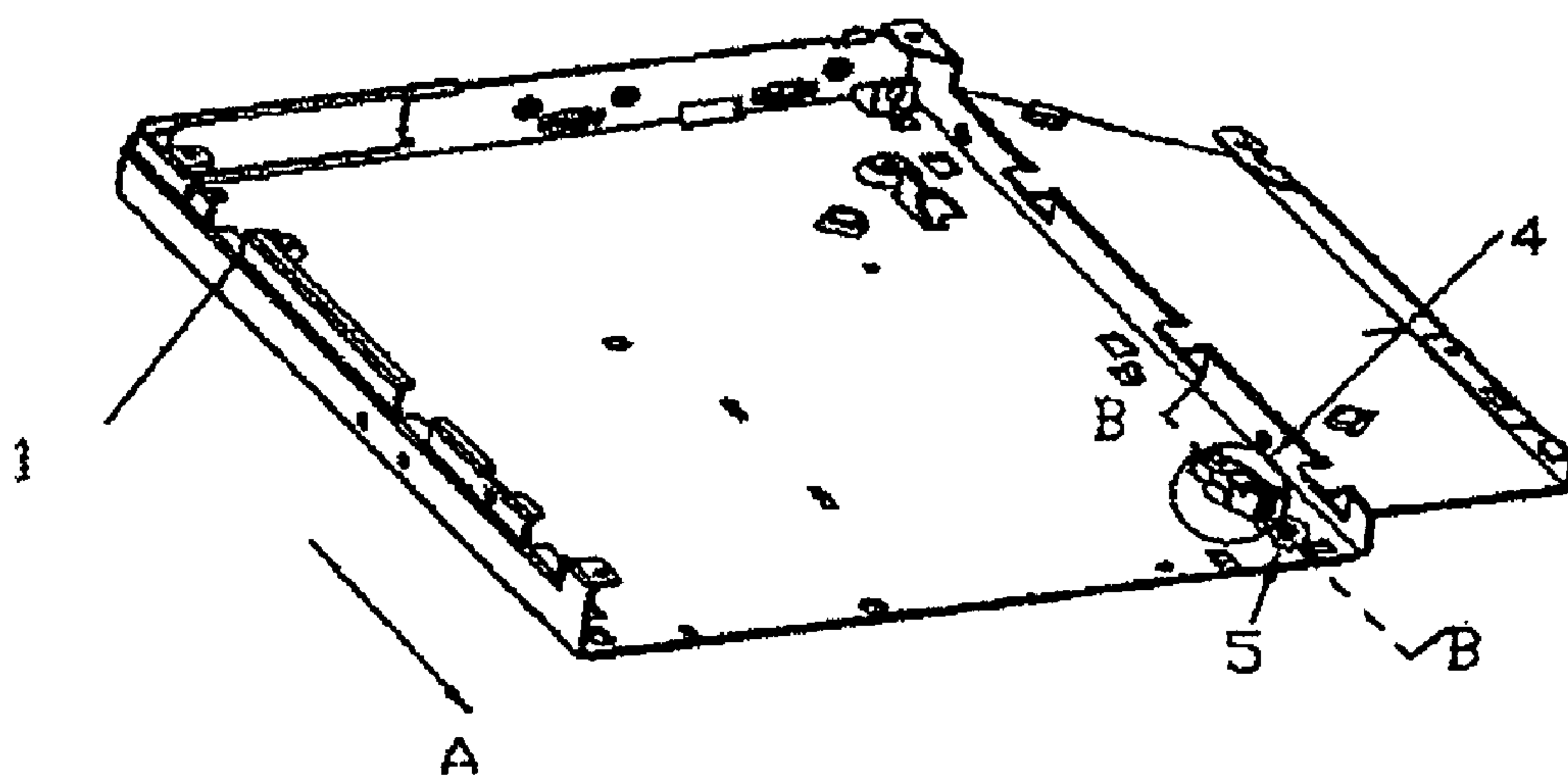
FIG. 2 (Prior Art)
