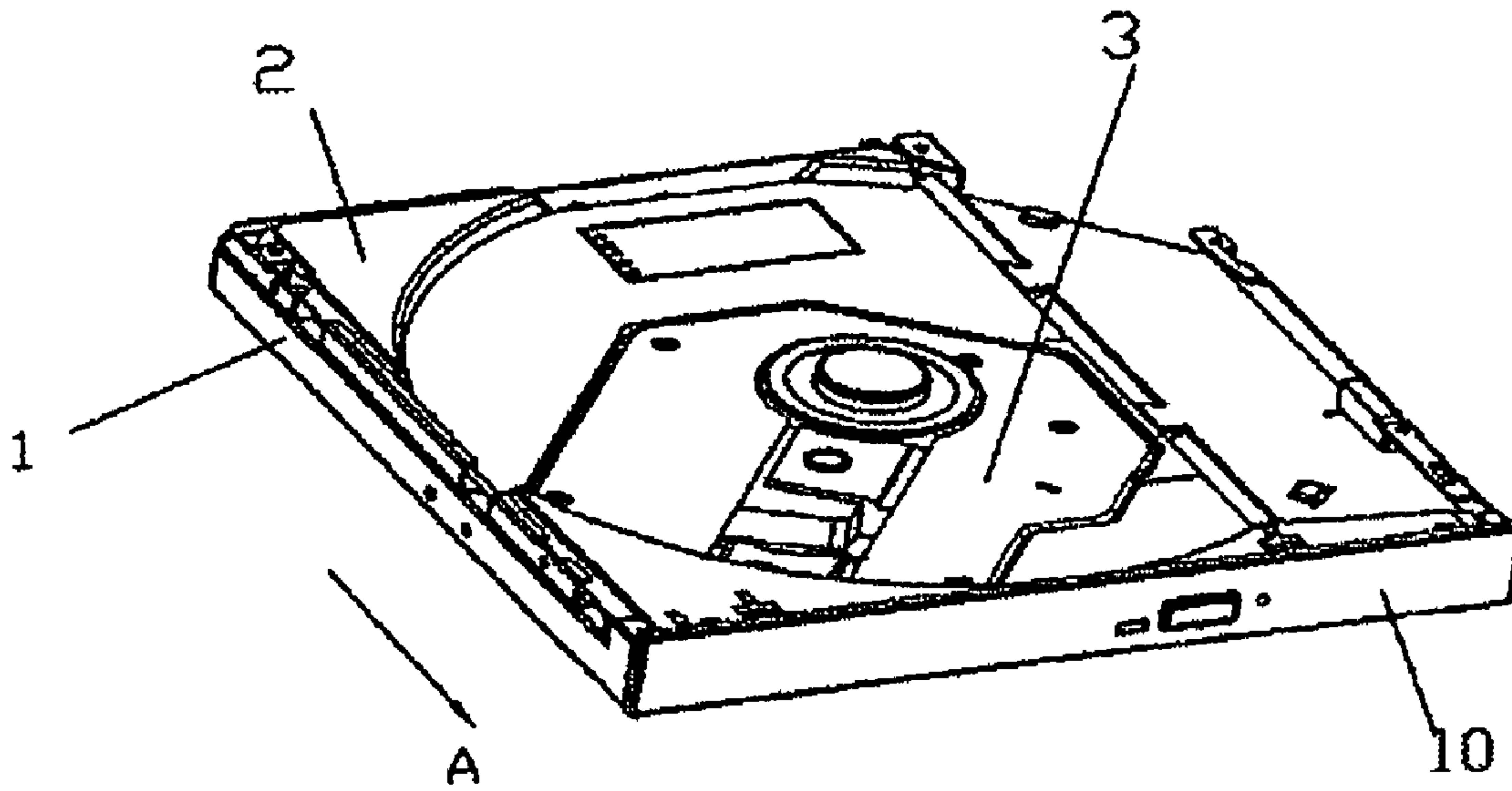
FIG. 1 (Prior Art)
