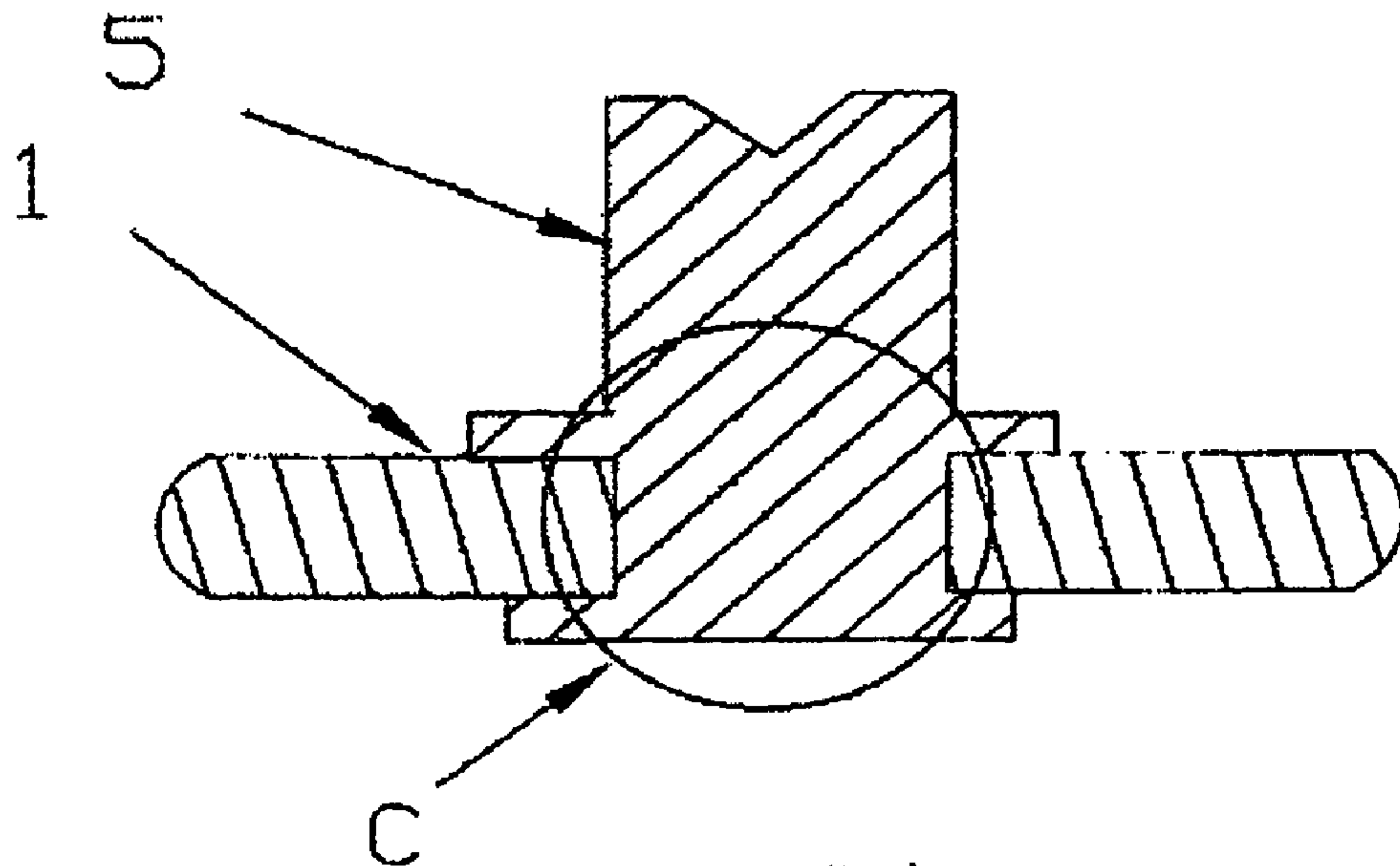
FIG. 4 (Prior art)
