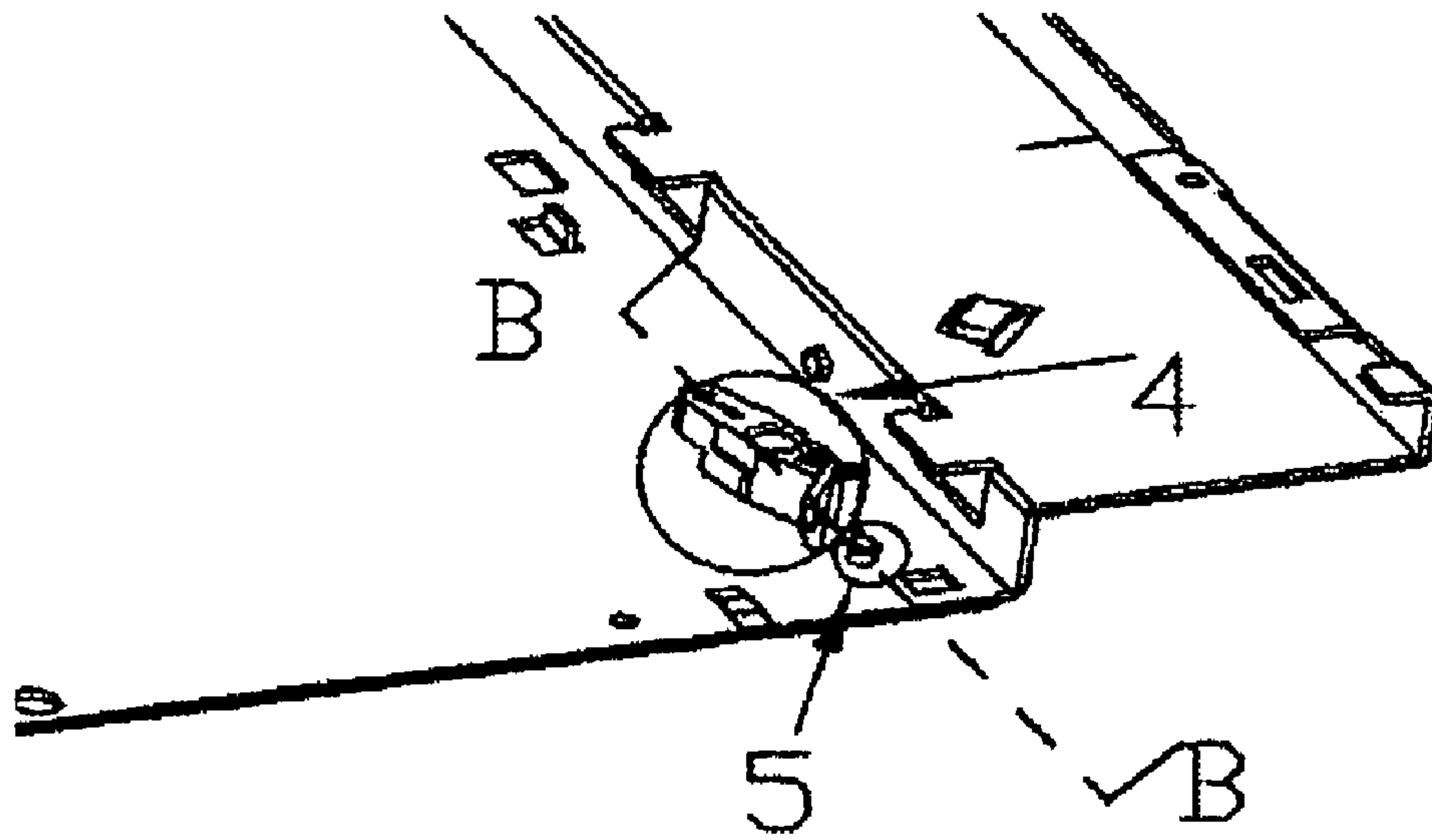
FIG. 3 (Prior Art)
