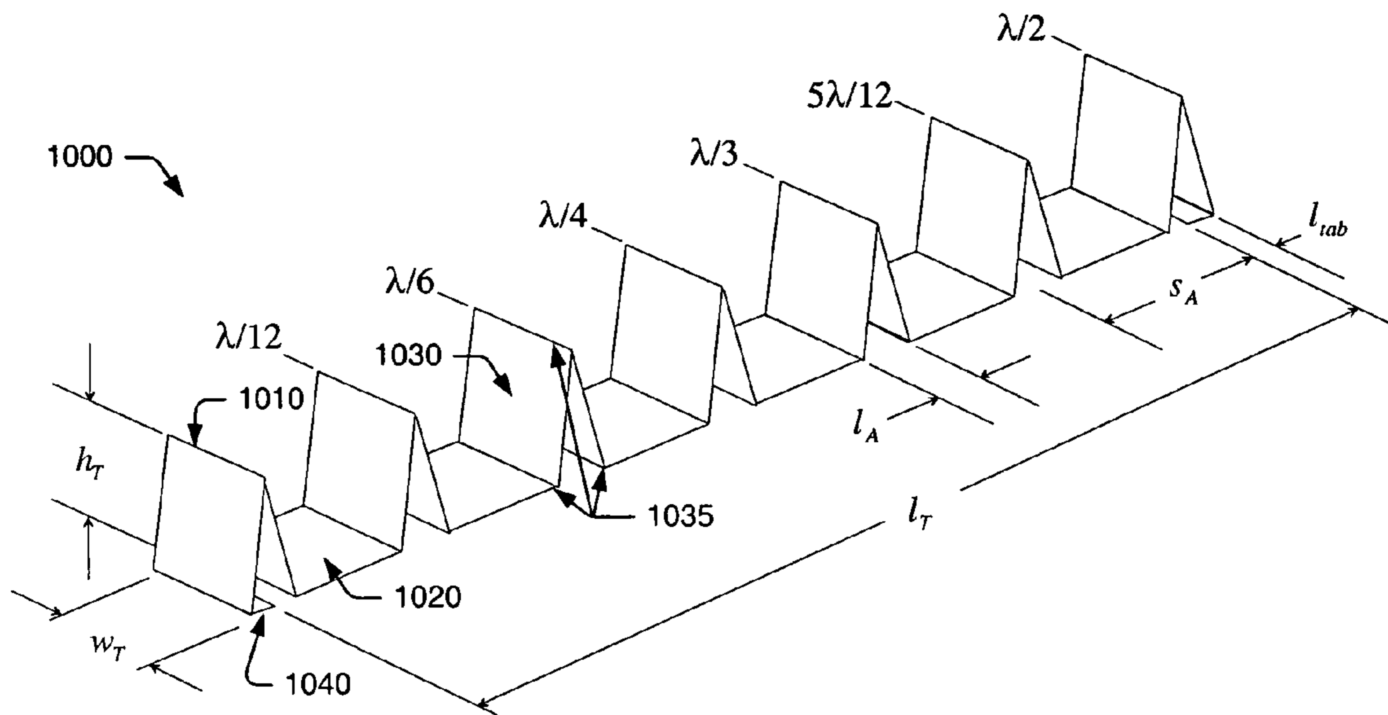
FIG. 10B FOLDED PATTERN
