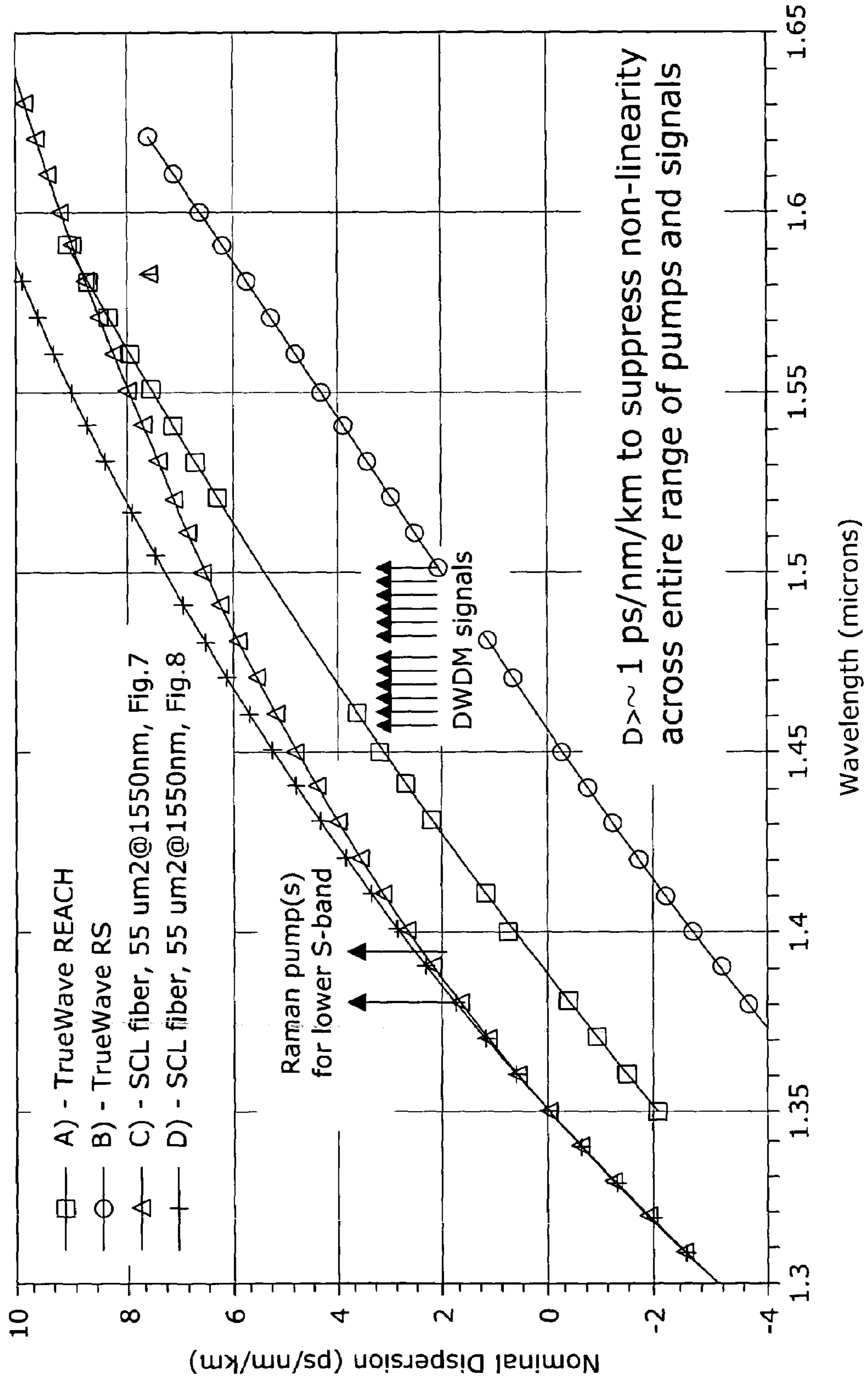
Fig. 2 Dispersion Curves for S-band Raman Pumping
