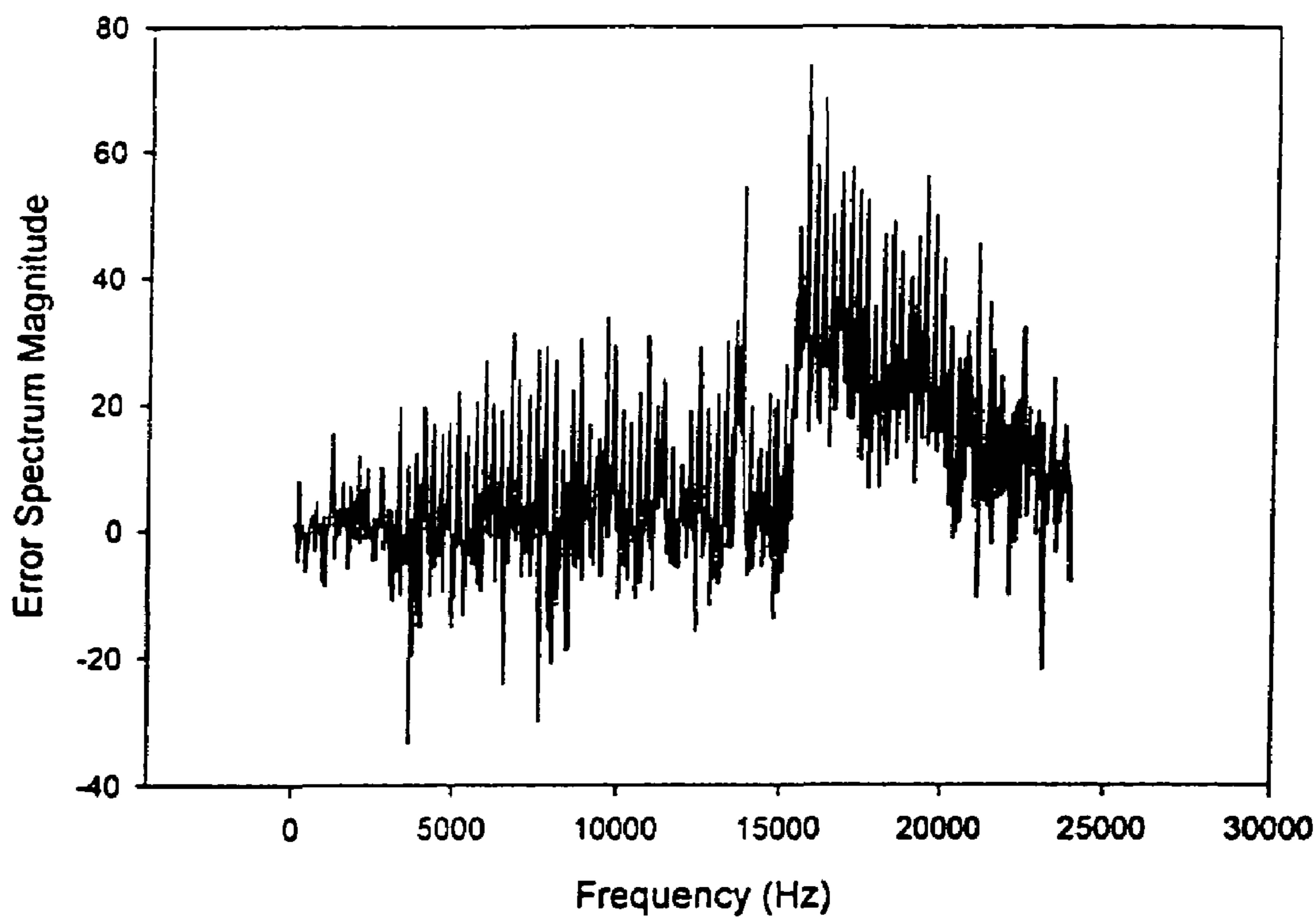
Figure 7. TestA error spectrum
