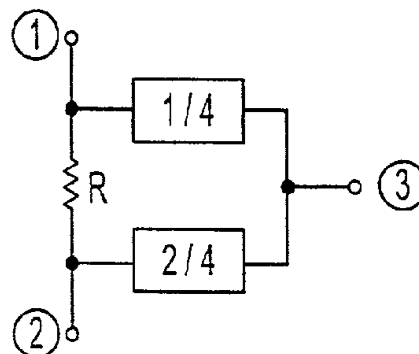
IN-PHASE SPLITTER-COMBINER
