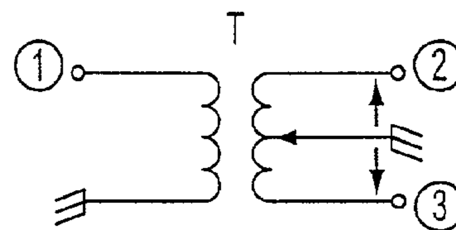
180° SPLITTER-COMBINER
