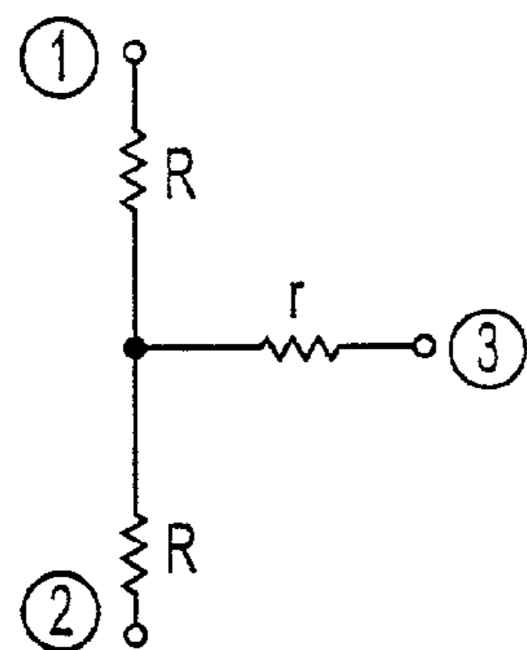
IN-PHASE SPLITTER-COMBINER
