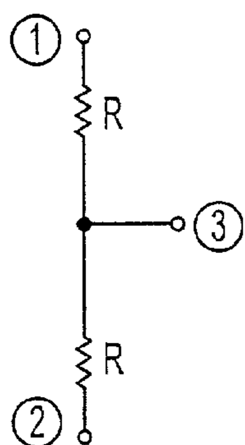
IN-PHASE SPLITTER-COMBINER
