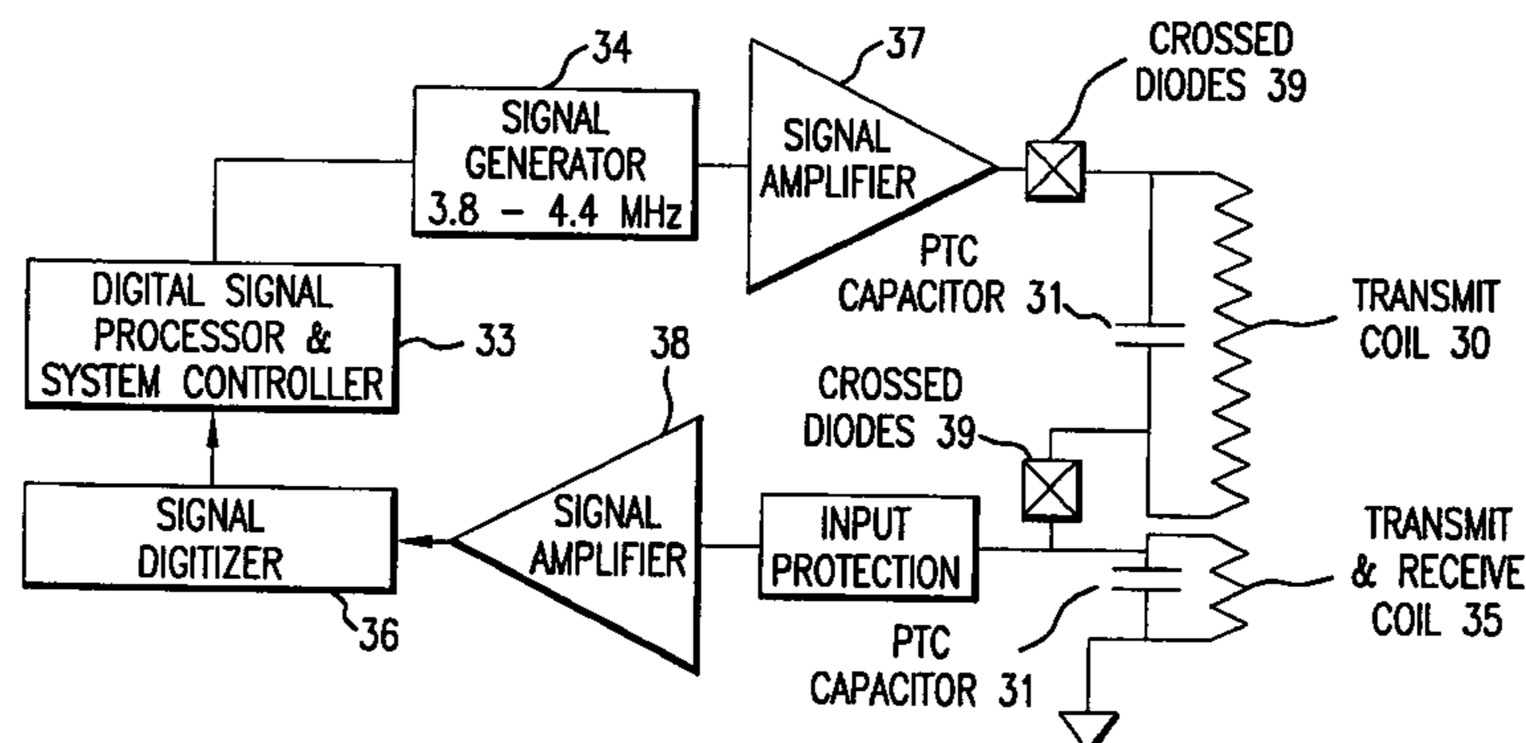
SYSTEM BLOCK DIAGRAM
