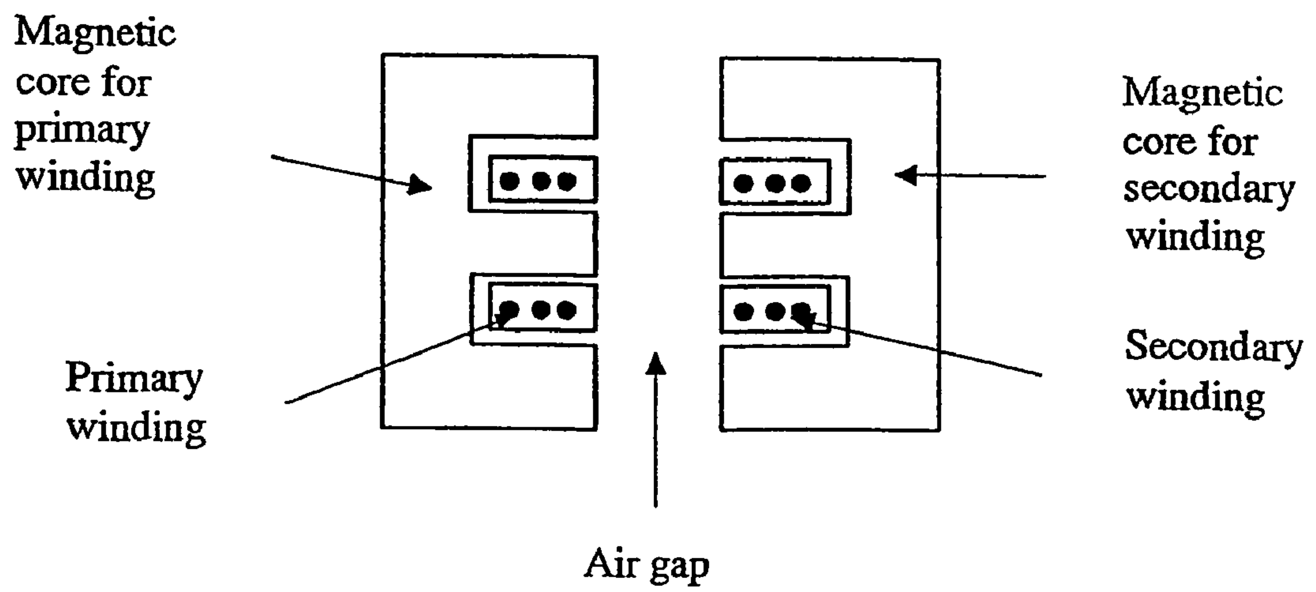
FIG. 2 (PRIOR ART)
