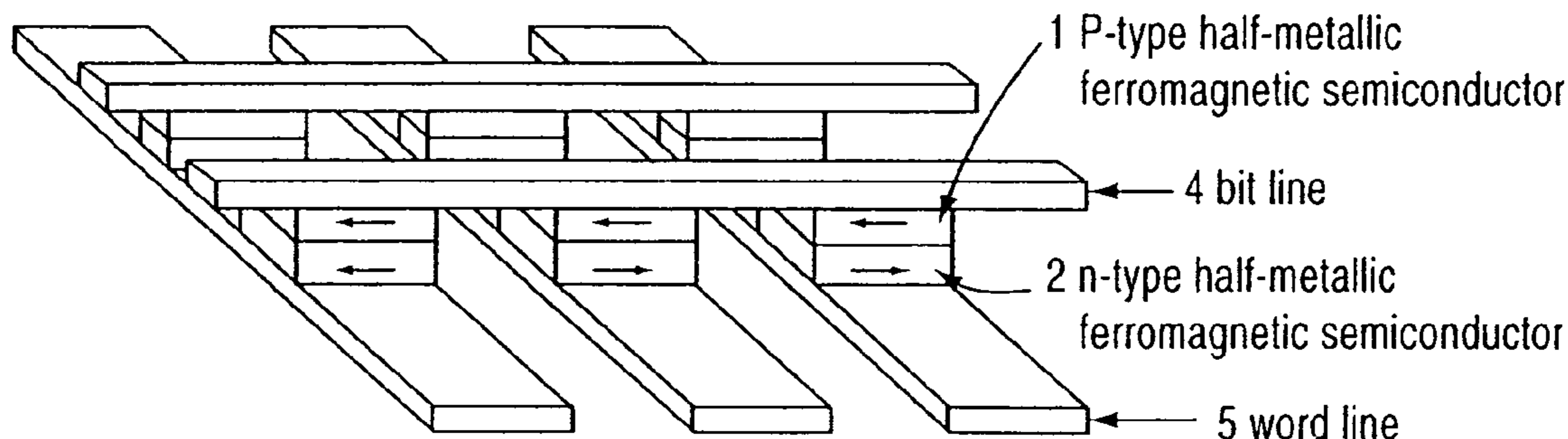
Ferromagnetic Tunneling Junction (P - n type)
