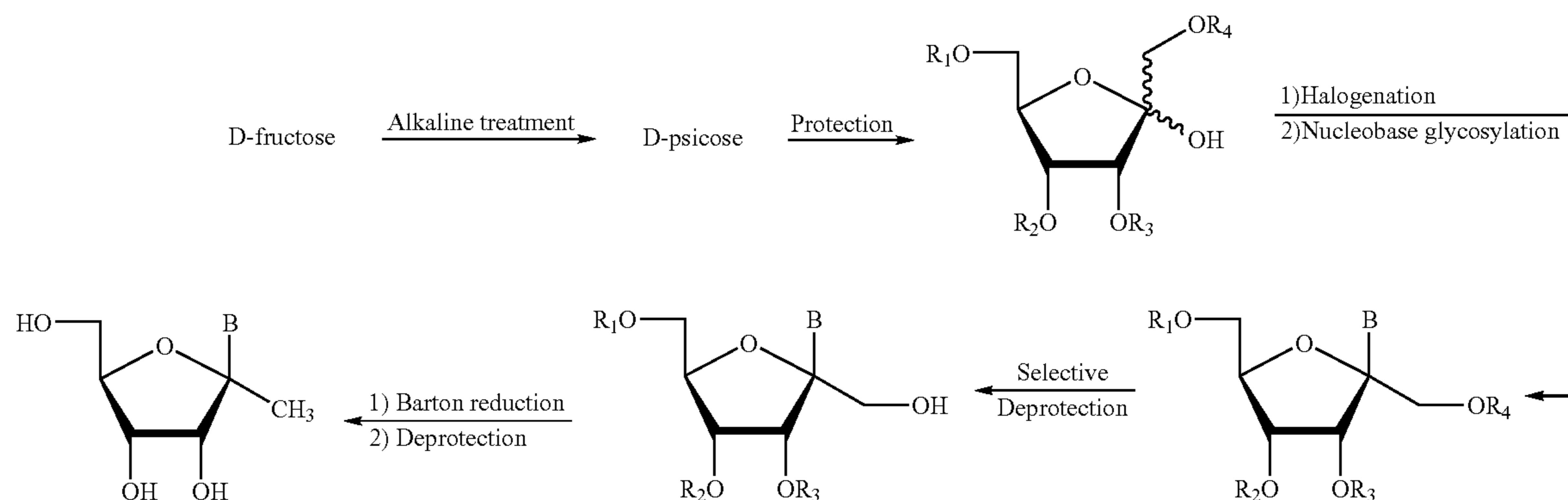
Scheme 2
