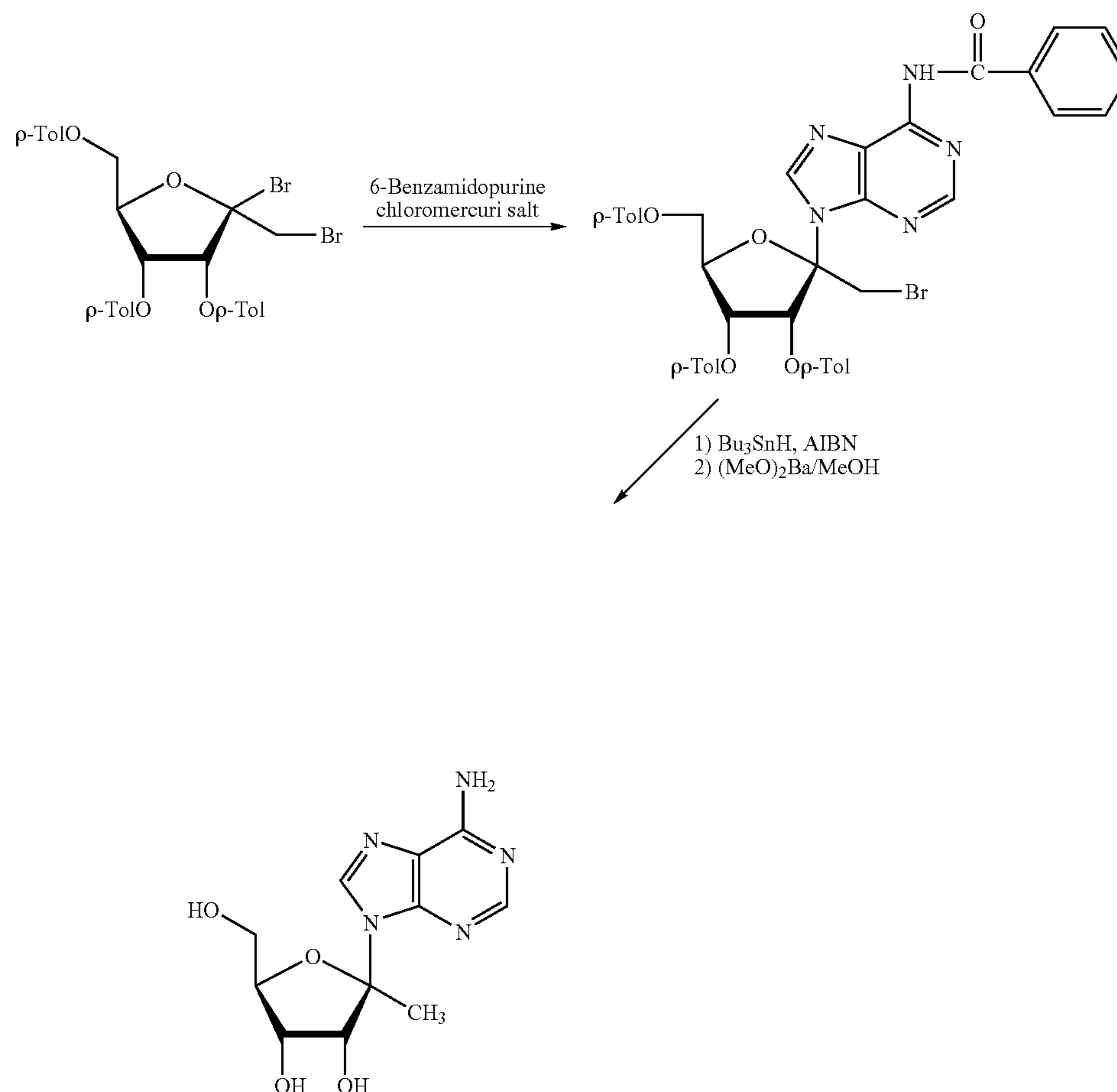
Scheme 7
