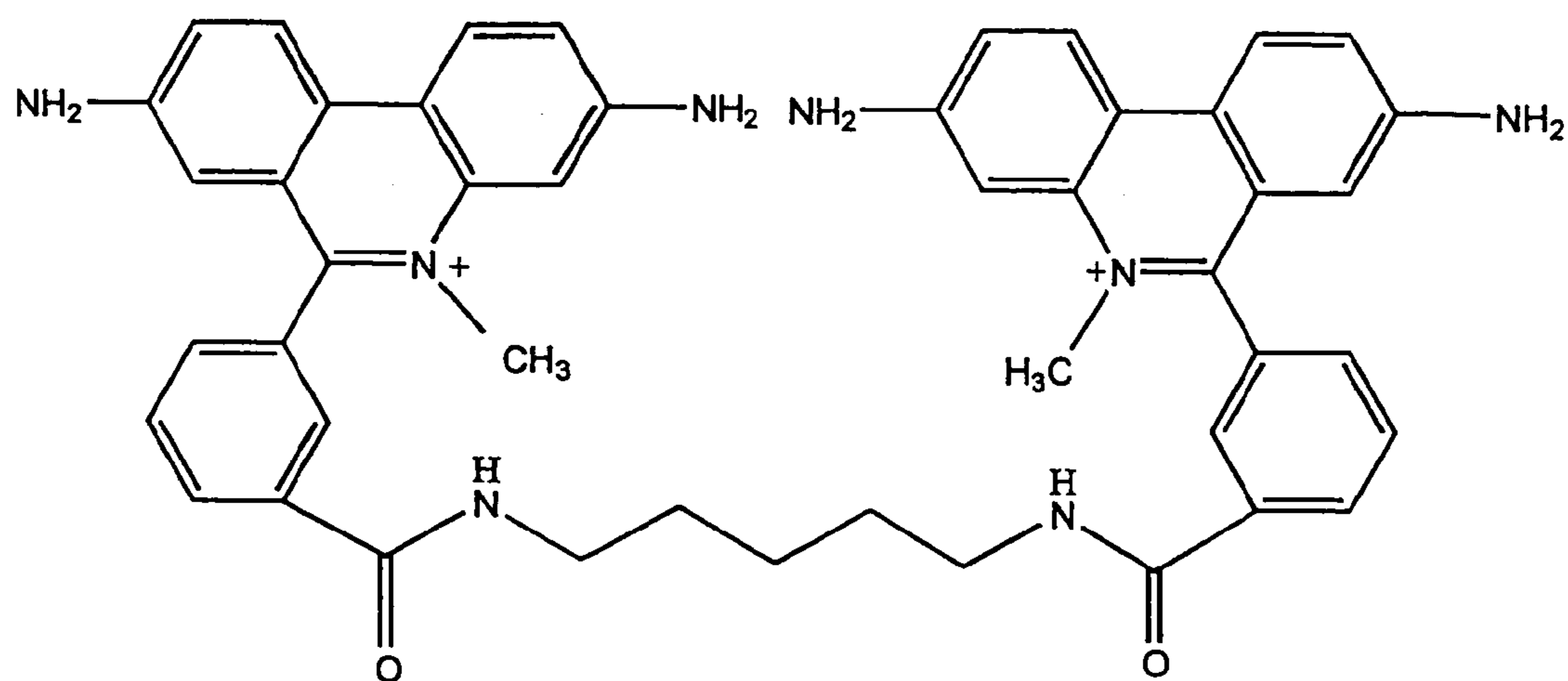
meta-EthD
