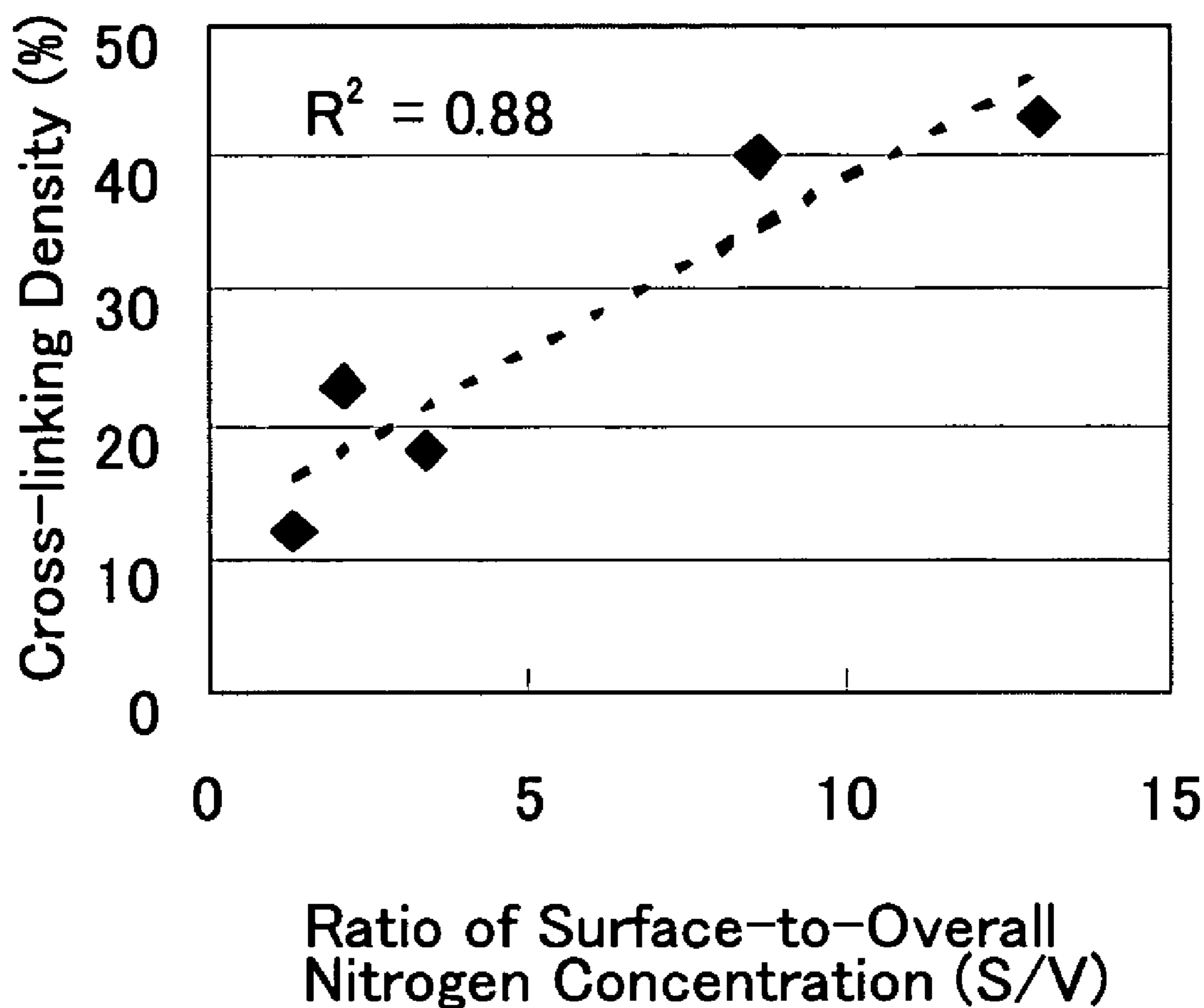
Relationship between Ratio of Surface-to-Overall Nitrogen Concentration and Cross-linking Density
