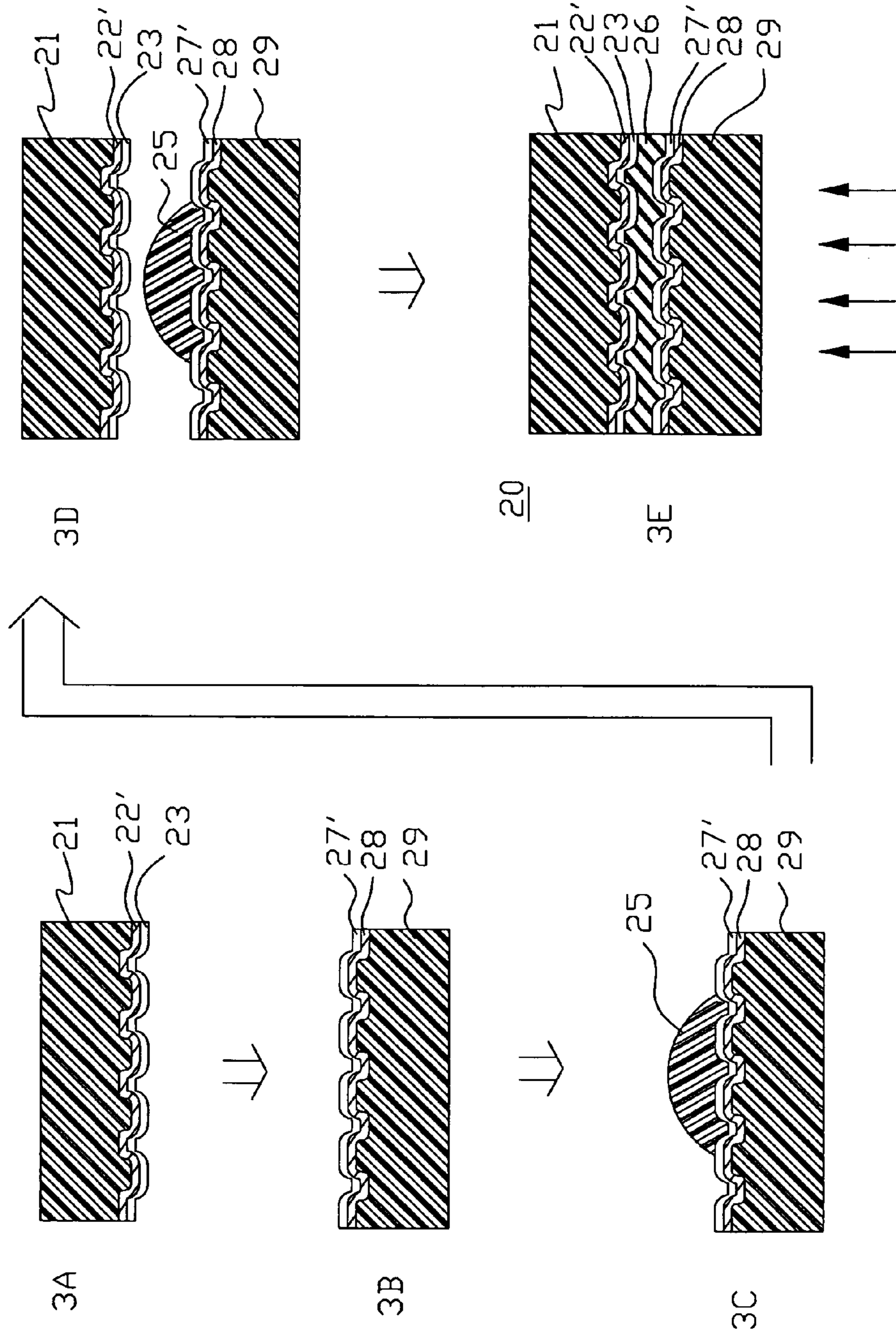
FIG. 3 PRIOR ART
