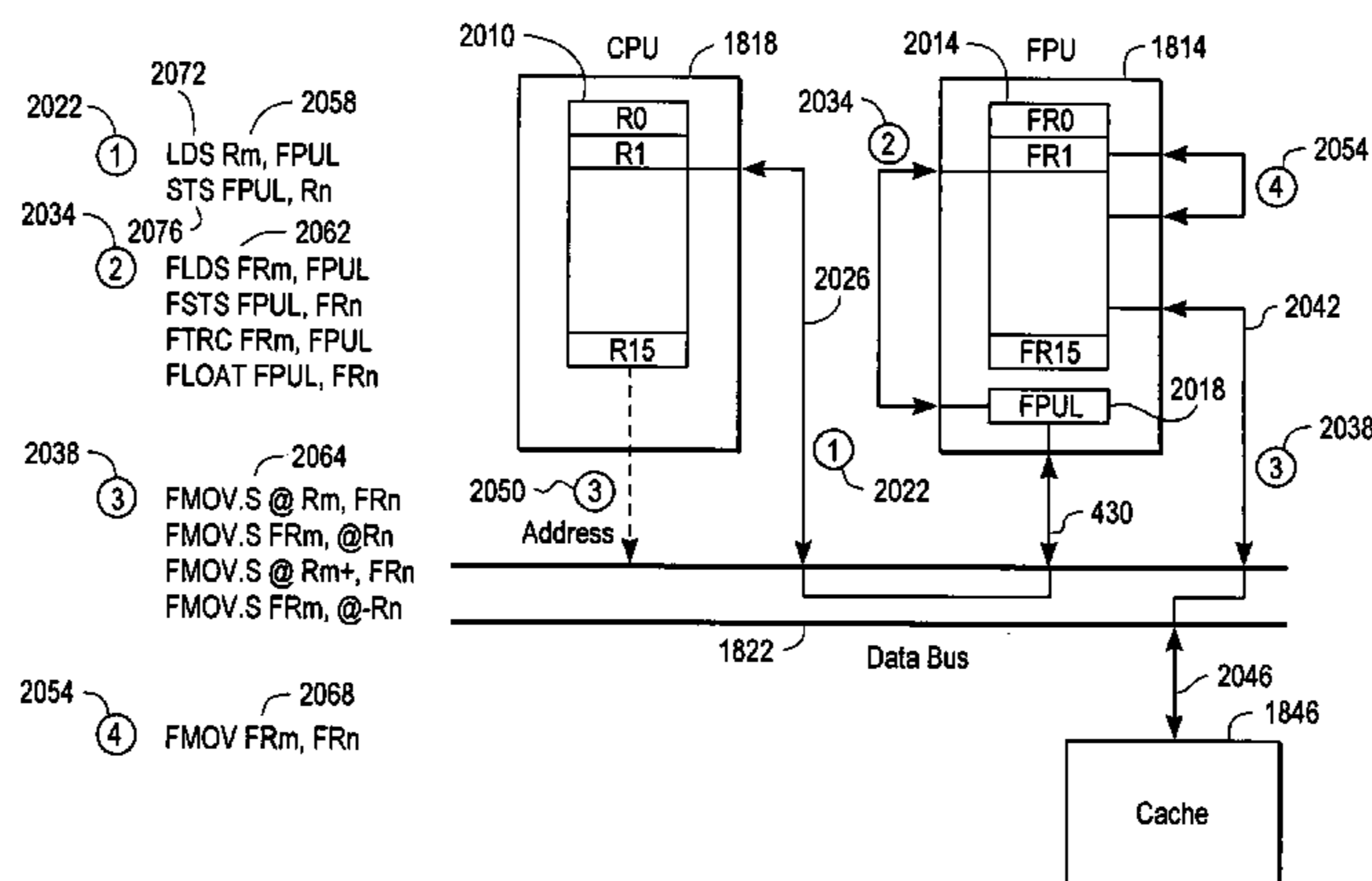
DATA MOVEMENT TO AND FROM FPU
