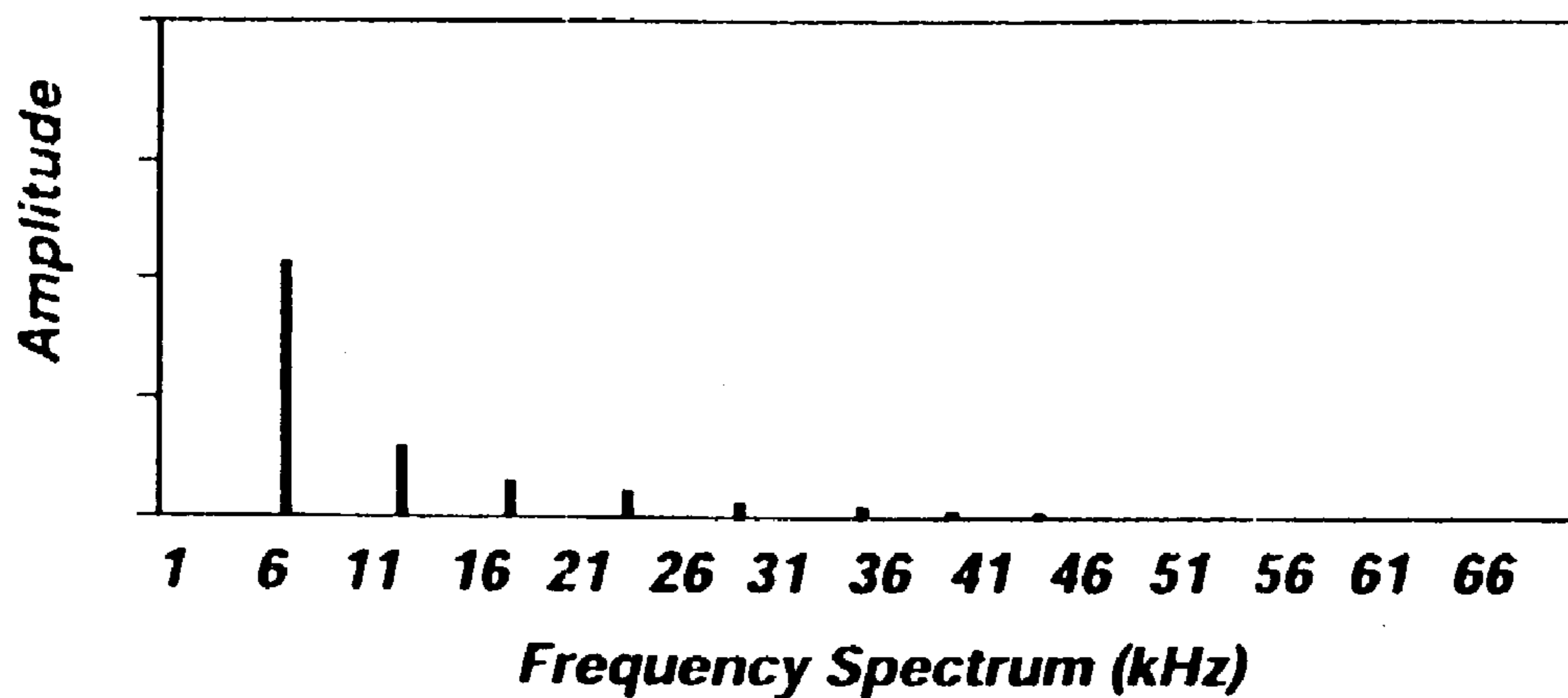
Fig. 3 (PRIOR ART)
