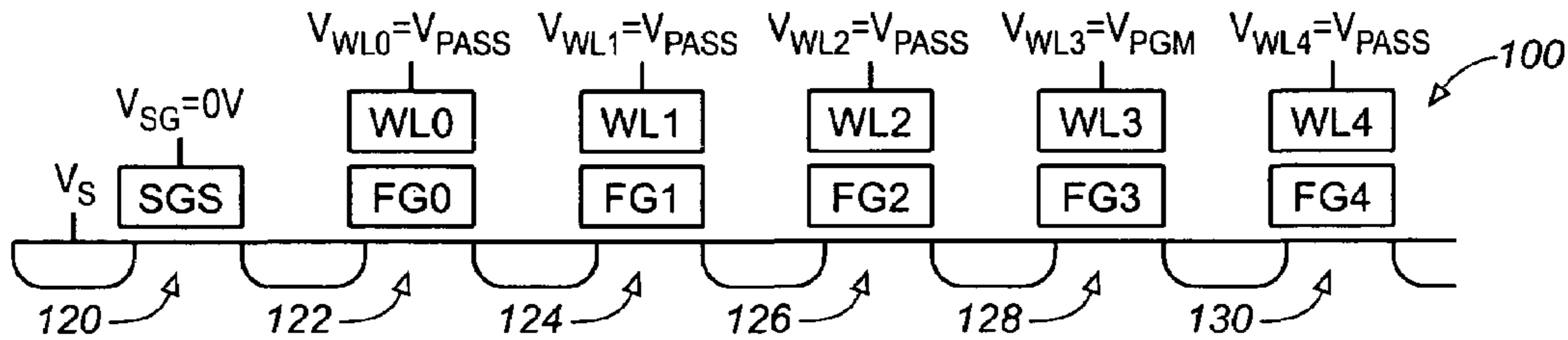
FIG. 4D (PRIOR ART)
