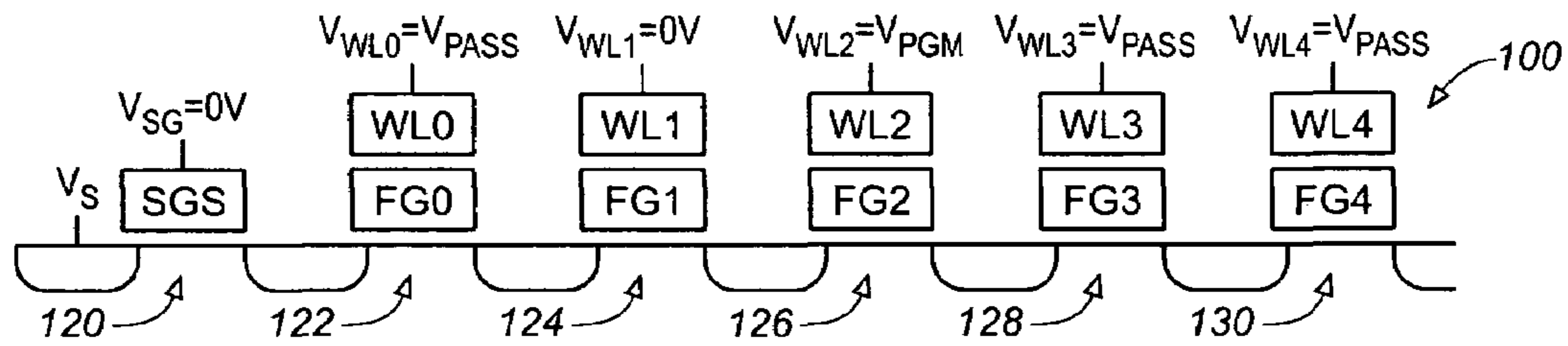
FIG. 6C (PRIOR ART)
