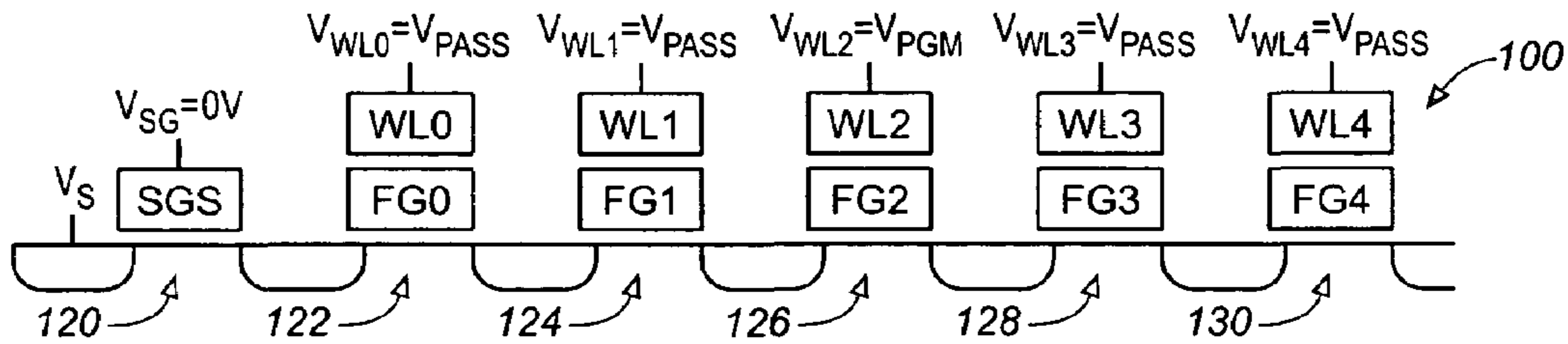
FIG. 4C (PRIOR ART)
