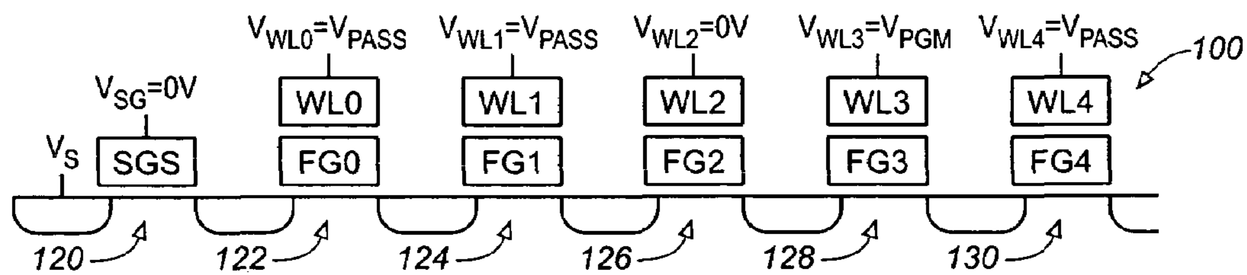
FIG. 6D (PRIOR ART)
