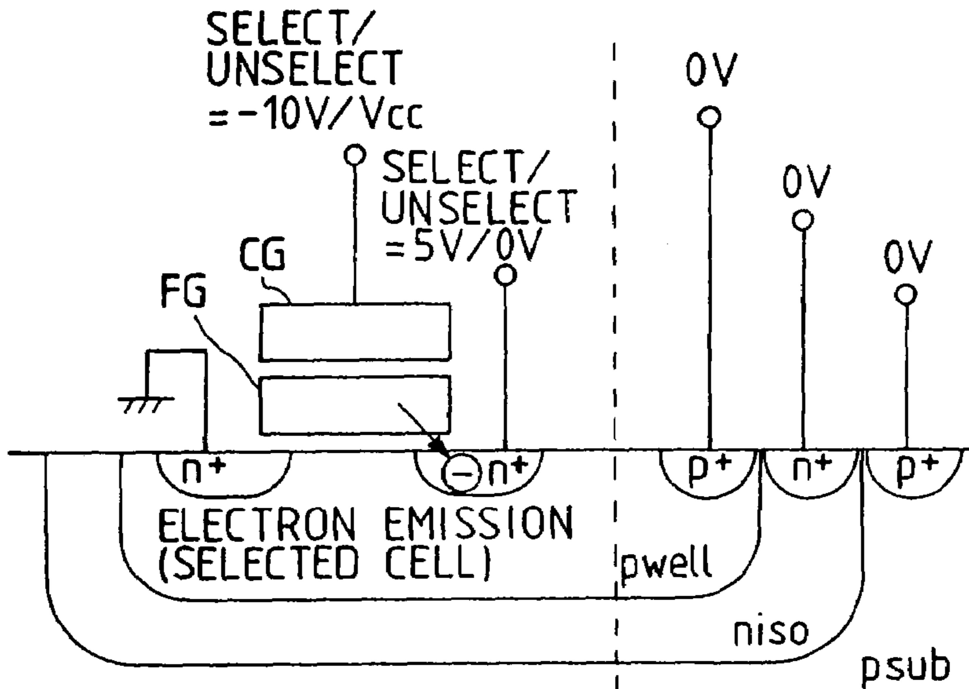
EXAMPLE OF APPLIED VOLTAGES AT PROGRAMMING TIME
