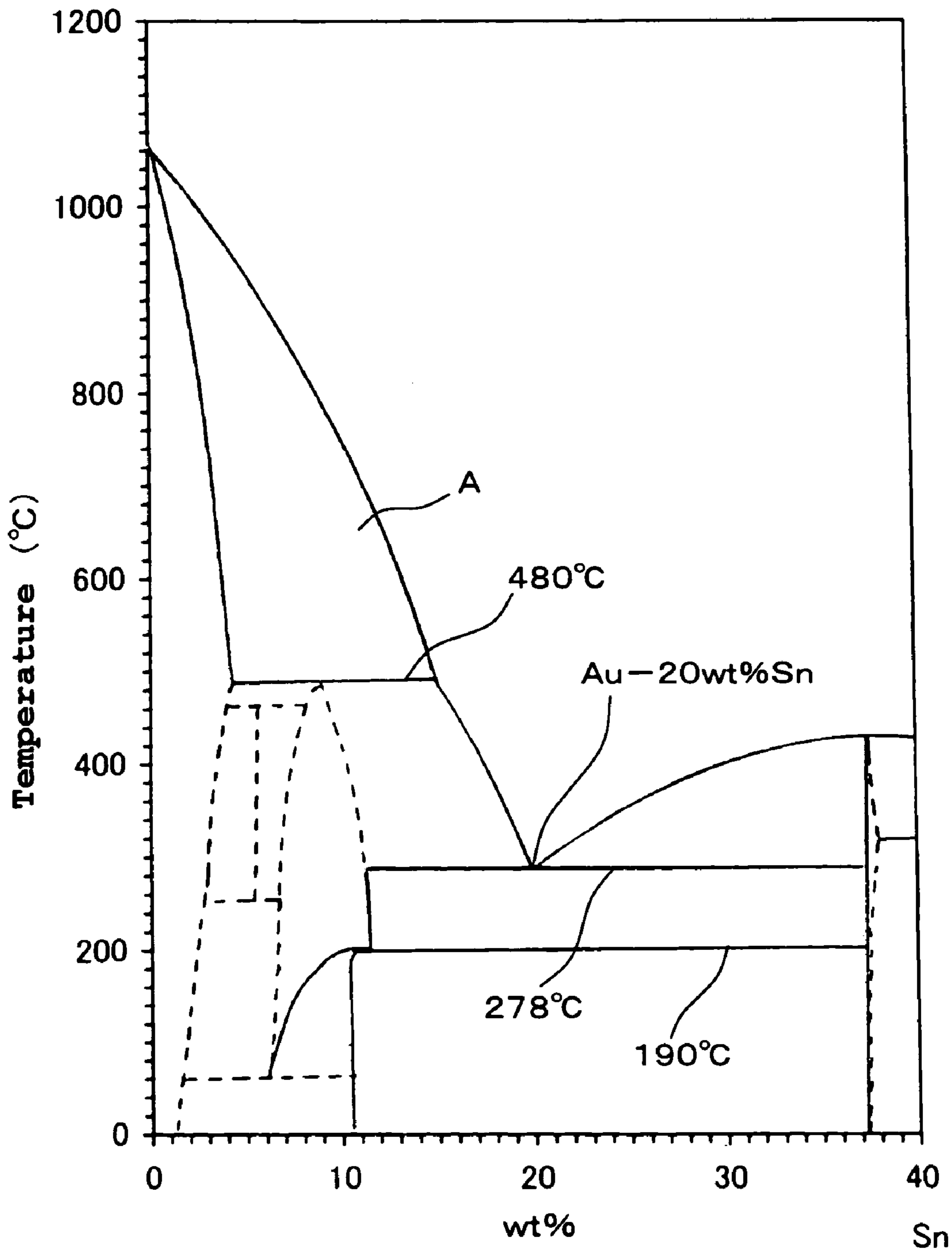
Au-Sn series equilibrium diagram
