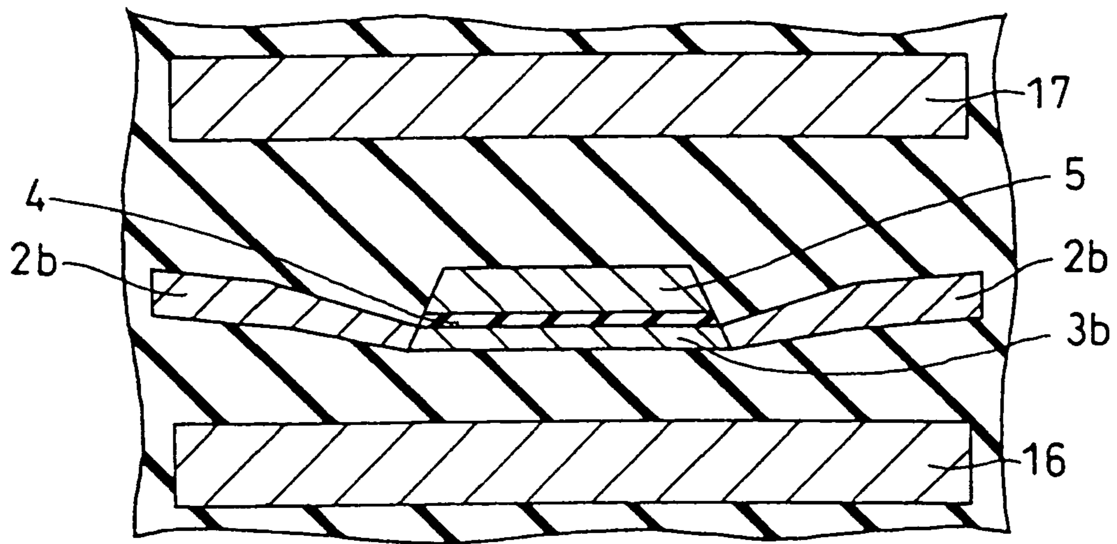
FIG. 3 (PRIOR ART)
