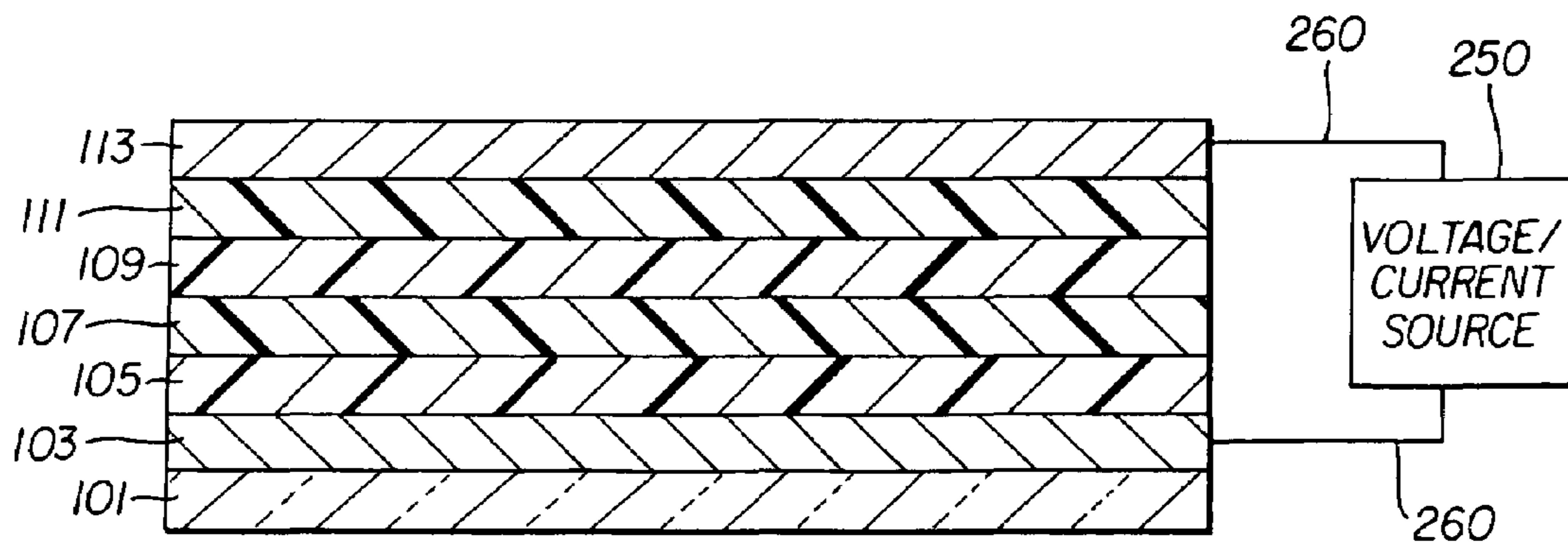
FIG. 4 (Prior Art)
