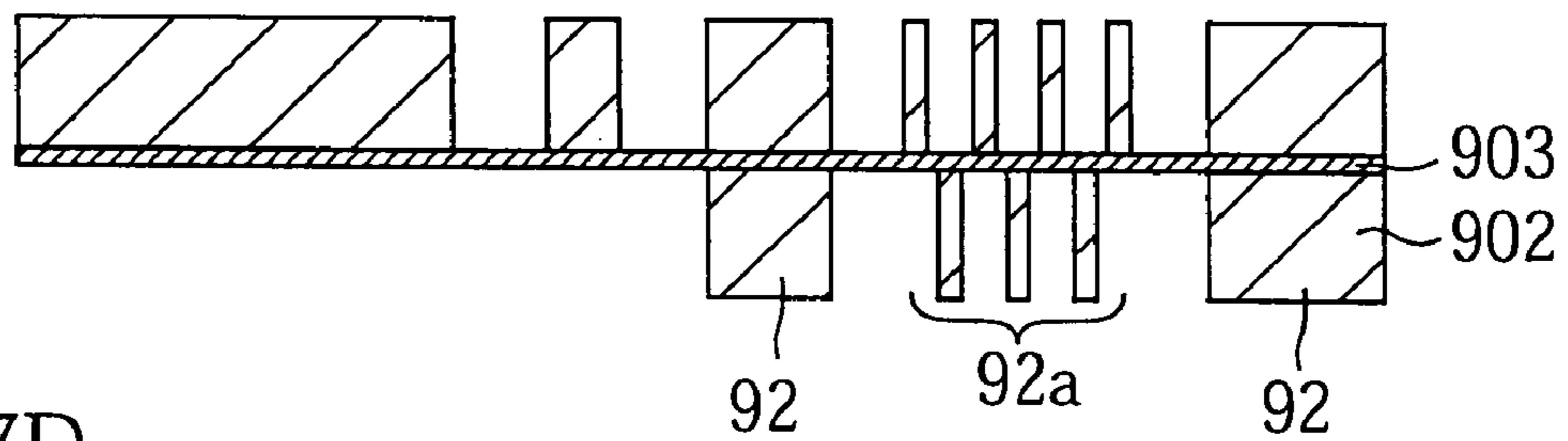
FIG. 47C PRIOR ART
