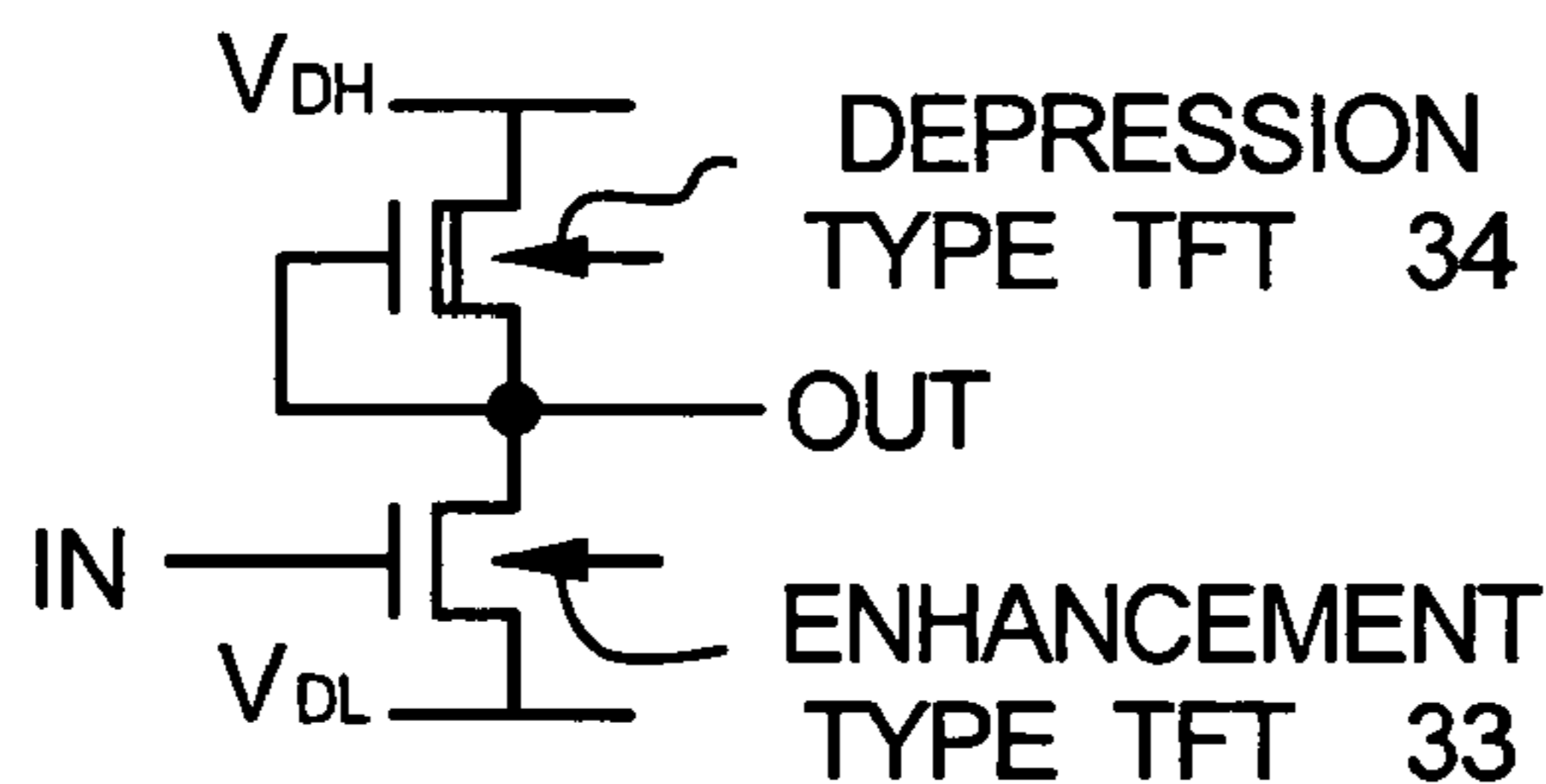
FIG. 8B EDMOS CIRCUIT
