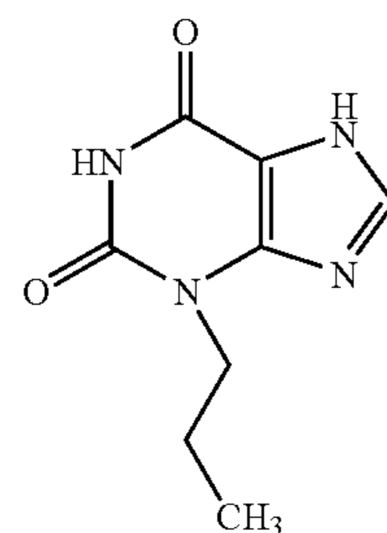
3-n-Propylxanthine
