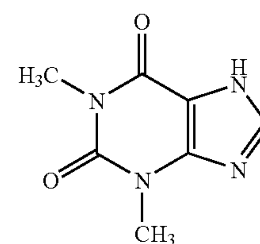
Theophylline
