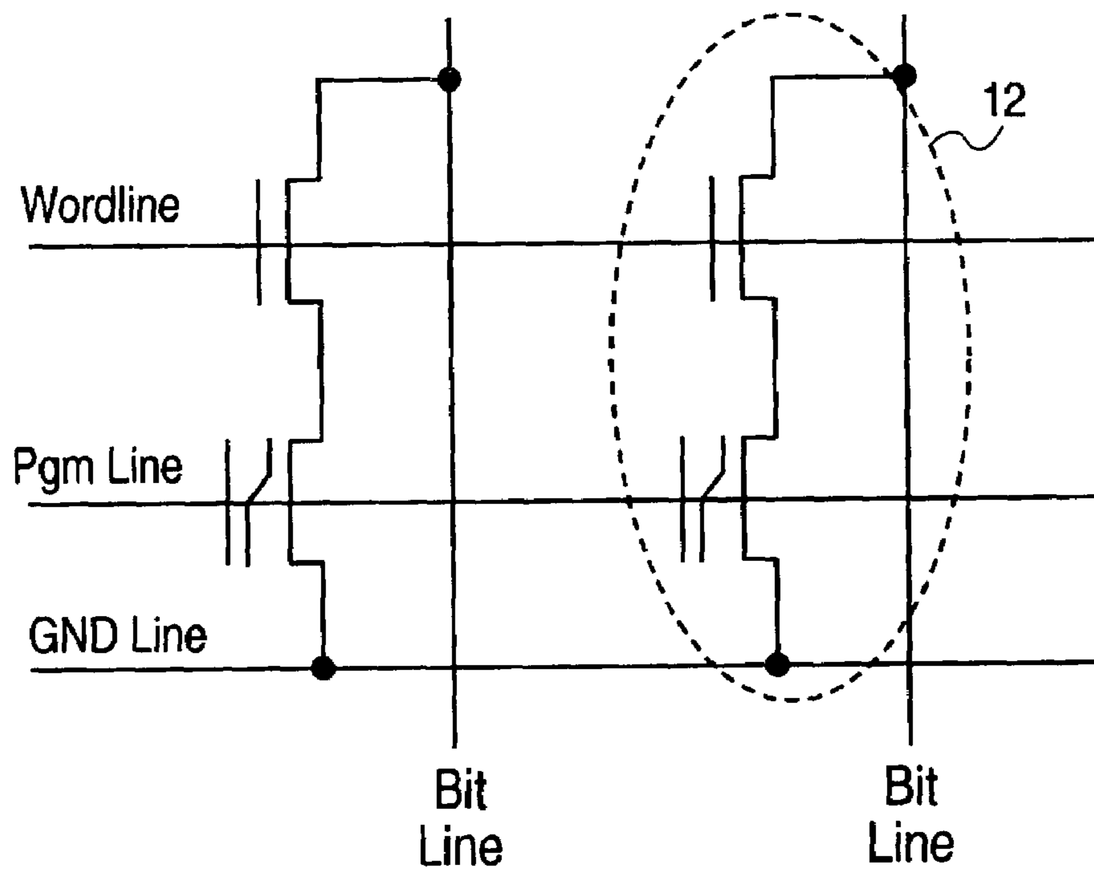
FIG. 2 (PRIOR ART)
