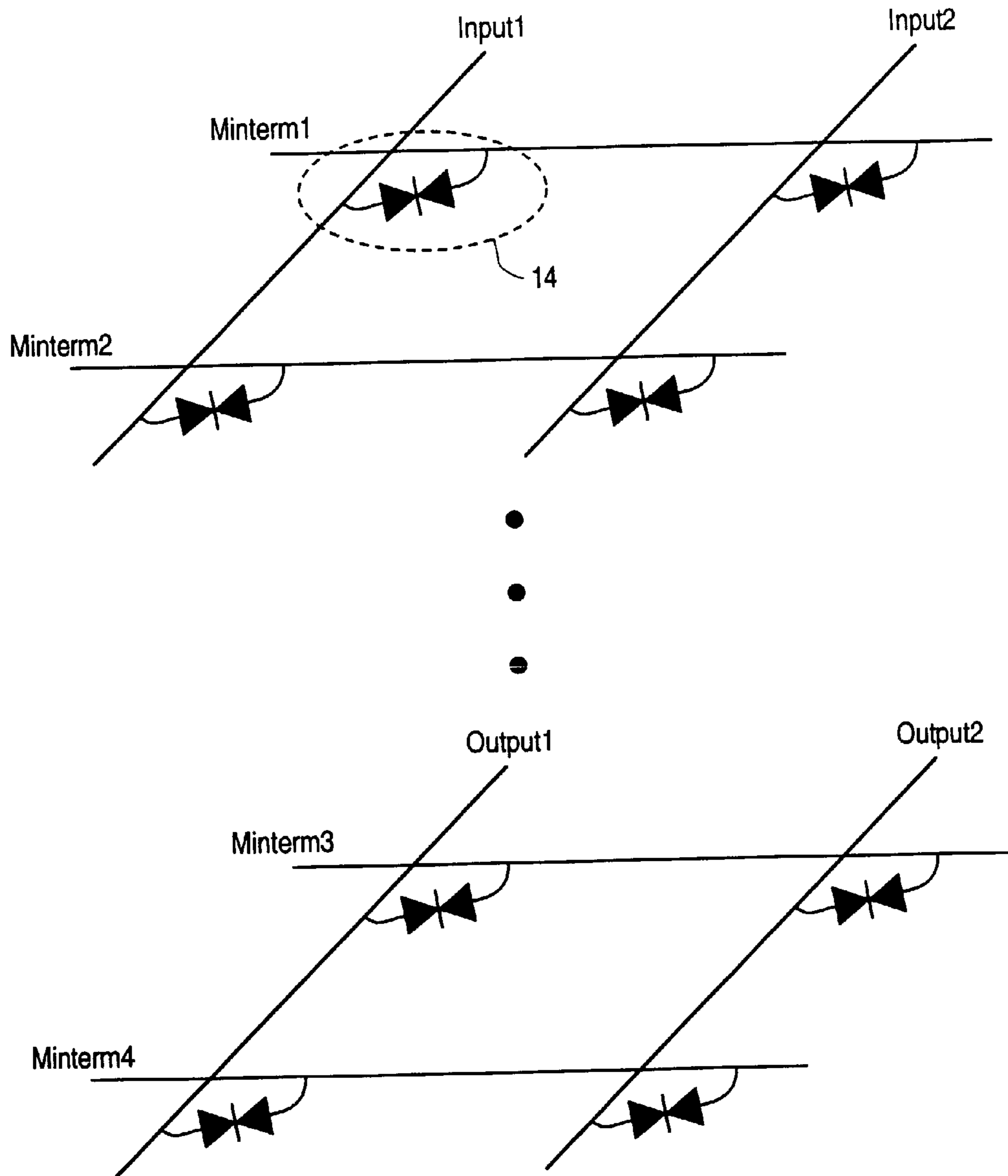
FIG. 3 (PRIOR ART)
