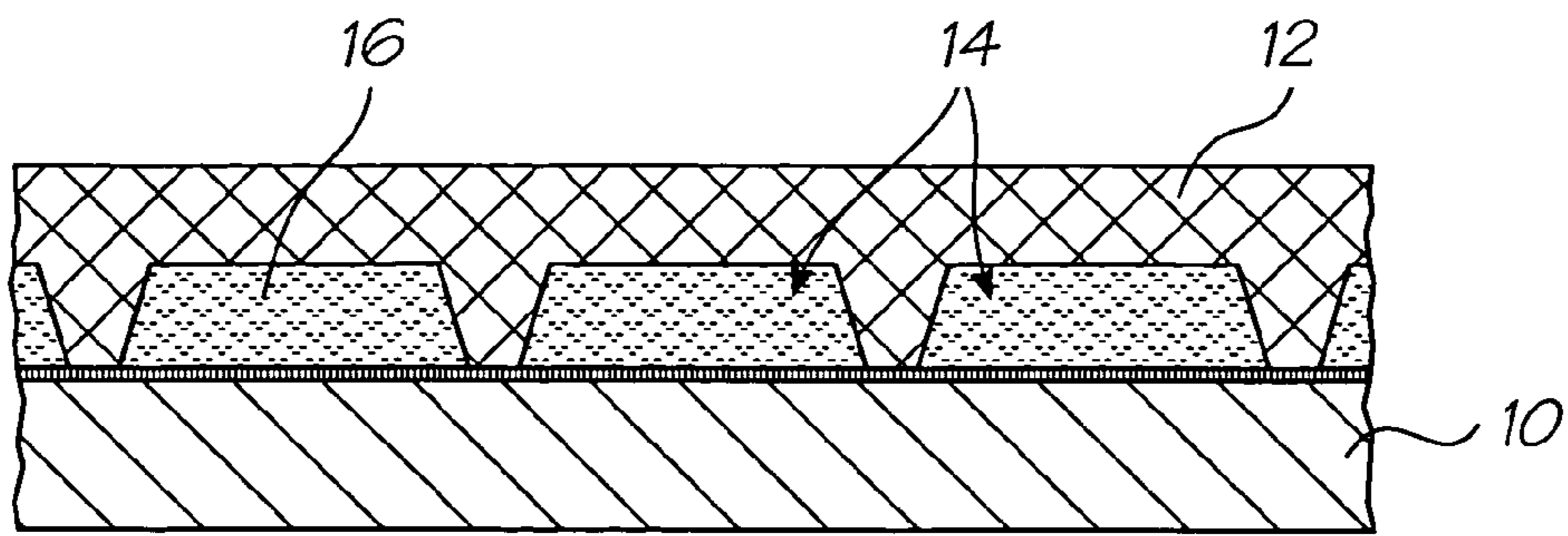
FIG. 1 (Prior Art)
