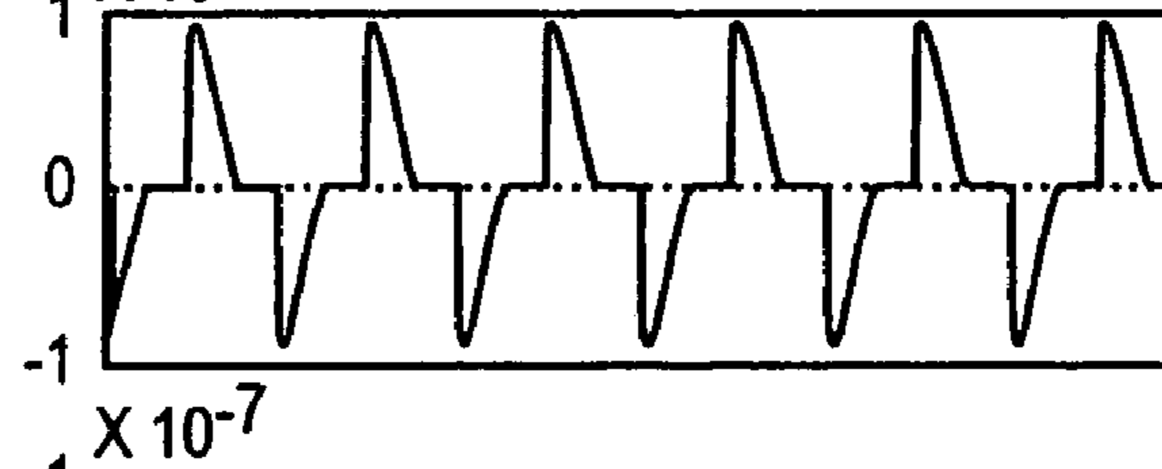
FIG. 18B TRANSDUCER CURRENT
