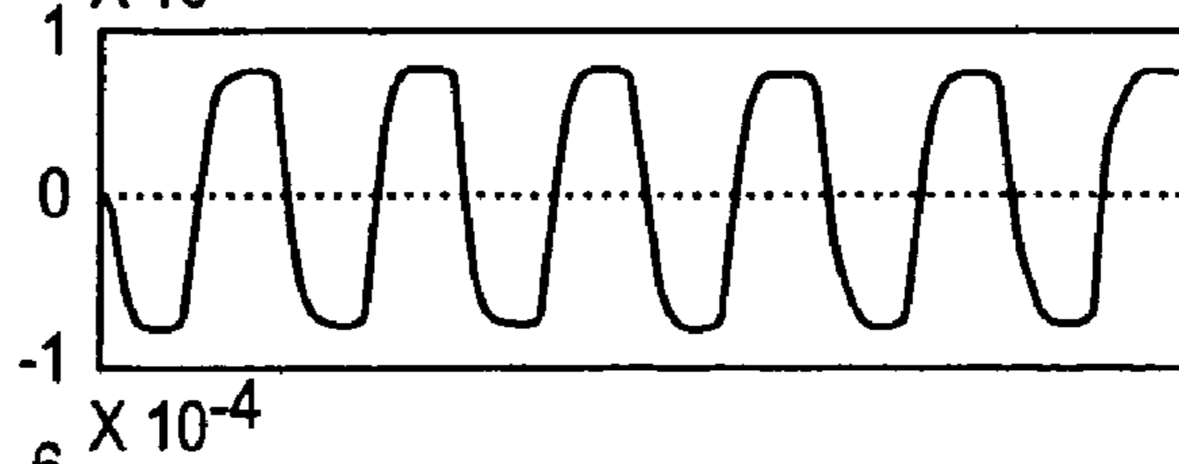
FIG. 18C Q_{\text{TRANSDUCER}}(C)
