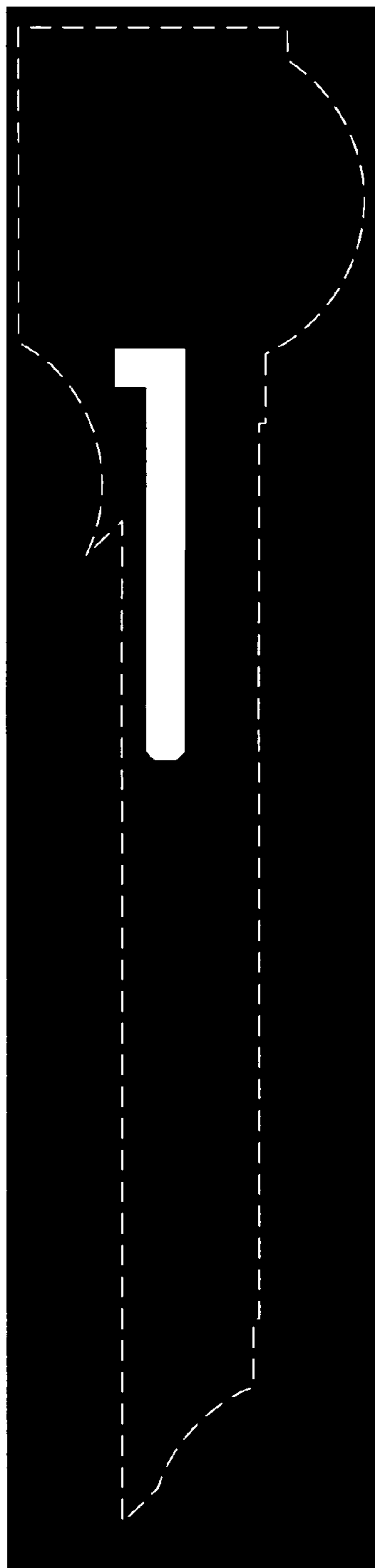
N-Well mask
