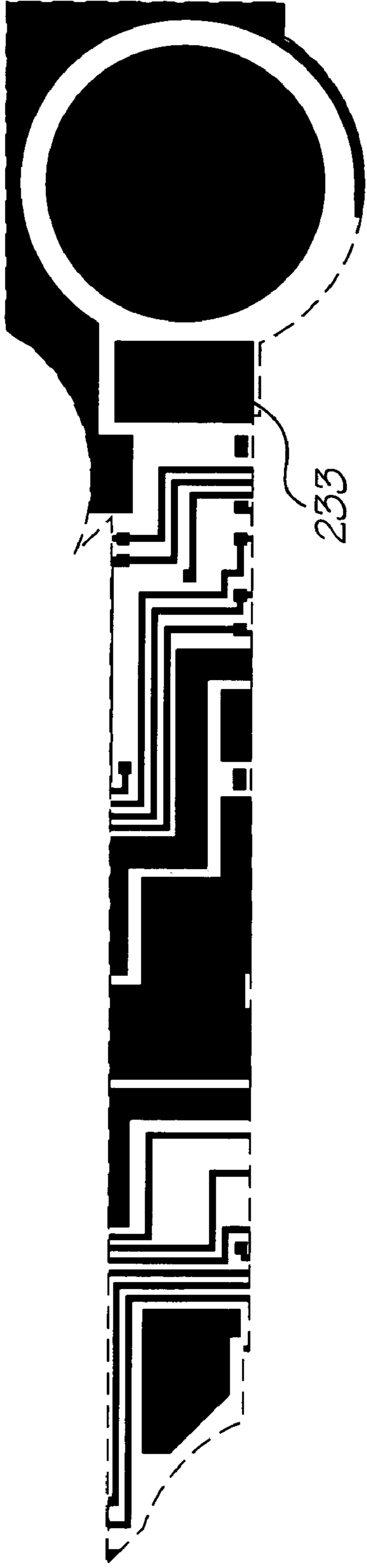
Metal 2 mask
